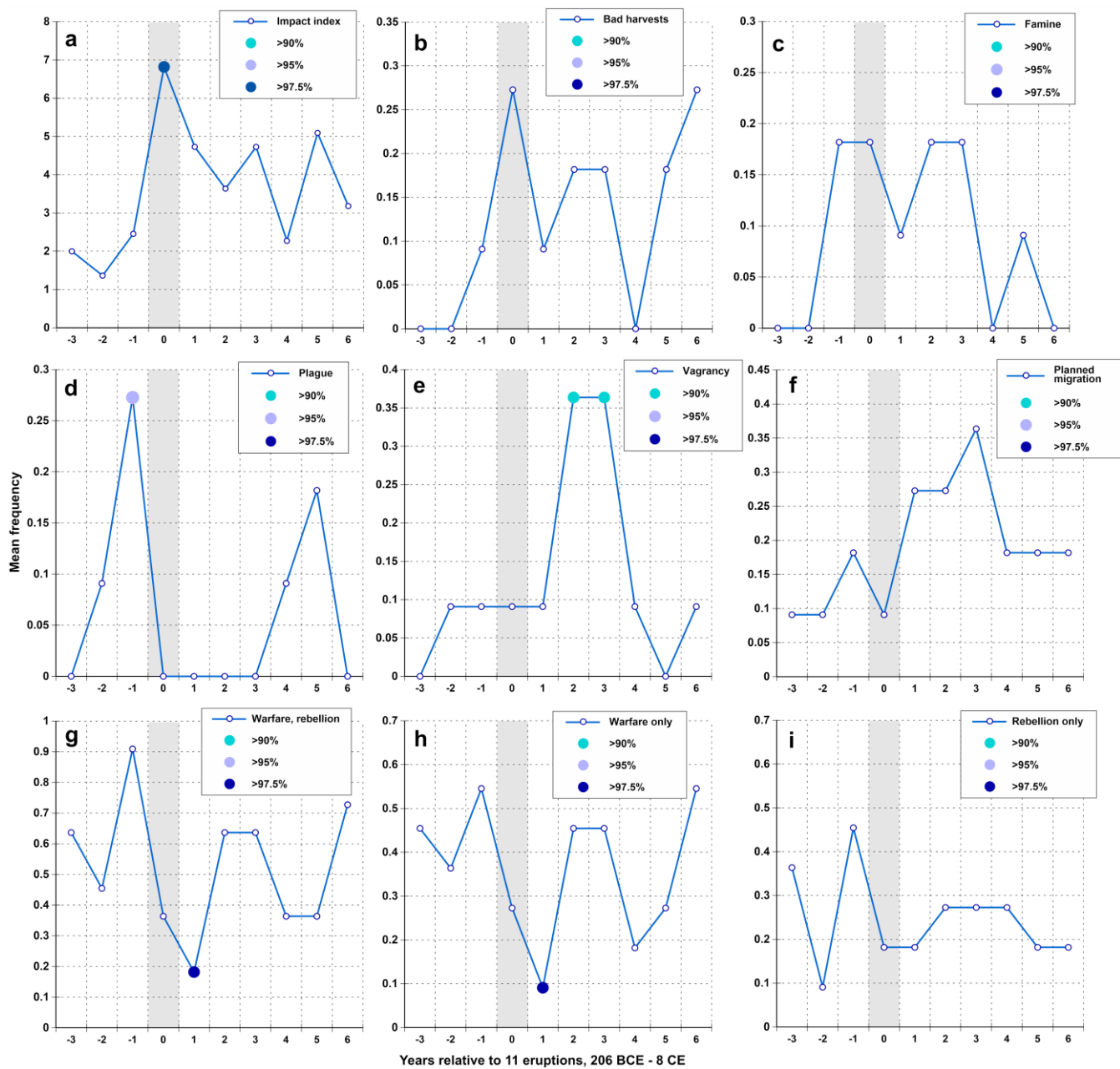
Figure 65. Superposed Epoch Analysis (SEA) results showing the compositing of each time series of societal stress proxies relative in time to the dates of 11 presumed-tropical and extratropical NH volcanic eruptions (identified based on ice-core evidence (Sigl et al., 2015)) that are taken as focal event years and represented at point 0 on the horizontal axes. Colour coded dots identify years deemed statistically significant at (at least) 90% confidence (one-tailed).
