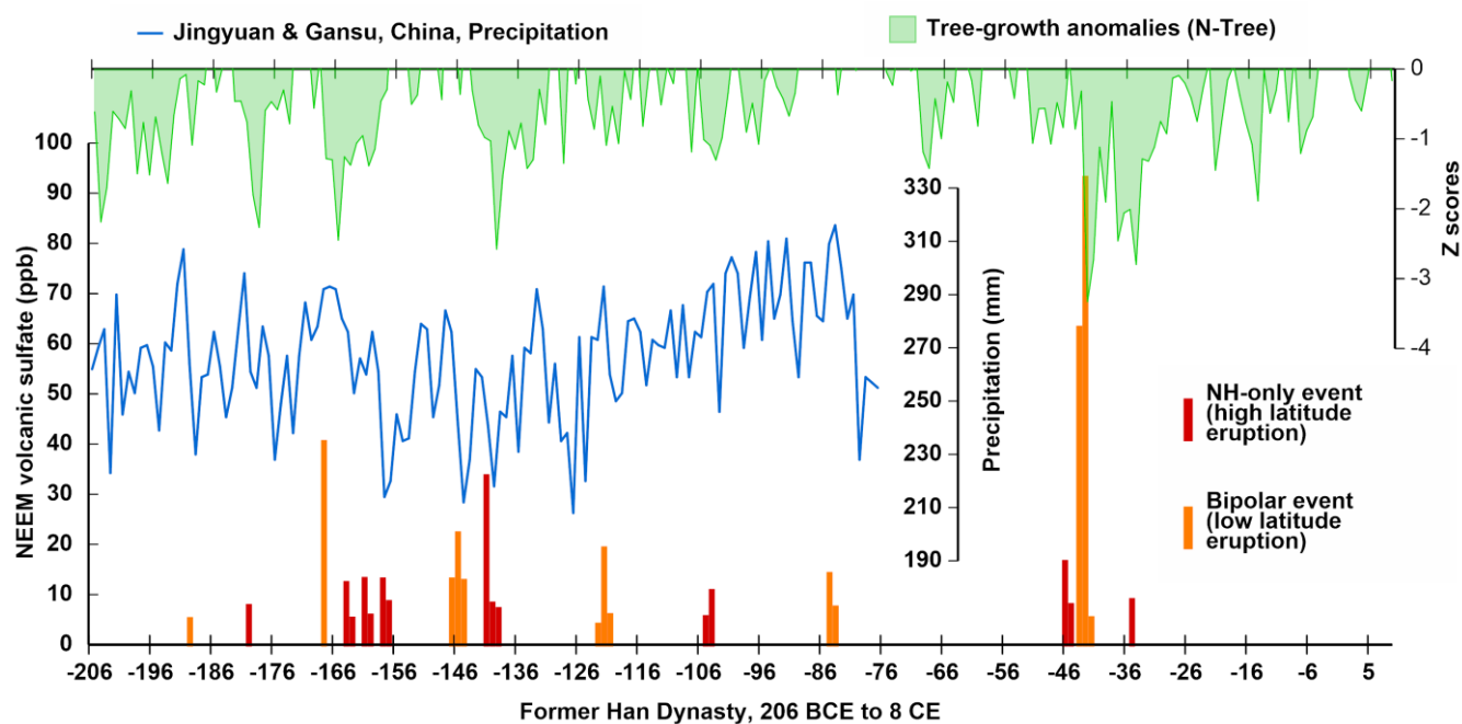
Figure 3-2: Indicative climate forcing potential as represented by the (non-sea-salt) volcanic sulphate volume measured in parts per billion (ppb) in the annual layers of the NEEM Greenland ice-core for the fourteen inferred tropical and NH extratropical eruptions identified during the Western Han period (Sigl et al., 2015). Higher volumes imply greater climate forcing potential. These deposition volumes can be converted into time-integrated global radiative forcing estimates of the reduction in solar energy received at the Earth’s surface in watts per square meter arising from the atmospheric loading of volcanic sulphate aerosols. For each eruption, these are 190 BCE (1.69 w/m 2 reduction), 180 (0.64), 168 (7.90) 164 (1.31), 161 (1.46), 158 (1.51), 147 (7.50), 141 (3.29), 123 (6.56), 105 (1.27), 85 (4.15), 46 (2.07), 43 (23.21) and 35 BCE (0.74). For context, the temperature sensitive NH N-Tree tree ring chronology is also shown (plotting negative growth anomalies relative to the 1000-1099 CE mean; Sigl et al., 2015), as is the Qin et al. (2025) tree-ring-based precipitation reconstruction for Jingyuan and Gansu, China.
