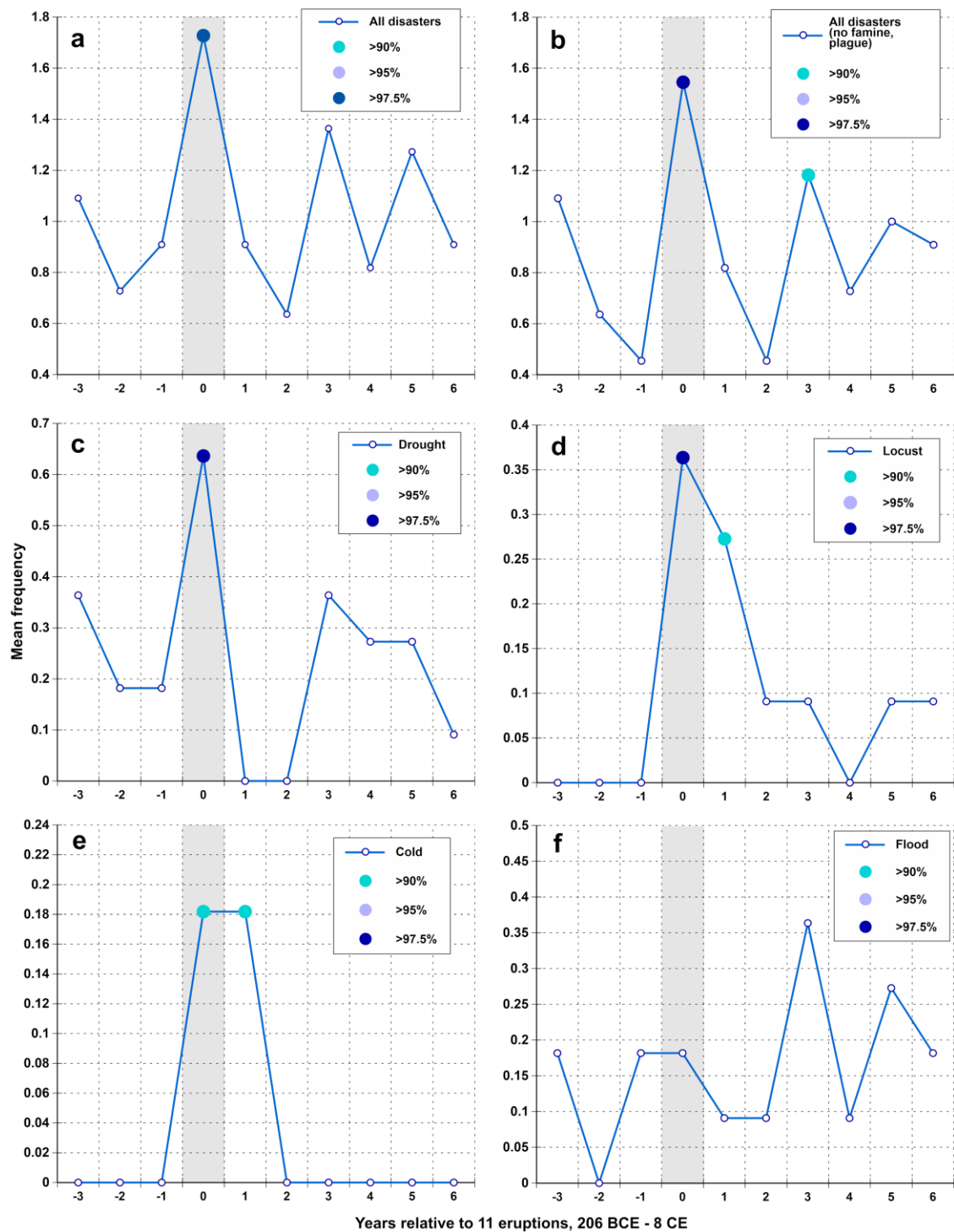
Figure 54. Superposed Epoch Analysis (SEA) results of the time series of climate and climate-related disasters relative in timing to 11 presumed-tropical and Northern Hemisphere (NH) extratropical volcanic eruptions (identified based on ice-core evidence (Sigl et al., 2015)) as focal event years (represented at year zero on the horizontal axes). Colour coded dots identify years deemed statistically significantly elevated at (at least) 90% confidence.
