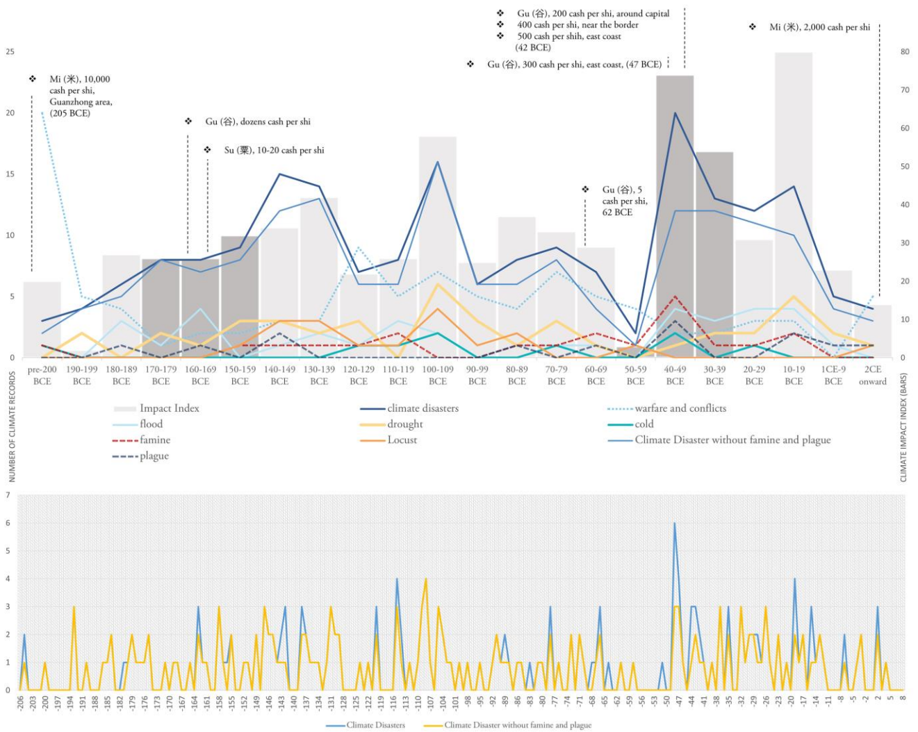
Figure 43. The top panel shows the time-series of various proxies of climatic and societal stresses in the Western Han dynasty at a decadal resolution. The bottom panel presents the time-series of the number of climate disasters, both including and excluding instances of famine and plague, at an annual resolution. Shi (top panel) is a unit of measurement, and it is approximately 30 kg today. Gu (谷) here refers to grain in general. Mi (米) is understood as rice or hulled millet, and Su (粟) refers to spiked millet (Dubs, 1938; Swann, 2013; Hsu, 1980).
