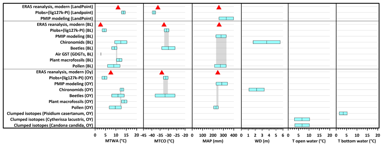
Figure 12. Boxplot of proxy-reconstructed and modeled climate and environmental data according to Table 7. BL – Bol’shoi Lyakhovskiy, Oy – Oyogos Yar, MTWA - mean temperature of the warmest month, MTCO – mean temperature of the coldest month, WD – water depth of thermokarst lakes, T open water – surface water temperature of lakes, T bottom water – bottom water temperature of lakes. Grey-shaded areas indicate ranges of overlap among paleoclimate indicators ; red triangles indicate the present-day reference.
