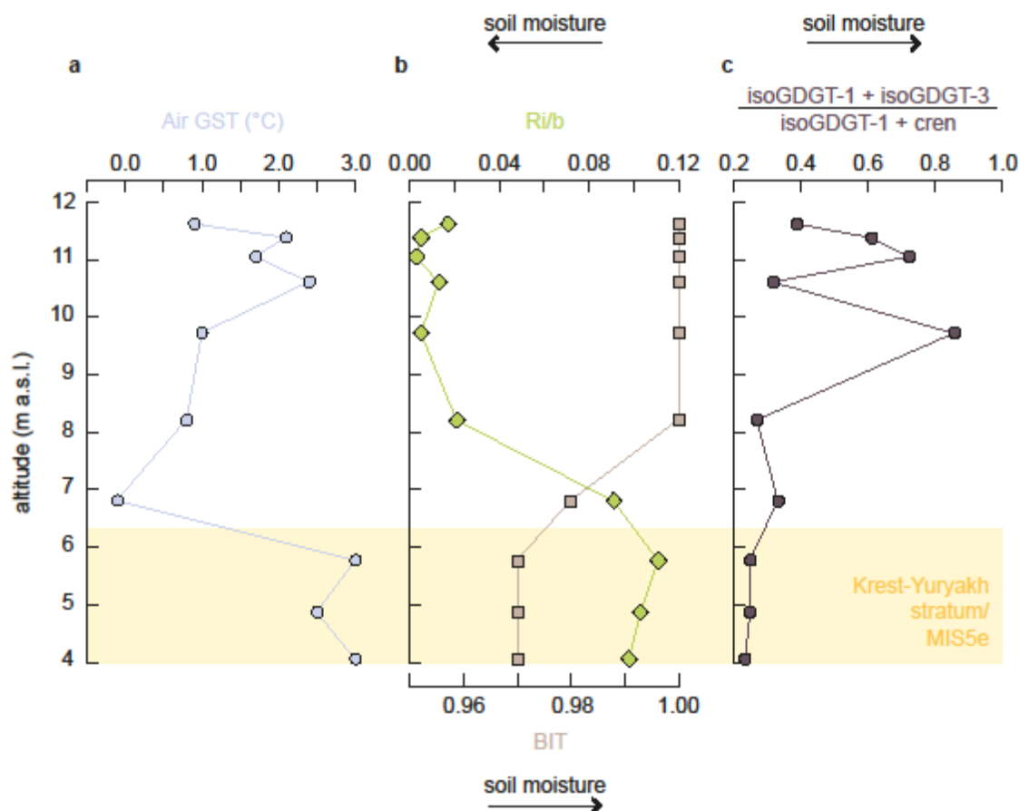
Figure 8. BrGDGT-based proxies in core L14-04: (a) MBT SME -based Air Growing Season Temperature (Air GST) following de Jonge et al. (2024); (b) branched and isoprenoid tetraether index (BIT) and ratio of isoGDGTs to brGDGTs (Ri/b); (c) ratio (\text{isoGDGT-1} + \text{isoGDGT-3})/(\text{isoGDGT-1} + \text{crenarchaeol}) .
