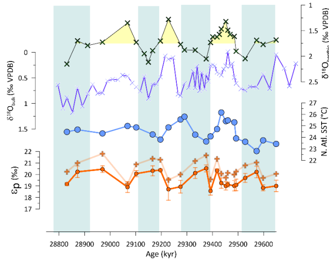
Figure 3. High resolution sampling from IODP 1406, showing \delta^{18}\text{O} of bulk carbonate and benthic foraminifera, alkenone SST estimates, and \epsilon_p calculated from bulk carbonate (circles) and benthic foraminifera assuming a constant offset (crosses).
