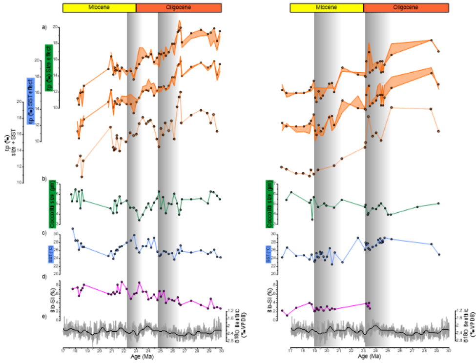
Figure 5: Timeseries of \epsilon_p at IODP 1406 and ODP 1168 including a) the measured \epsilon_p record (solid line) and the estimated \epsilon_p resulting once size and temperature effect is applied following Torres et al., (2024), and Stoll et al., (2019) (transparent shadows). b) Coccolith size record from Guitian et al., (2020); c) SST estimates d) Biogenic silica measurements (Guitian et al., (2020) and this study); e) reference CENOGRIID benthic \delta^{18}\text{O} curve (Westerhold et al., 2020)
