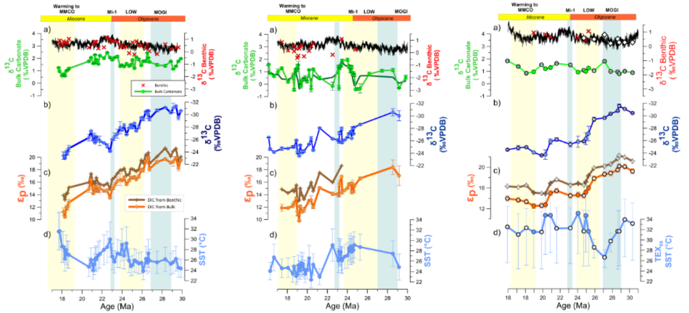
Figure 2: Analytical results of this study. a) Carbonate stable isotopes for benthic foraminifera (red crosses-symbols), data from this work for each site; black line shows results from Westerhold et al., (2020) and bulk sediment carbonate (green lines and circles). b) Alkenone C 37.2 δ 13 C. c) Calculated alkenone carbon fractionation, solid line DIC δ 13 C is derived from bulk carbonate, transparent line from picked benthic foraminifera at the same samples. d) Temperature estimates. IODP 1406, including SST and benthic δ 18 O dataset from Guitian et al., (2019); ODP 1168, dark green δ 13 C bulk carbonate shows the 4-point moving average used to calculate ε p at the site; ODP 925, filled circles are new measurements for this study, white symbols are published data (Zhang et al., 2013), being ε p recalculated following method described in text, SST is derived from GDGT at this site. Alkenone SST-derived show 1σ error bars and GDGTs 925-TEX 86 refer to 2σ.
