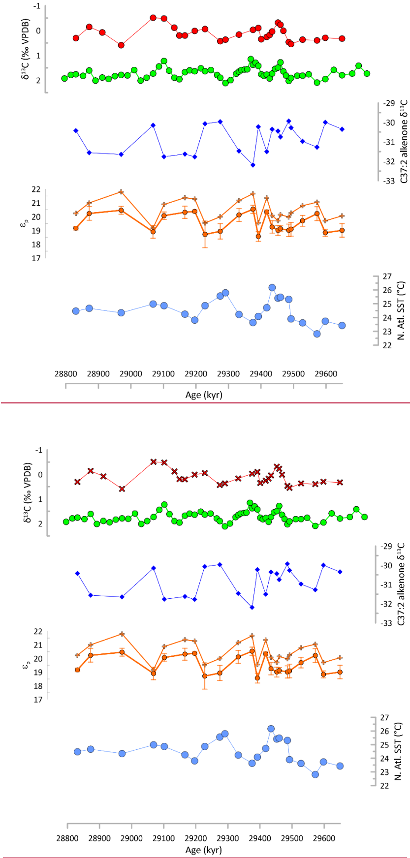
Figure S1. High resolution IODP 1406 subset of measured \delta^{13}\text{C} benthic foraminifera (red crosses), bulk carbonate (green circles), \text{C}_{37:2} alkenone, calculated \epsilon_p (where DIC \delta^{13}\text{C} derived from bulk carbonate is solid line and circles, from benthic foraminifera transparent line and crosses), and SST.
