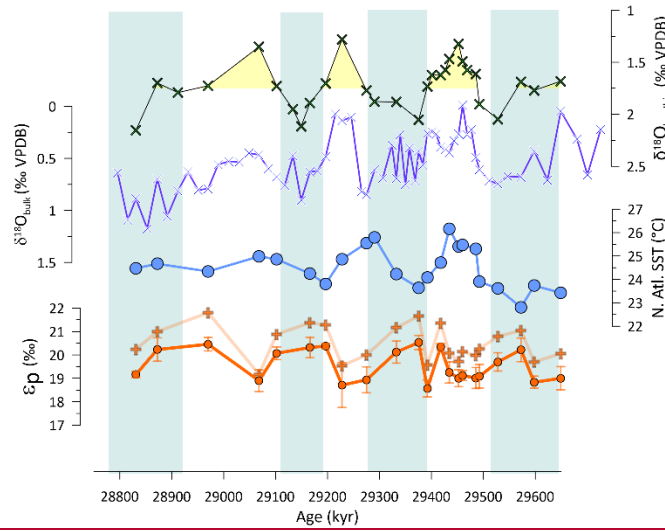
290 Figure 3. High resolution sampling from IODP 1406, showing \delta^{18}\text{O} of bulk carbonate and benthic foraminifera, alkenone SST estimates, and \epsilon_p calculated from bulk carbonate (circles) and benthic foraminifera assuming a constant offset (crosses).
