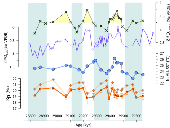
Figure 2: Analytical results of this study. a) Carbonate stable isotopes for benthic foraminifera (red crosses-symbols), data from this work for each site; black line shows results from Westerhold et al., (2020) and bulk sediment carbonate (green lines and circles). b) Alkenone C 37.2 δ 13 C. c) Calculated alkenone carbon fractionation, solid line DIC δ 13 C is derived from bulk carbonate, transparent line from picked benthic foraminifera at the same samples. d) Temperature estimates. IODP 1406, including SST and benthic δ 18 O dataset from Guitian et al., (2019); ODP 1168, dark green δ 13 C bulk carbonate shows the 4-point moving average used to calculate ε p at the site; ODP 925, filled circles are new measurements for this study, white symbols are published data (Zhang et al., 2013), being ε p recalculated following method described in text, SST is derived from GDGT at this site. Alkenone SST-derived show 1σ error bars and GDGTs 925-TEX 86 refer to 2σ.
