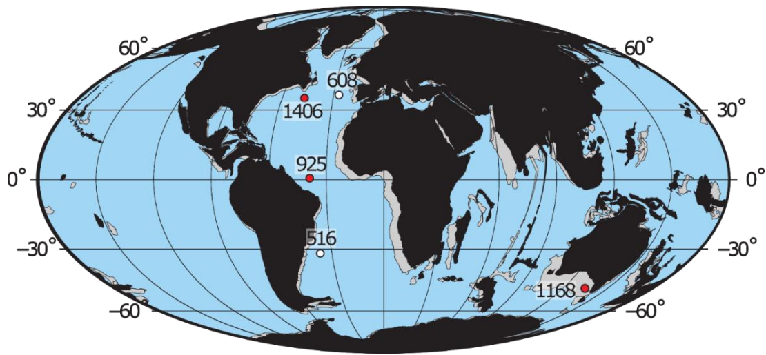
160 Figure 1. Location of the study sites. Reconstructed map of continental distribution over the 30 Ma (grey) – 17 Ma (black) time interval. Modified after the plate tectonic reconstruction service from the Ocean Drilling Stratigraphic Network ( https://www.odsn.de/ ) using the data from Hay et al. (1999).
