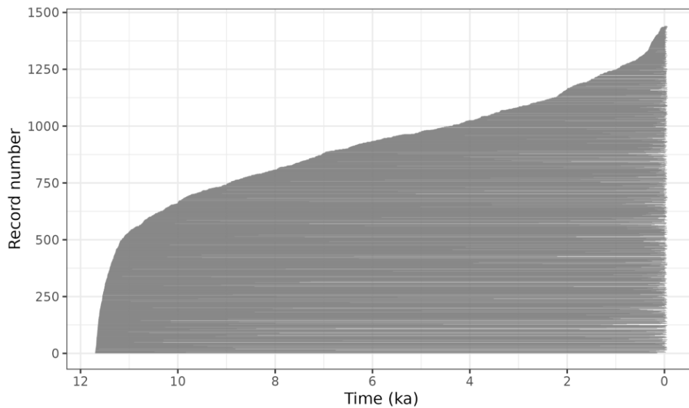
Figure 1: The spatiotemporal distribution of fossil pollen data used here. A) Map indicating the spatial distribution of sites recovered from the Neotoma Paleoecology Database, as well as the case study regions (WCAN/AK: Western Canada and Alaska; PCCS: Pacific Coast, Cascades, and Sierra Nevada; ECAN: Eastern Canada; and NEUS/SEC: North-Eastern US and South-Eastern Canada). B) Temporal extent of all sites, in which each site is represented by a horizontal gray line between the site's oldest and youngest Holocene samples. Sites are ordered by age of the oldest sample, reported as ka. Samples older than 11.7 ka are not shown.
