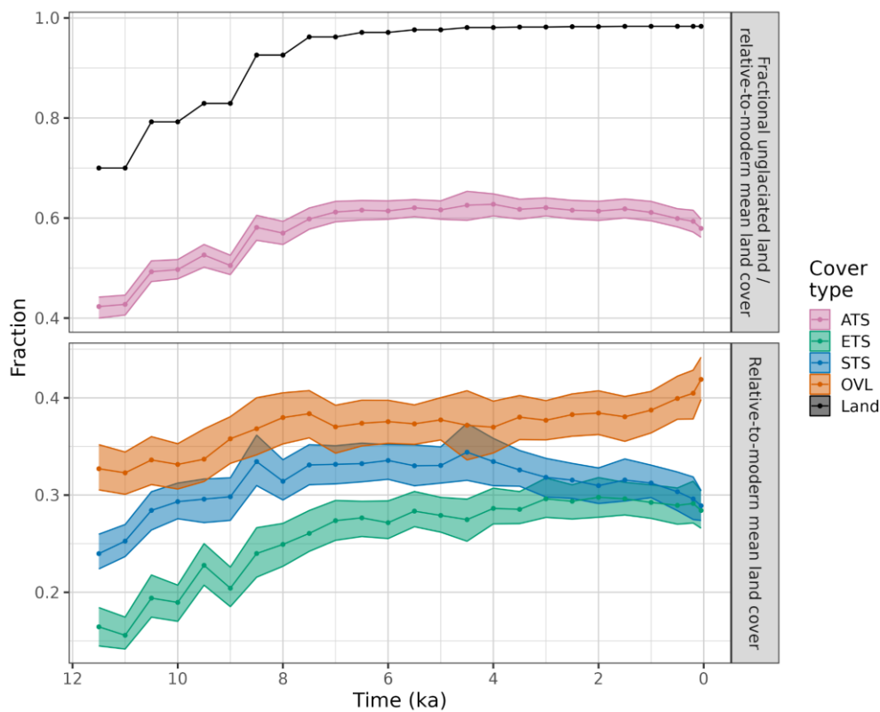
353 354 Figure 3: (a) Holocene trends in relative-to-modern mean land cover for weighted cover of all trees 355 and shrubs (ATS) in North America (pink curve with 95% uncertainty envelope), expressed relative to 356 present unglaciated land area (see Methods), and the fraction of unglaciated land relative to continental 357 land area (black). ATS is the sum of the evergreen and summergreen trees and shrubs. (b)
