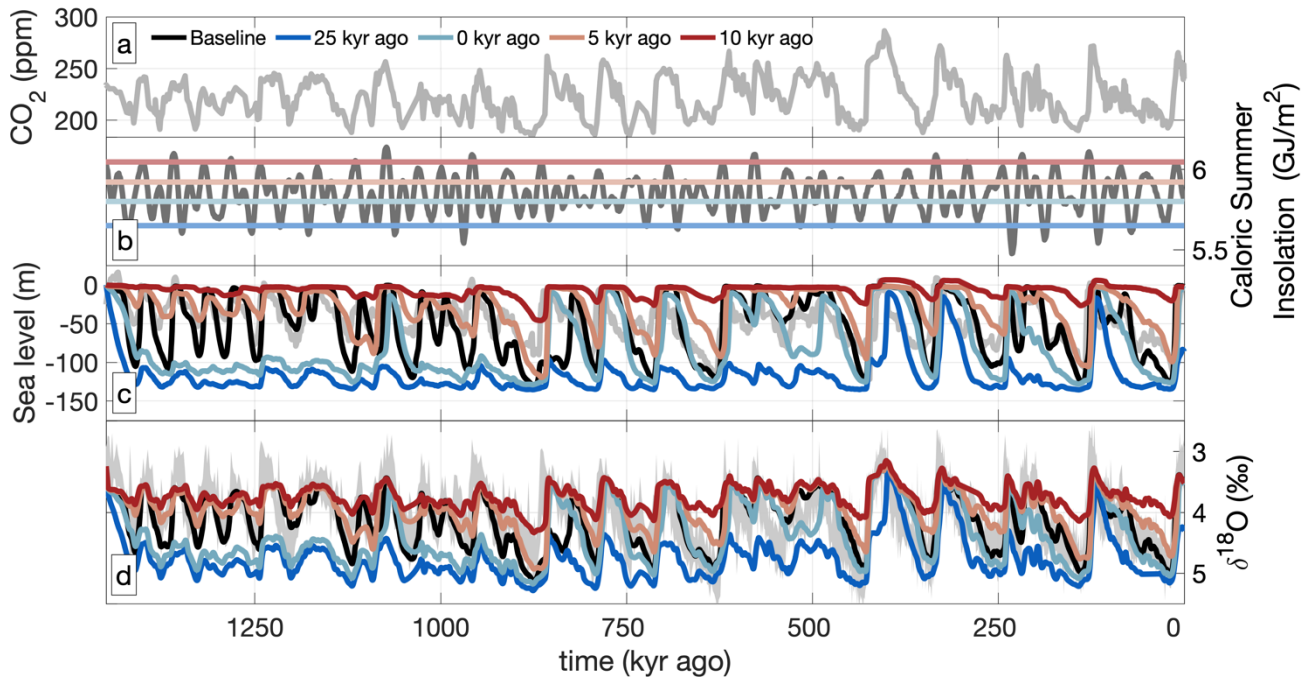
Figure 7. Time-series of prescribed \text{CO}_2 (a), insolation (b), sea level (c) and \delta^{18}\text{O} (d). \text{CO}_2 reconstruction by Yamamoto et al. (2022; a), sea-level by Rohling et al. (2012; c), and \delta^{18}\text{O} Ahn et al (2017; d) all shown in grey.
