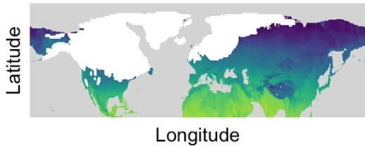
Beyer 5-min model (WC) - LGM
