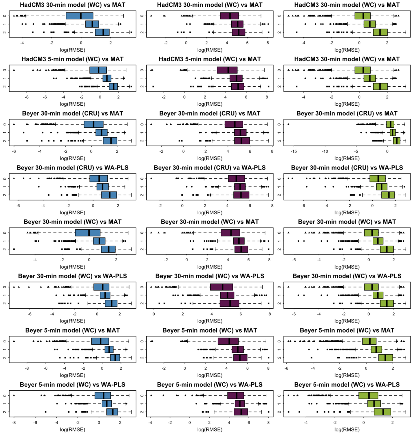
Figure 5. Boxplots of pair-wise log root mean square error (RMSE) results model-data comparisons of mean annual temperature (blue), mean annual precipitation (purple) and mean July temperature (green) from those representing the present (0), MIS 1 (1) and MIS 2 (2).
