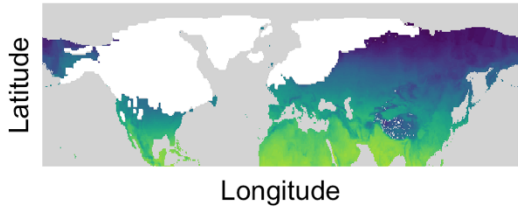
Beyer 30-min model (WC)- LGM
