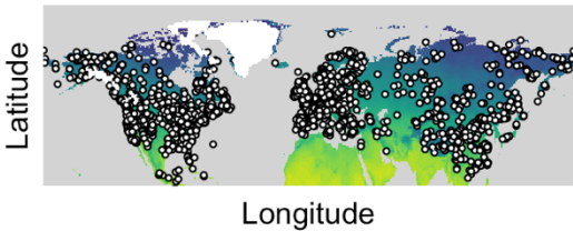
Beyer 5-min model (WC) - present day
