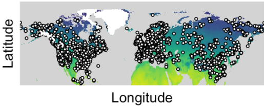
Beyer 30-min model (WC) - present day
