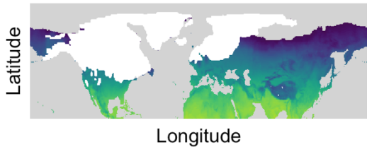
HadCM3 30-min model (WC) - LGM
