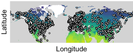
HadCM3 30-min model (WC) - present day
