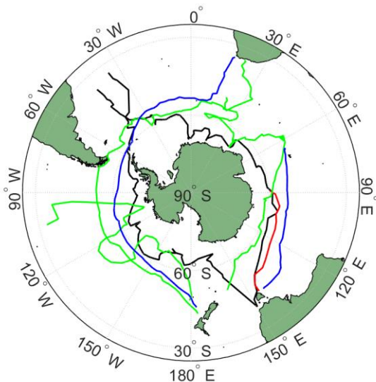
Figure 1: Southern Ocean sections of the voyages considered in this paper; green line: Resolution , blue line: Adventure , black line: Vostok , red line: Mirny . Note that Cook's outward South Atlantic section is not shown until he encountered ice (~ 50.7°S, 20.3°E), while his return is shown all the way to Cape Town.
