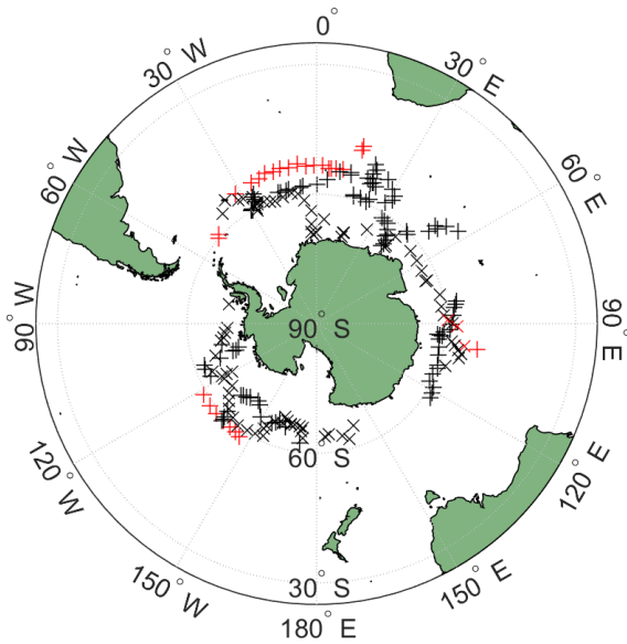
Fig. 5: Iceberg observations recorded by the voyages of Cook ('+') and Bellingshausen ('x'). These include any iceberg sightings, so cover all records of category '1' to '3'. Note that additional observations from the Adventure , for Cook's expedition, and the Mirny , for Bellingshausen's, are shown in red.
