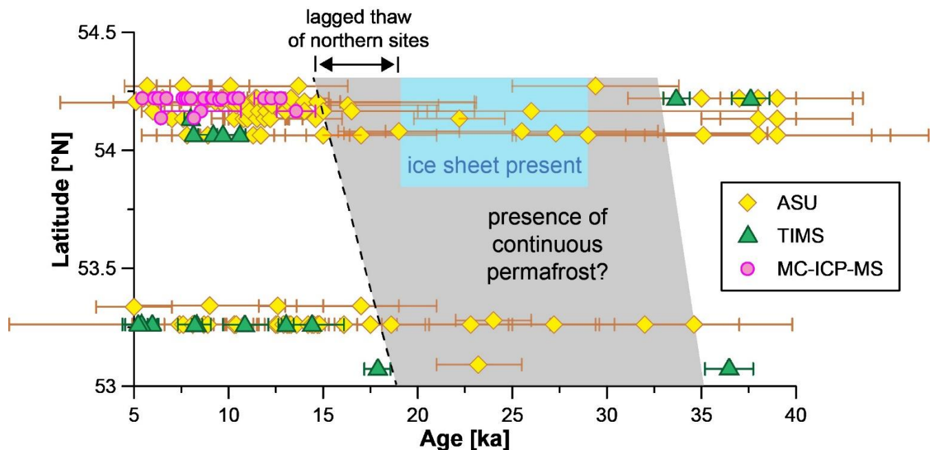
355 Figure 6: Distribution of speleothem ages in northern England between 40 and 5 ka based on the three different dating methods. Ice presence inferred from the empirical British-Irish Ice Sheet reconstruction minimal to optimal extent (Clark et al., 2022b). Inferred potential presence of continuous permafrost based on available TIMS and MC-ICP-MS dates.
