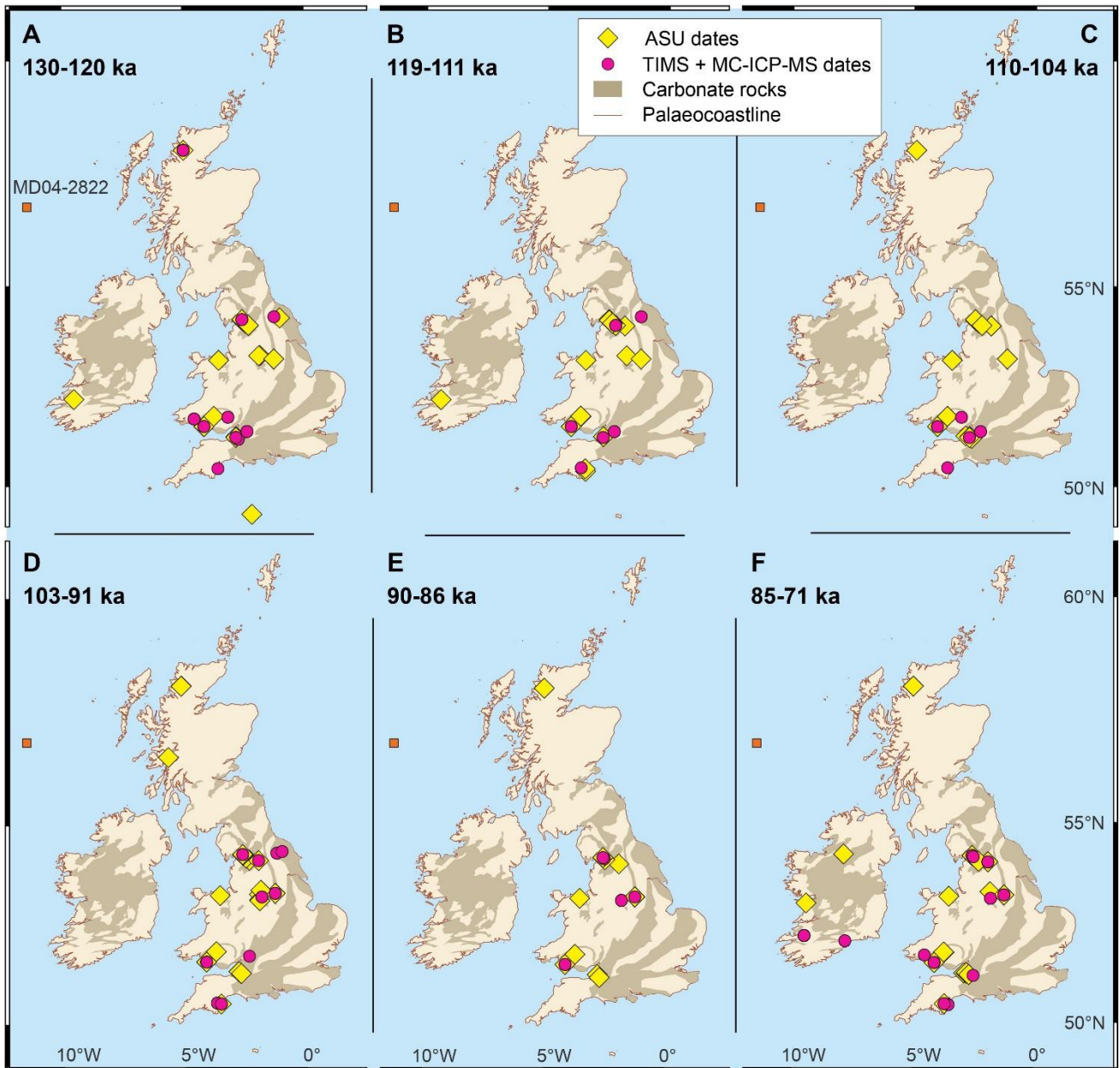
380 Figure 8: Speleothem growth in the British Isles during selected time intervals from 130 to 71 ka, and location of site MD04-2822 (Hibbert et al., 2010). Distribution of carbonate rocks from World Karst Aquifer Mapping project (Chen et al., 2017).
