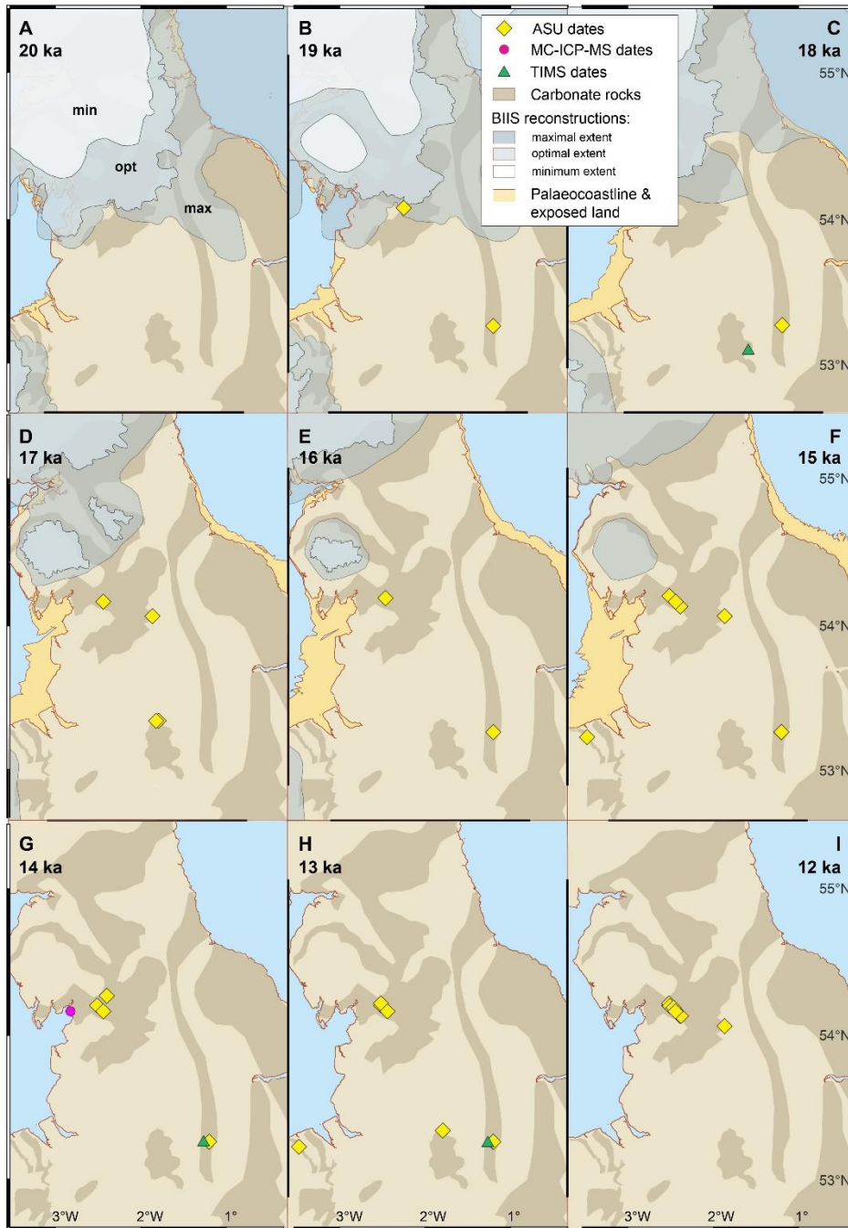
375 Figure 7: Speleothem growth in northern England from 20 to 12 ka. (A-F) Empirical British-Irish Ice Sheet reconstruction (BIIS) (minimal, optimal and maximum extent) and modelled position of palaeo-coastline from Clark et al. (2022b). Distribution of carbonate rocks from World Karst Aquifer Mapping project (Chen et al., 2017).
