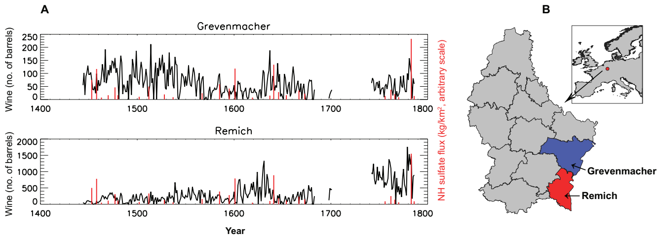
Figure 1. A Annual wine production in number of barrels for each series ( in black ) and volcanic sulfate flux derived from Greenland sulfate deposition in \text{kg}/\text{km}^2 ( in red ). B Location of the two sites with wine data from 1444–1786 (with gaps) in the Moselle Valley of Luxembourg.
