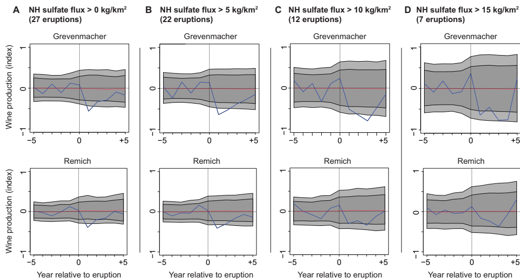
Figure 2. Superposed epoch analysis (SEA) of volcanic forcing, after NH sulfate flux kg/km^2 size, on standardised wine production quantity for Grevenmacher, Remich. The grey bands indicate p = 0.05 (light grey) and p = 0.01 (dark grey) significance levels, calculated by a bootstrap method (randomly selected key years).
