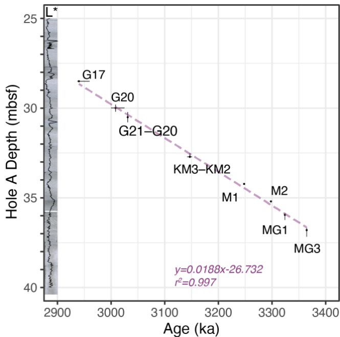
Figure 4: Age-depth plot of Site 1168 Hole A along with core photos (Core3H6W–Core5H3W) and L^* colour reflectance in the late-Pliocene. Tie points are presented in Fig. 3. Vertical error bars indicate potential errors in depth when tie points are assigned based on \delta^{18}O_{bf} and \delta^{18}O_{bulk} , see Table S1; Purple dashed line=linear regression, for an estimation of sedimentation rate, which is used for dinocyst burial flux calculation, see supplementary data and Fig. S1.
