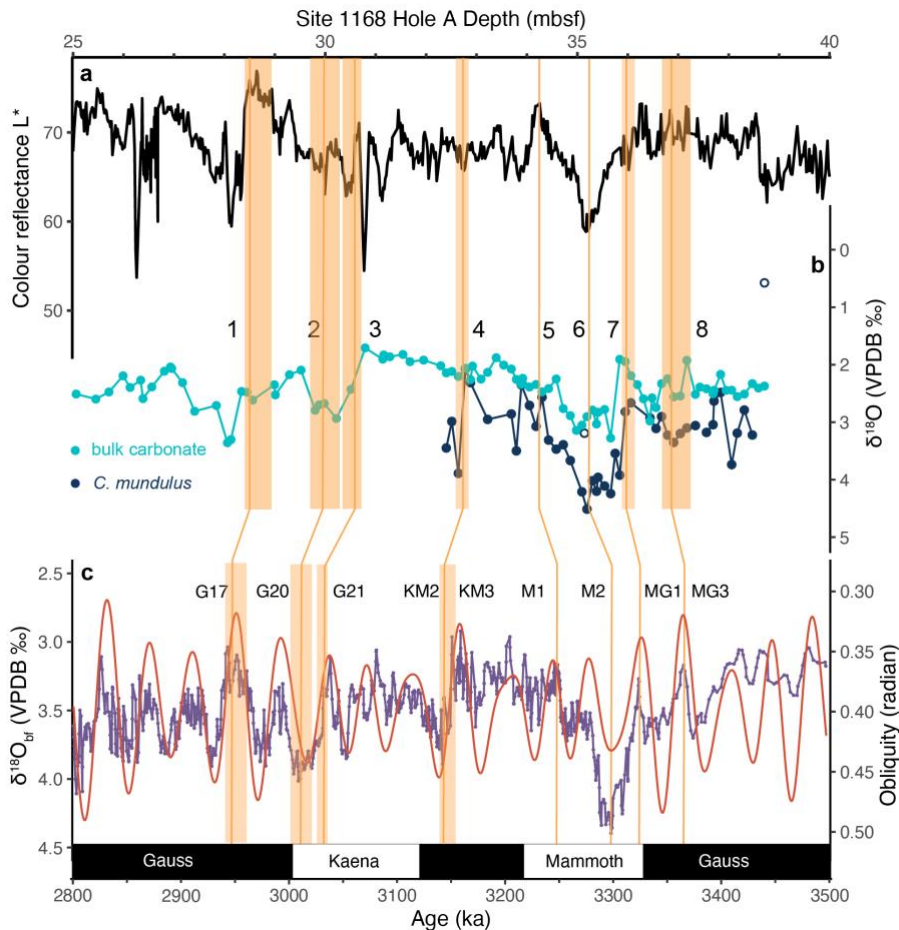
Figure 3: Age tuning for the Pliocene of ODP Site 1168 Hole A. (a) L^* colour reflectance of Site 1168A (Exon et al., 2001). (b) \delta^{18}\text{O}_{\text{br}} and \delta^{18}\text{O}_{\text{bulk}} of Site 1168A, (c) CENOGRID (Westerhold et al., 2020) and obliquity insolation curve (Laskar et al., 2004) using the software Acycle (Li et al., 2019). Orange lines=tie points; Orange rectangles= errors in depth or age.
