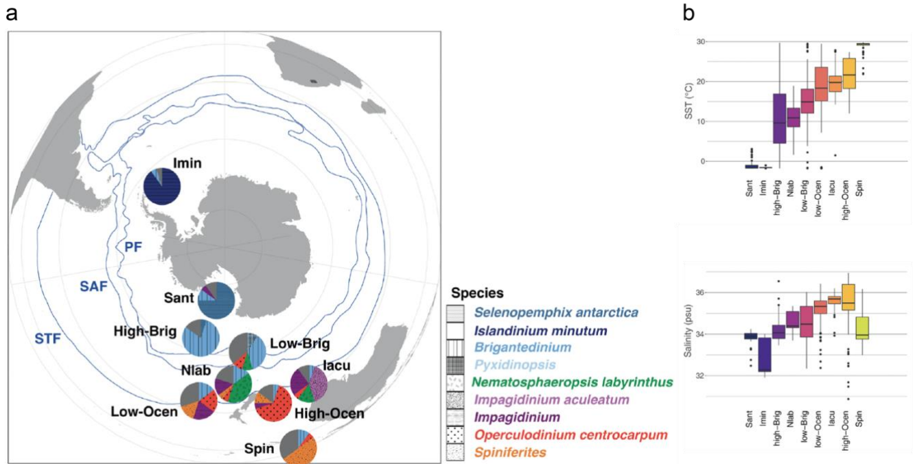
Figure 2: (a). Schematic representation of the generalized biogeographic distribution of dinocysts in Southern Ocean surface sediments. Pies represent average assemblage composition of the nine clusters described in this paper. Position of these pies represent their typical latitudinal band of occurrence. Also plotted are the frontal systems (blue lines, STF = Subtropical Front, SAF = Subantarctic Front, PF = Polar Front). The Subantarctic Zone (SAZ) is the water mass between the STF and PF. (b) Comparison of sea surface temperature and sea surface salinity in different clusters for the 9-cluster solution of the modern distribution. The median, 25% – 75% quantiles and 95% confidence interval are indicated by the black line, boxes and whiskers, respectively. Modified from Thöle et al. (2023).
