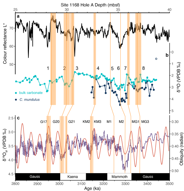
205 Figure 3: Age tuning for the Pliocene of ODP Site 1168 Hole A. (a) L^* colour reflectance of Site 1168A (Exon et al., 2001). (b) \delta^{18}\text{O}_{\text{br}} and \delta^{18}\text{O}_{\text{bulk}} of Site 1168A, (c) CENOGRID (Westerhold et al., 2020) and obliquity insolation curve (Laskar et al., 2004) using the software Acycle (Li et al., 2019). Orange lines= tie points; Orange rectangles= errors in depth or age.
