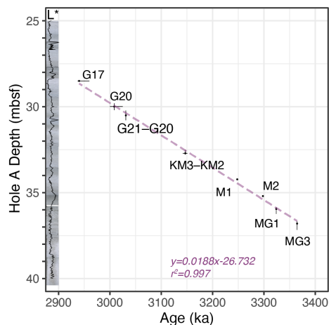
215 Figure 4: Age-depth plot of Site 1168 Hole A along with core photos (Core3H6W–Core5H3W) and L* colour reflectance in the late-Pliocene. Tie points are presented in Fig. 3. Vertical error bars indicate potential errors in depth when tie points are assigned based on \delta^{18}\text{O}_{\text{br}} and \delta^{18}\text{O}_{\text{bulk}} , see Table S1; Purple dashed line=linear regression, for an estimation of sedimentation rate, which is used for dinocyst burial flux calculation, see supplementary data and Fig. S1.
