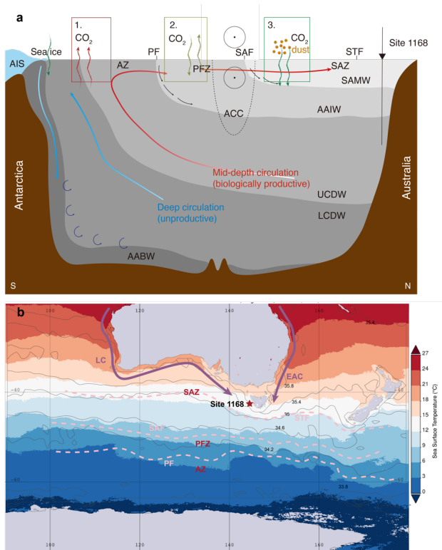
95 Figure 1: (a) Schematic view of the ocean circulation in the Southern Ocean between Antarctica and Australia. Arrows in the ocean denote southern overturning circulation (blue), mid-depth overturning circulation (red); grey areas depict water masses; 100 SAMW=subantarctic mode water, AAIW=Antarctic Intermediate Water, U/LCDW=Upper/Lower Component Deep Water, AABW=Antarctic Bottom Water, ACC=Antarctic Circumpolar Current; Curvy arrows denote CO 2 uptake or outgassing processes (1. Deep ocean degassing, red; 2. Physical diffusion, spring green; 3. Biological carbon pump, green). (b) Modern site location of ODP Site 1168. Colors indicate sea surface temperatures; Contours indicate sea surface salinity; Grey blocks indicate modern 105 coastline and sea ice extent. Purple arrows denote ocean currents (LC=Leeuwin Current, EAC=East Australia Current). Pink dashed lines denote oceanic fronts (STF=Subtropical Front, SAF=Subantarctic Front, PF=Polar Front) and ocean zones in between (SAZ=Subtropical/Subantarctic Zone, PFZ=Polar Frontal Zone, AZ=Antarctic Zone) are mentioned in red. Data, map and visualization were generated using the Giovanni online data system ( https://giovanni.gsfc.nasa.gov/giovanni/ ) developed and maintained by the National Aeronautics and Space Administration Goddard Earth Sciences Data and Information Services Center (Acker and Leptoukh, 2007). SST and SSS data are derived from Moderate Resolution Imaging Spectroradiometer on the Aqua satellite (MODIS-Aqua) provided to Giovanni by the Ocean Biology Distributed Active Archive Center.
