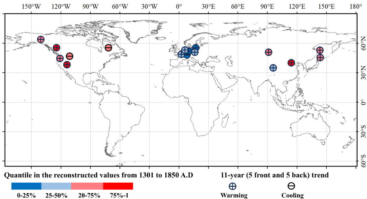
380 Figure 6: Behaviour in the rest of the Northern Hemisphere during the summer of 1743.
