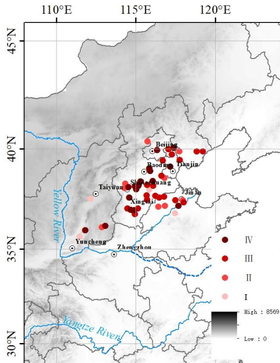
235 Figure 3: Spatial pattern of heat severity.
