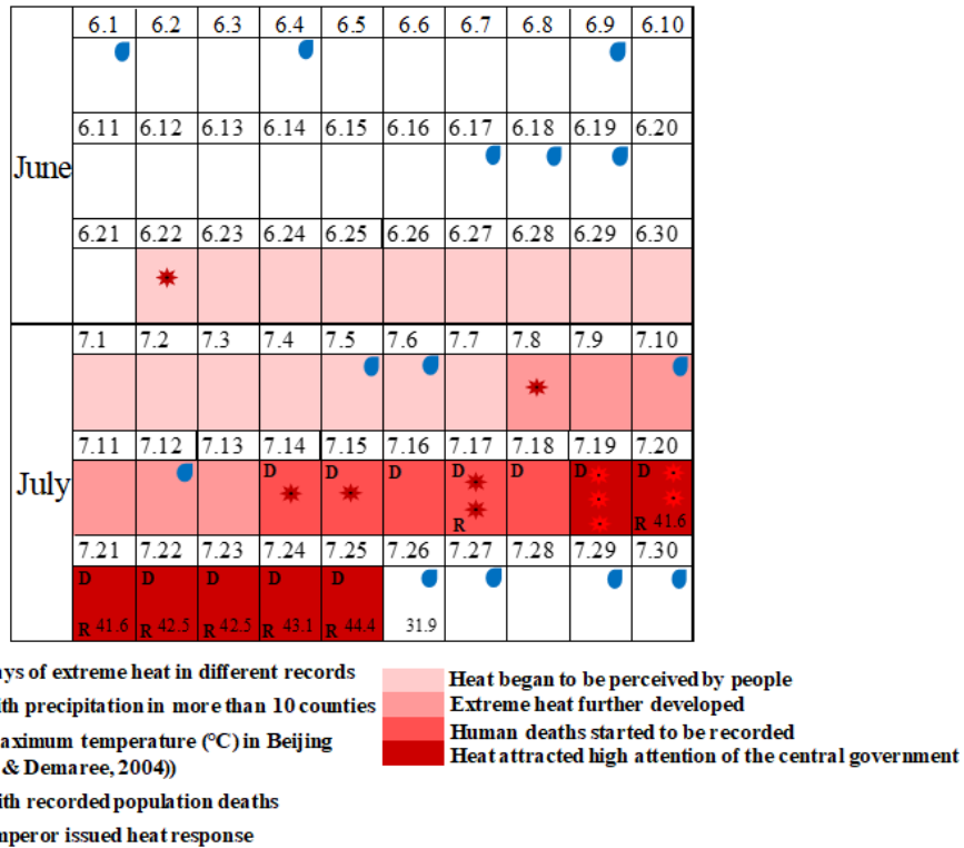
Figure 2: Processes over time during the 1743 extreme heat event (in the form of a calendar).
