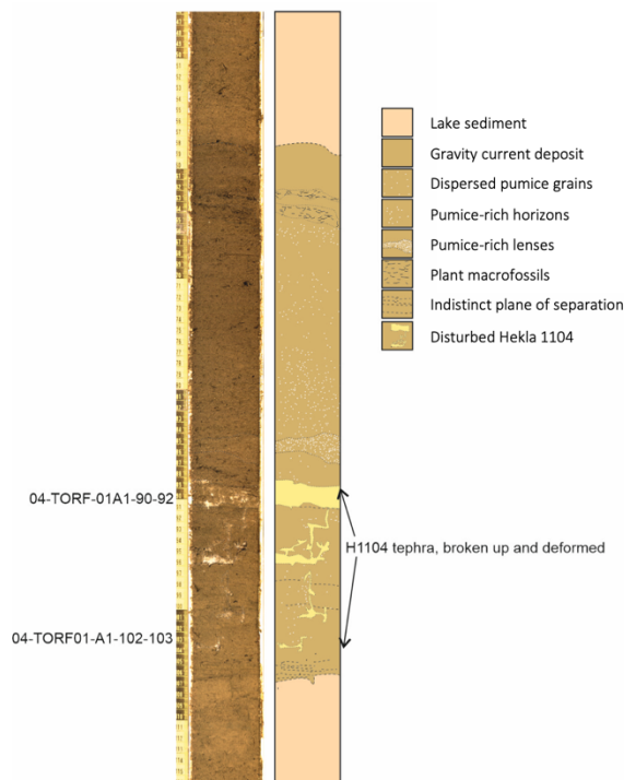
545 Figure 8: Lithostratigraphy of the deformed Hekla 1104 CE tephra layer (i.e., tephra-seismitite) in core 2004NC. On the left is a photo image and on the right is a simplified schematic based on the major identified sediment types.
