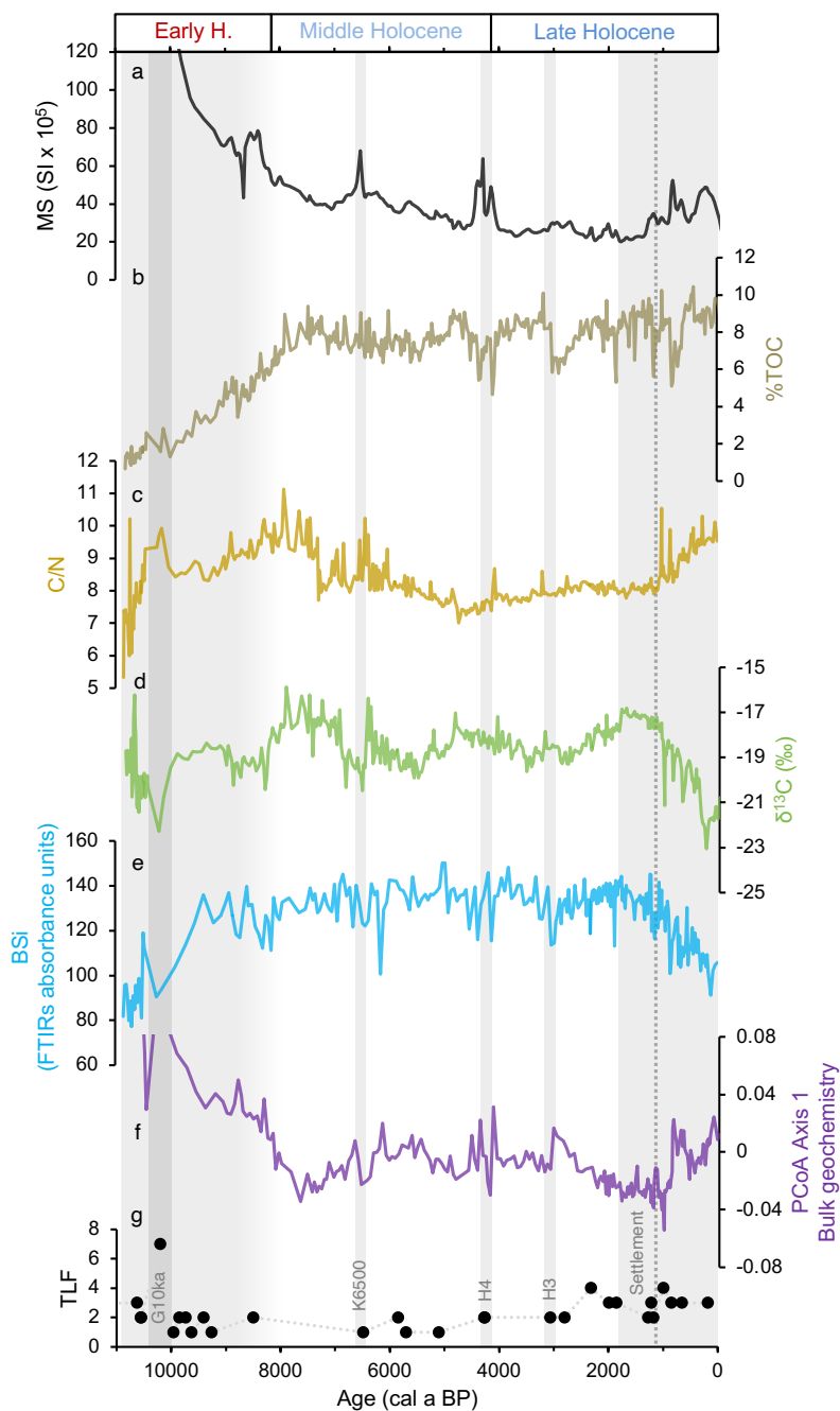
275 Figure 4: Bulk physical and geochemical proxy records (a-e), PCoA Axis 1 of bulk geochemistry proxies (f), and tephra layer frequency (TLF, g) from core 2012NC. Note that MS in panel a is truncated at 120 SI x 10 5 and values at the base of the record reach up to 523 SI x 10 5 . Grey bars reflect landscape disturbances associated with large tephra layer deposits and erosion and dashed gray line denotes the timing of presumed human settlement (1080 cal a BP).
