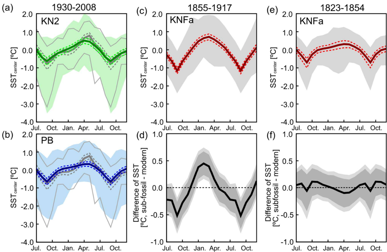
410 Figure 7: Mean seasonal cycles of SST center derived from modern and sub-fossil Enggano corals. (a) 1930-2008, core KN2 (in green; solid line is monthly mean, dashed green lines are \pm 1\sigma , green shading indicates 99 % percentiles of monthly means). Satellite SST data (Huang et al., 2021) (mean removed, thick grey line is monthly mean, dashed grey lines are \pm 1\sigma ; thin grey lines are 99 % percentiles of monthly means) are shown for comparison. (b) Same as (a), but for core PB (in blue; solid line is monthly mean, dashed blue lines are \pm 1\sigma , blue shading indicates 99 % percentiles of monthly means). (c) Same as (a) but for core KNFa in the time period from 1855-1917 (in red; solid line is monthly mean, dashed red lines are \pm 1\sigma , grey shading indicates 99 % percentiles of monthly means), (d) Difference of mean seasonal cycles: (1930-2008 monthly average data of KN2 and PB) minus (1855-1917 of monthly average data of KNFa), with 95 and 99 % confidence levels (dark and light shading, respectively) based on a 20 000 sample Monte Carlo. Note the inflated y-axis. (e) and (f) same as (c) and (d) for the time period from 1823-1854 (KNFa). 415
