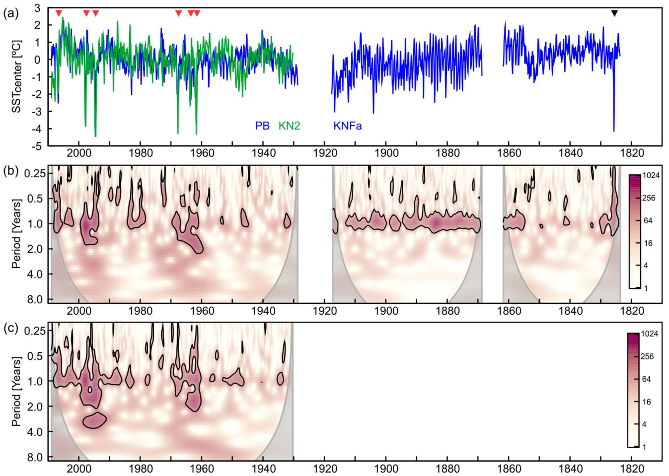
365 Figure 6: Modern and sub-fossil, monthly SST center inferred from Enggano coral Sr/Ca ratios. (a) The monthly SST center record from Enggano comprises two modern (PB, KN2) and one sub-fossil core (KNFa) and extends from 1930-2008, 1869-1917 and 1823-1861. Note that the sub-fossil coral chronology is based on U/Th dating with an age uncertainty of \pm 2.4 years ( 2\sigma ). Extreme pIOD events lead to cooling of \geq -4 °C in 1961, 1963, 1967, 1994, 1997 and 2006 (red arrows). The sub-fossil core KNFa shows an extreme pIOD event on par with the event in 1997 in 1825 (black arrow). (b) Wavelet power spectra of SST center time series of core PB and KNFa. (c) same as (b) but for core KN2. Power spectra of PB and KN2 are dominated by extreme pIOD events (red arrows in a). SST center of KNFa shows enhanced seasonal variability between 1855 and 1917. Prior to 1855, seasonal variability is comparable to PB and KN2. Wavelet Power spectra were computed in R using the Morlet Wavelet. Thick black lines indicate significant periodicities at a certain time ( p < 0.05 ). Grey shading indicates cone of influence.
