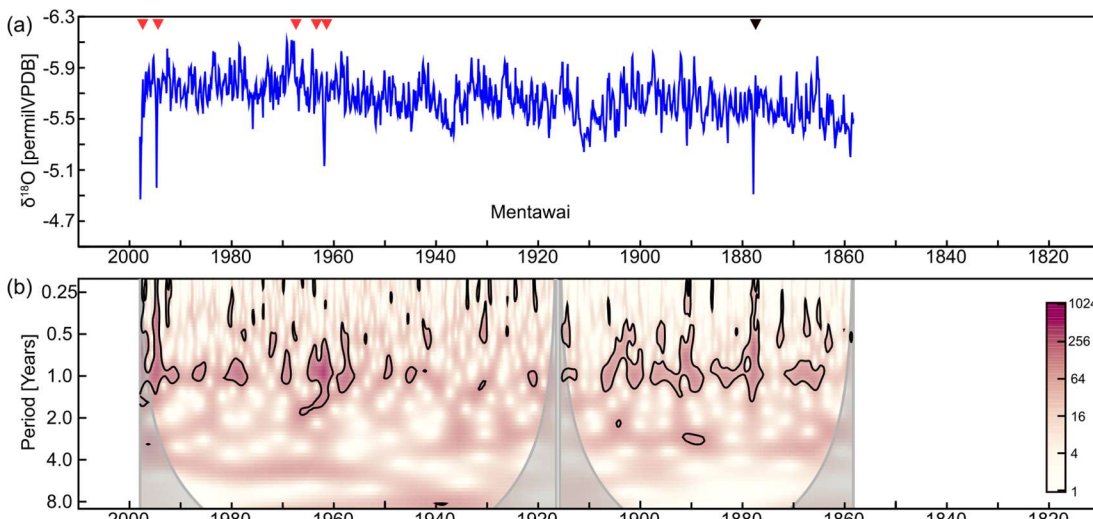
540 Figure 10: Monthly coral \delta^{18}\text{O} record from northern Mentawai from (Abram et al., 2008). (a) monthly mean coral \delta^{18}\text{O} (thin blue lines) and ten-year running averages (thick red line) from 1858-1997. Red arrows mark extreme pIOD events seen in the Sr/Ca record from Enggano (Pfeiffer et al., 2022). Note: The Mentawai coral record does not record the events of 1963 and 1967. One extreme pIOD event is recorded in 1877 (black arrow). (b) Wavelet Power spectrum of the Mentawai record, with largest variability on interannual periodicities. Wavelet Power spectrum was computed in R using the Morlet Wavelet. Thick black lines indicate significant periodicities at a certain time (p<0.05). Grey shading indicates cone of influence. 545
