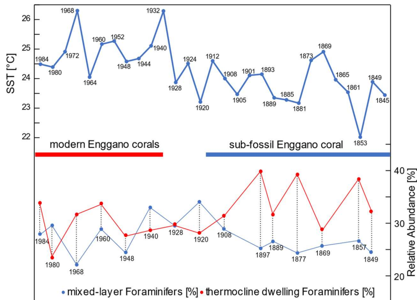
550 Figure 11. Top: Mean SSTs inferred from Foraminiferal Mg/Ca ratios from a sediment core taken off Sumba Island (Steinke et al., 2014a; Steinke et al., 2014b). Each dot represents one measurement, with estimated ages of (Steinke et al., 2014b). Red (blue) horizontal bars indicate time period covered by modern (sub-fossil) coral records from Enggano Island. Bottom: Relative abundance of mixed layer (blue dots) and thermocline dwelling (red dots) foraminifera (Steinke et al., 2014b). See text for discussion.
