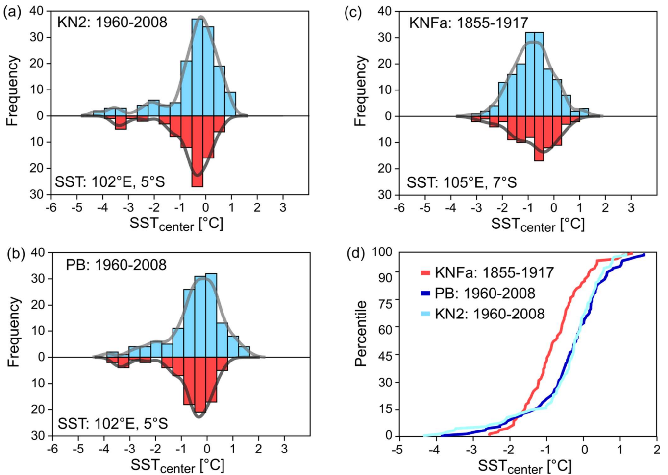
Figure 8: (a)-(c): Distribution of September-November monthly mean SST centre inferred from the Enggano Sr/Ca records (in blue) compared to satellite SSTs (in red, OI SST, 1/4° grid, 1982-2008, centred to its mean) (Huang et al., 2021). Thick grey lines are the Kernel density functions of the histograms. (a, b) Modern September-November SST centre (KN2 and PB) from 1960-2008 shows the same distribution as SSTs in the grid centred at Enggano island. The negative skewness reflects the occurrence of extreme pIOD events. Between 1855-1917, September-November SST centre (KNFa) shows a symmetric distribution, comparable to the SST distribution seen today at 7°S. (d) Percentiles of SST centre shown in (a), (b) and (c). See Table A3 and A4 for a comparison of the distributions using a Kolmogorov-Smirnov test. Histograms and percentiles were computed using PAST (Hammer et al., 2001).
