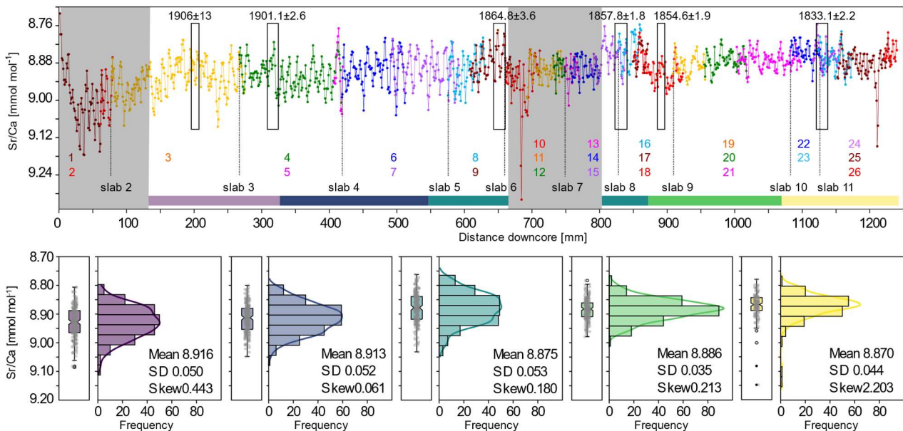
280 Figure 5: Sub-fossil coral Sr/Ca data of core KNFa. Top panel: Measured Sr/Ca data of core KNFa vs. distance downcore (in mm). Each dot corresponds to one Sr/Ca measurement. Sampling transects are highlighted by different colors and numbered (bottom) (see Fig. 4 for location of transect). Grey shading marks intervals discarded from further interpretation as diagenetic alterations have been detected. Sections sampled for U/Th ages are shown by black rectangles. Color bars at the bottom indicate data included in the histograms, box- and jitter-plots shown in the bottom panel. Note the reduction in the standard deviation of measured Sr/Ca data at a depth of \sim 860 mm. Histograms computed using PAST (Hammer et al., 2001).
