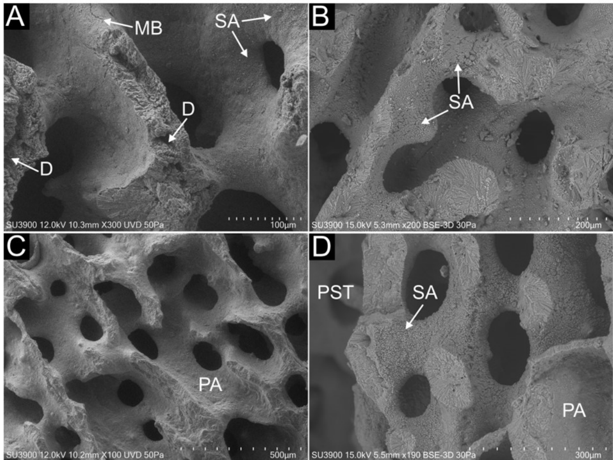
Figure A6: Scanning electron microscopy images showing pristine and diagenetic altered parts of sub-fossil coral KNFa. The top 14 cm of the core shows several macroscopic bioerosion traces on x-ray images (Fig. 4). This interval (a and b) is characterized by filamentous microborings (MB), dissolution (D) of centers of calcification and secondary aragonite (SA) cement. The degree of cementation is variable, ranging from (a) pristine coral skeletons and traces of cement to (b) more pervasive fibrous aragonite cement (5 to 10 \mu\text{m} -length). The interval below 14 cm is generally pristine (c) showing smooth primary aragonite (PA) skeletal surfaces. The only exception occurs in an interval from the base of slab 5 to the top of slab 7 (Fig. 5). A patch of secondary aragonite cement on transect 10 of slab 6 caused an extreme spike in the proxy record with unusually low Sr/Ca ratio of 9.32 mmol/mol. This 'false alarm' spike escaped detection by our first standard diagenetic screening, but was identified by our semi contentious SEM screening along the proxy sampling track.
