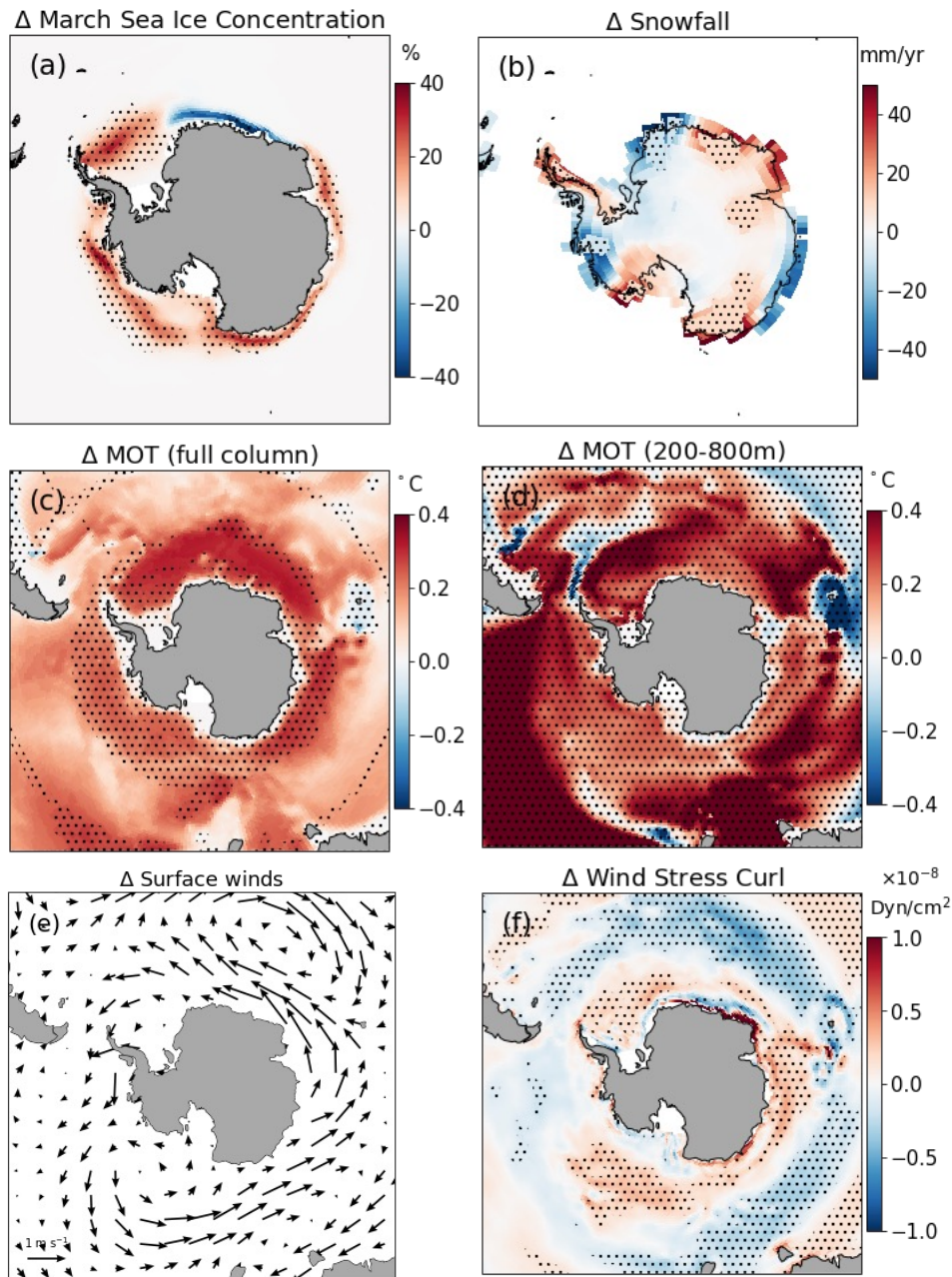
Figure 4. Climate anomalies between 127ka and piControl . Climatological 127ka anomaly of minimum (March) sea ice concentration (a), snowfall rate (hatching indicates significance) (b), mean ocean temperature (MOT) for the full ocean column (c), MOT (200-800m only) (d), surface winds (e) and wind stress curl (f). Anomalies are with respect to piControl . Climatologies are computed over Hatching indicates significance at the last 50 years of each simulation 95% confidence level.
