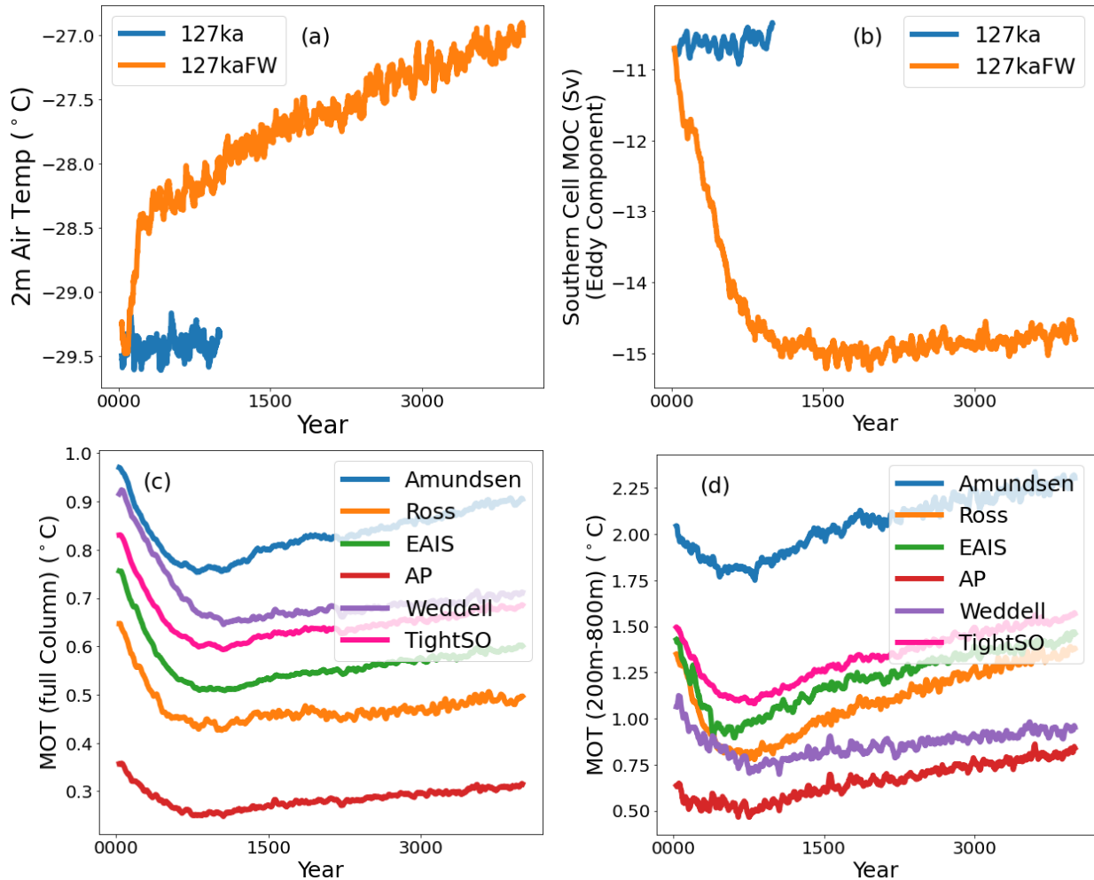
Figure 7. Antarctic and Southern Ocean response to 127kaFW forcing. All curves show 30-year rolling means. (a) Near-surface air temperature over the Antarctic continent ( land points ). (b) Global meridional overturning circulation (MOC) lower cell strength. Location extracted where minimum streamfunction is located, below 2km depth and south of 33^{\circ}\text{S} . Larger negative values indicate stronger circulation (negative indicates counterclockwise flow). (c) Mean ocean temperature (MOT) for the full ocean column in different sectors near the continent (sectors follow Fig. 3). (d) Same as (c) but for depths from 200–800 m.
