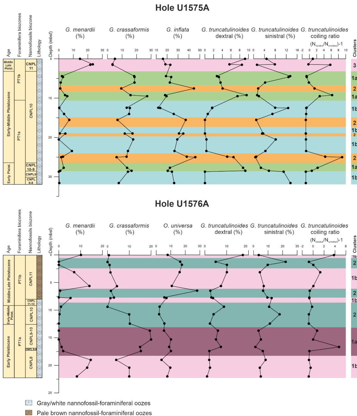
Fig. 3: Relative abundances (%) plotted against depth (mbsl) of the planktonic foraminiferal species which define the clusters in Holes U1575A and U1576A. The figure also shows the ratio between right and left-coiling tests of Globorotalia truncatulinoides . Foraminifera and calcareous nannofossils biozonations as well as the lithological units are also indicated.
