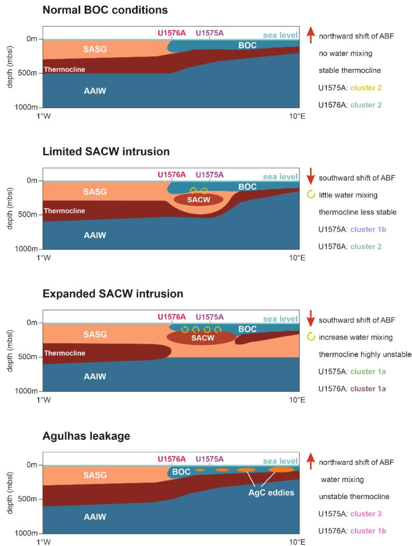
Fig. 6: Conceptual model showing the interaction between the SACW, BOC and AgC water masses in the studied area. BOC=Benguela Offshore Current; SACW=South Atlantic Central Water; SASG=South Atlantic Subtropical Gyre waters; AAIW=Antarctic Intermediate Water; AgC=Agulhas Current. The clusters for Holes U1575A and U1576A associated with each paleoceanographic condition are also indicated. The local thermocline is represented as a dark orange area.
