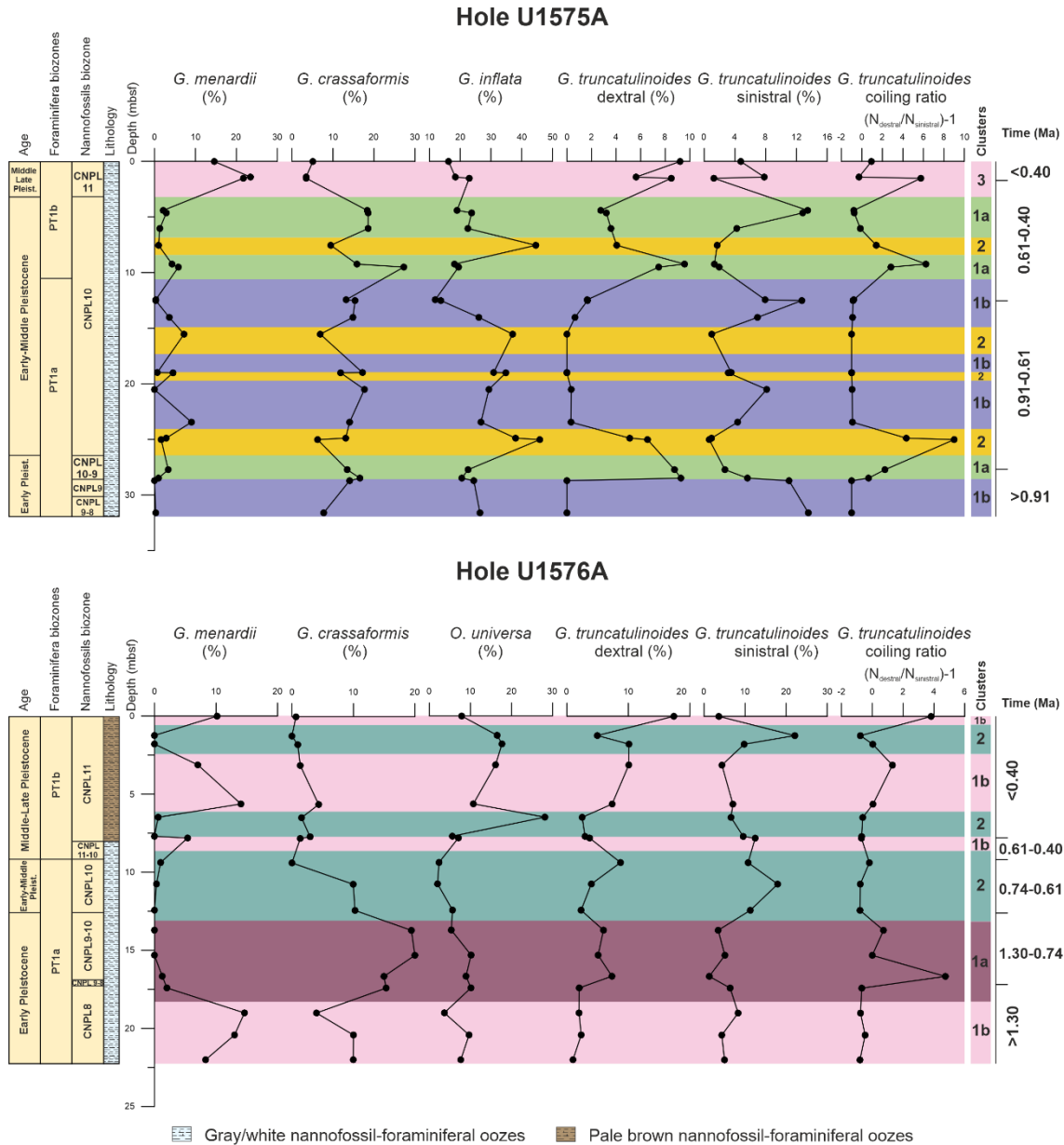
Fig. 3: Relative abundances (%) plotted against depth (mbsf) of the planktonic foraminiferal species which define the clusters in Holes U1575A and U1576A. The figure also shows the ratio between right and left-coiling tests of Globorotalia truncatulinoides . Foraminifera
