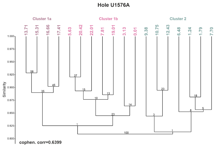
Fig. 4: UPGMA dendrograms of cluster analysis for Holes U1575A and U1576A.
