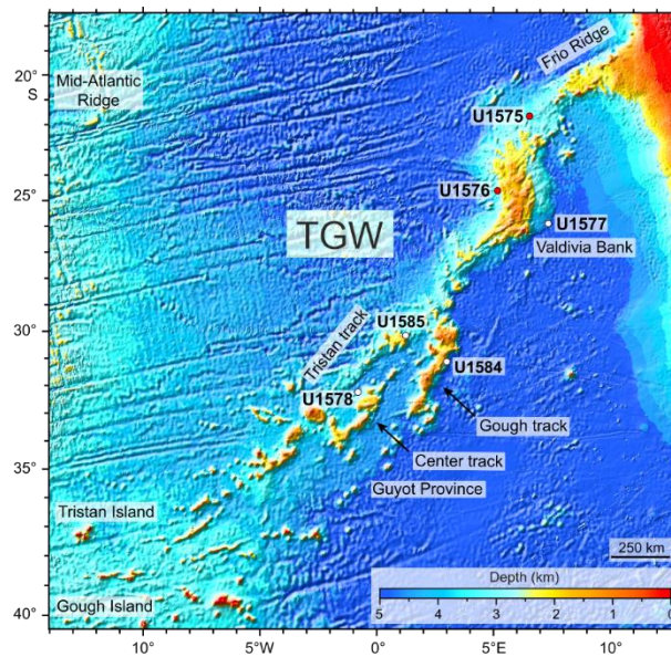
Fig. 1: Bathymetric map of the Tristan-Gough-Walvis Ridge (TGW) volcanic chain and its main seamount tracks (modified from Sager et al., 2023). Red dots=IODP sites used for this study.
