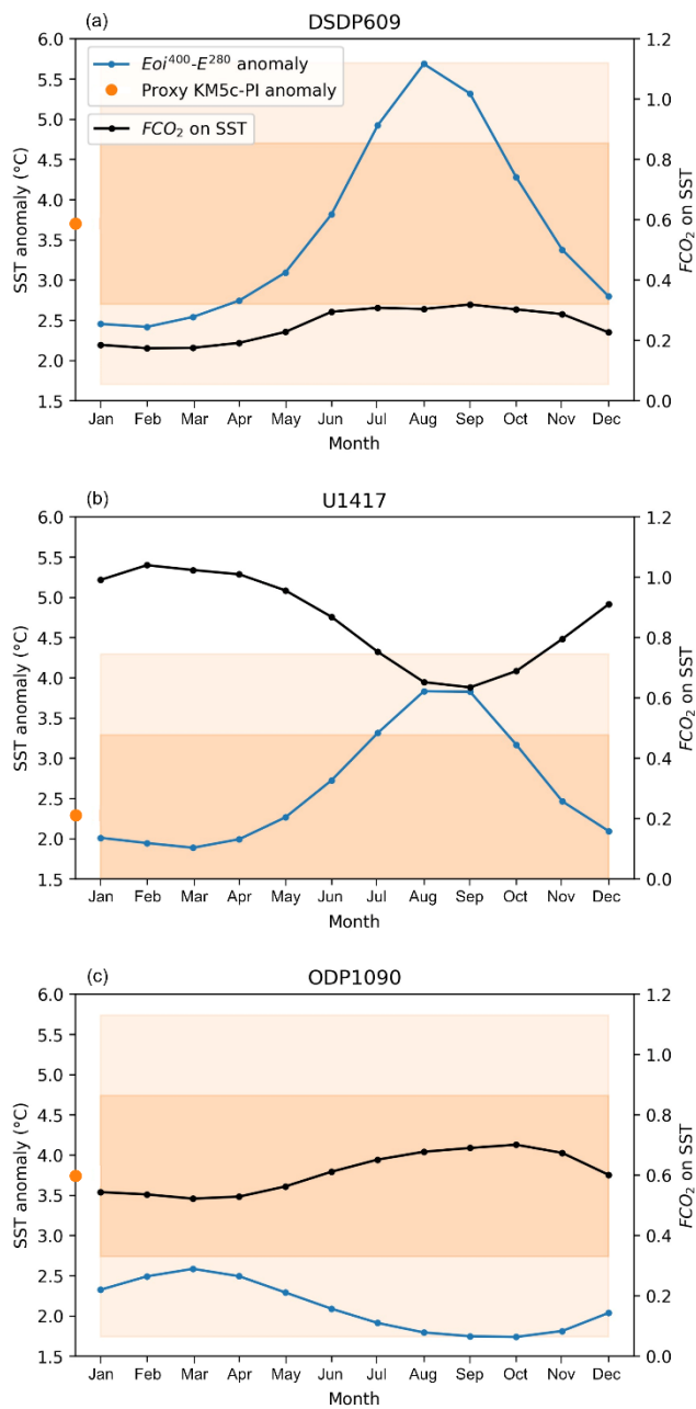
410 Figure 6: Monthly MMM Eoi^{400}-E^{280} SST anomaly (blue line) and FCO 2 on SST (black line) at sites DSDP609 (a), U1417 (b) and ODP1090 (c). The proxy data KM5c-PI anomaly value is shown by the orange circle on the y-axis, with plausible uncertainty estimates shown by orange shading (darker orange denoting \pm 1^\circ\text{C} , lighter orange denoting \pm 2^\circ\text{C} ). Note that the scale for FCO 2 on SST extends to 1.2 as some monthly values exceed 1.0 for site U1417.
