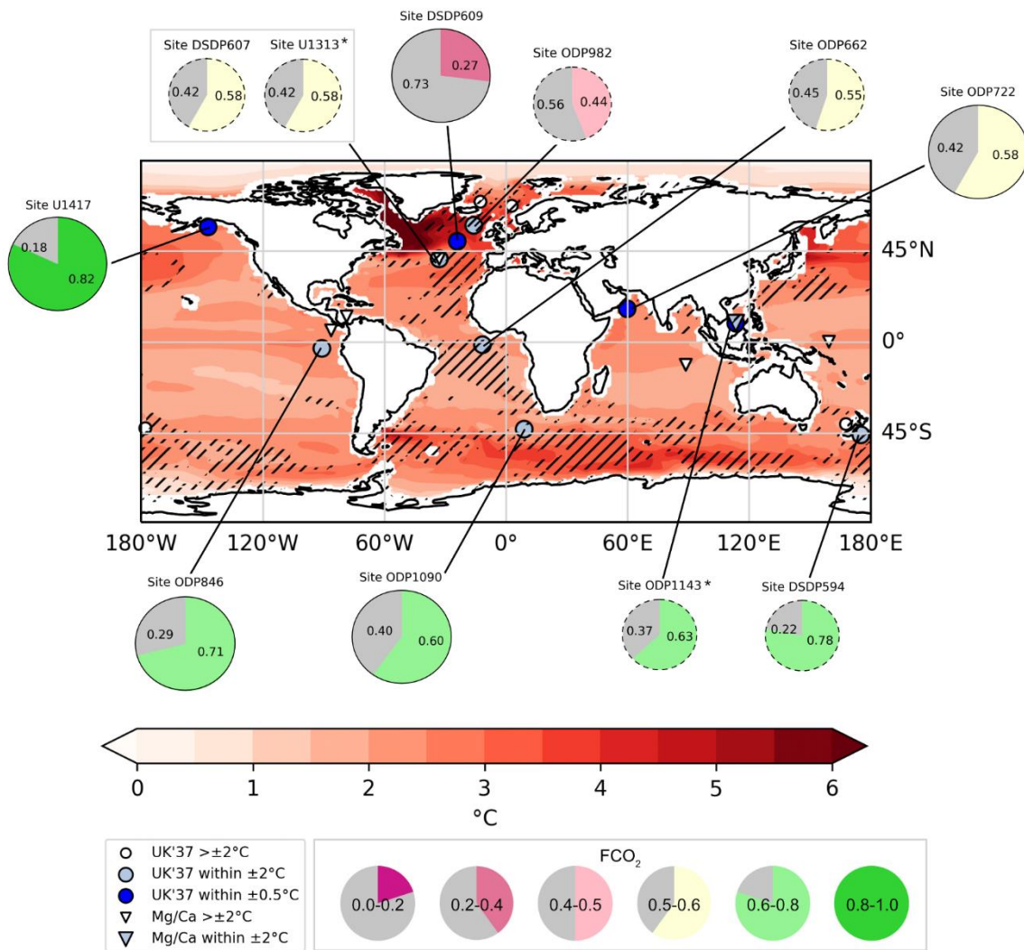
280 Figure 3: MMM Eoi 400 -E 280 SST anomaly, represented by the background red shading. The MMM is comprised from CCSM4-UoT, CESM2, COSMOS, HadCM3, MIROC4m and NorESM1-F. Hatching represents uncertainty in FCO 2 , where three or fewer of the six models agree on the dominant forcing (i.e., whether FCO 2 < 0.5 or FCO 2 > 0.5). The shape of the overlying symbols denotes the type of proxy data at each site (circle = U 37 K' , triangle = Mg/Ca); and the colour of the symbol represents the level of data-model agreement (darker = stronger agreement). All proxy data is for KM5c.
