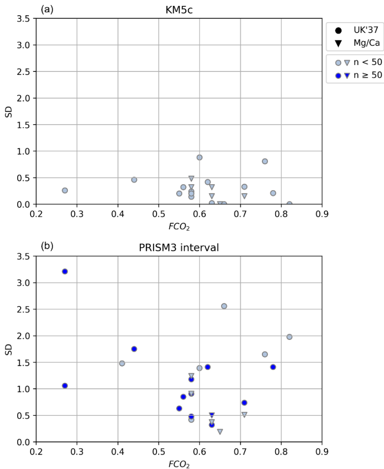
360 Figure 5: FCO 2 on SST MMM compared to standard deviation (SD) of SST proxy data for KM5c (a) and the PRISM3 interval (b). U_{37}^{Kf} data is are represented by circles and Mg/Ca data is are represented by triangles. Sites are grouped into two classes according to the number of data points available: sites with fewer than 50 data points are shown in light blue, and sites with greater than or equal to 50 data points are shown in dark blue.
