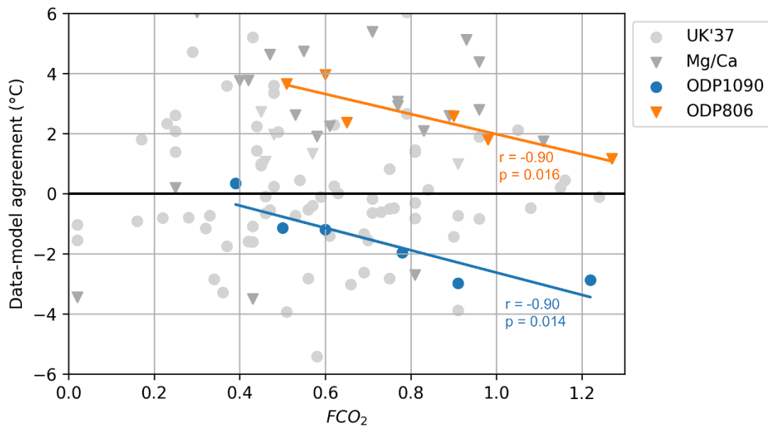
Figure 4: The relationship between individual model FCO_2 and the data-model agreement model-proxy data anomaly for all KM5c proxy sites considered here. U_{37}^{K'} data are represented by circles and Mg/Ca data are represented by triangles. Only the two sites with a significant relationship are coloured: U_{37}^{K'} site ODP1090 in blue circles and Mg/Ca site ODP806 in orange triangles. Note that the FCO_2 scale extends to 1.3 to include values from all six models. Some data points with extreme FCO_2 values lie outside of the FCO_2 range included in this figure, but the axes limits allow the significant relationships at sites ODP1090 and ODP806 to be demonstrated clearly.
