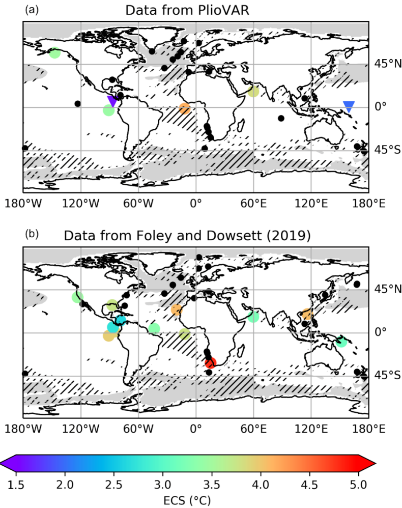
475 Figure 7: KM5c proxy-data informed ECS estimates. using Estimates are calculated using the PlioVAR data used throughout this 480 paper (a) and using FD19 as presented in Haywood et al. (2020) (b), the BAYSPLINE reconstruction in McClymont et al. (2020) and Mg/Ca reconstruction in McClymont, Ho et al. (2023) (a), and ECS estimates using FD19 presented in Haywood et al. (2020) (b). The triangles in (a) represent Mg/Ca sites, all other sites shown in (a) and (b) have U_{37}^{K'} data (large, coloured circles). The smaller black circles in represent sites that did not meet the conditions so were excluded. FCO_2 on SST is shown by the background shading: areas in white are predominantly driven by CO_2 ( FCO_2 > 0.5 ) and areas in light grey are predominantly driven by non- CO_2 forcing ( FCO_2 < 0.5 ). Hatching represents where three or fewer models agree on the dominant forcing (i.e., whether FCO_2 < 0.5 or FCO_2 > 0.5 ).
