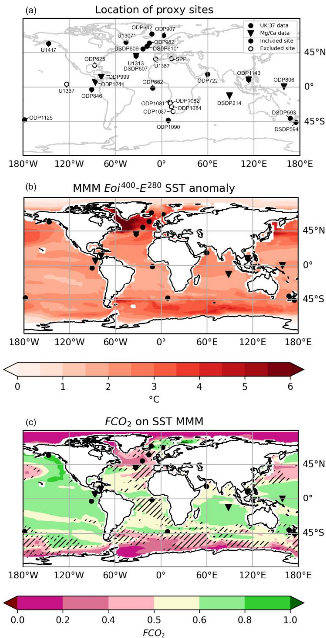
210 Figure 1: Location of PlioVAR proxy data sites (a). U_{37}^{Kf} sites are denoted by a circle, and Mg/Ca sites are denoted a triangle. Filled symbols indicate that the site is used in this paper; open symbols indicate that the site is not used, either because no model SST values are available at the site and/or because analysis had not been conducted for the PRISM3 interval as well as KM5c. Sites marked with an asterisk (*) only have data available for the PRISM3 interval (no data is available for KM5c) and are only 215 considered in the temporal variability analysis (Section 3.3). Sites included in this paper Included sites are shown again in (b) with the MMM EoI^{400}-E^{280} SST anomaly and in (c) with the FCO_2 on SST MMM. The MMM is comprised from CCSM4-UoT, CESM2, COSMOS, HadCM3, MIROC4m and NorESM1-F. Hatching in (c) denotes regions of uncertainty in FCO_2 , defined where three or fewer models agreed on the dominant forcing (i.e., whether FCO_2 < 0.5 or FCO_2 > 0.5 ).
