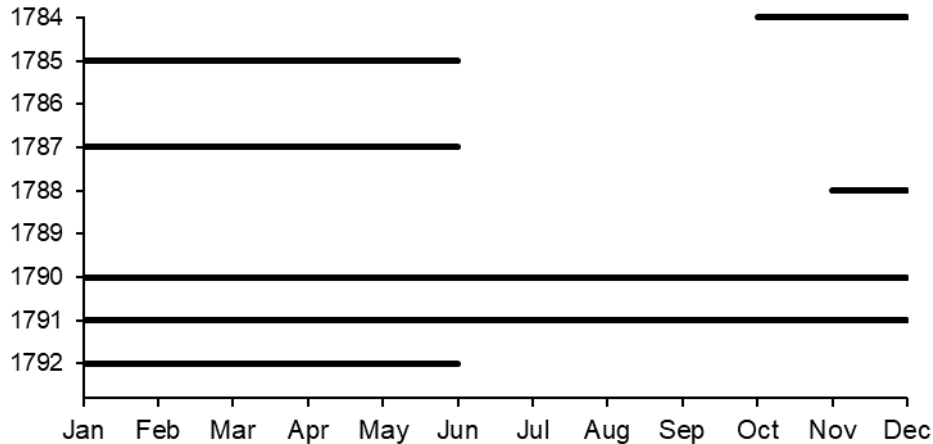
Figure 2: Coverage of air temperature data in Nuuk (orig. Godthaab), 1784–92.
