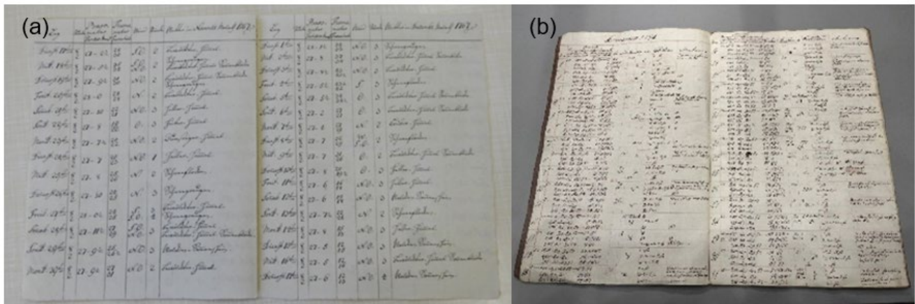
Figure 3: Examples of manuscripts presenting meteorological observations: (a) for Neu-Herrnhut (1 Sep 1767 to 22 Jul 1768), source: MH R.15 J.a.13.9. Data presented in the manuscript: 17 November to 17 December 1767, (b) for Godthaab (1782–92), source: Astronomiske og meteorologisk lagttagelser, anstillede i Godthaab i Grønland 1782–92 (Det Kgl. Bibliotek in Copenhagen). Data presented in the manuscript: January 1791.
