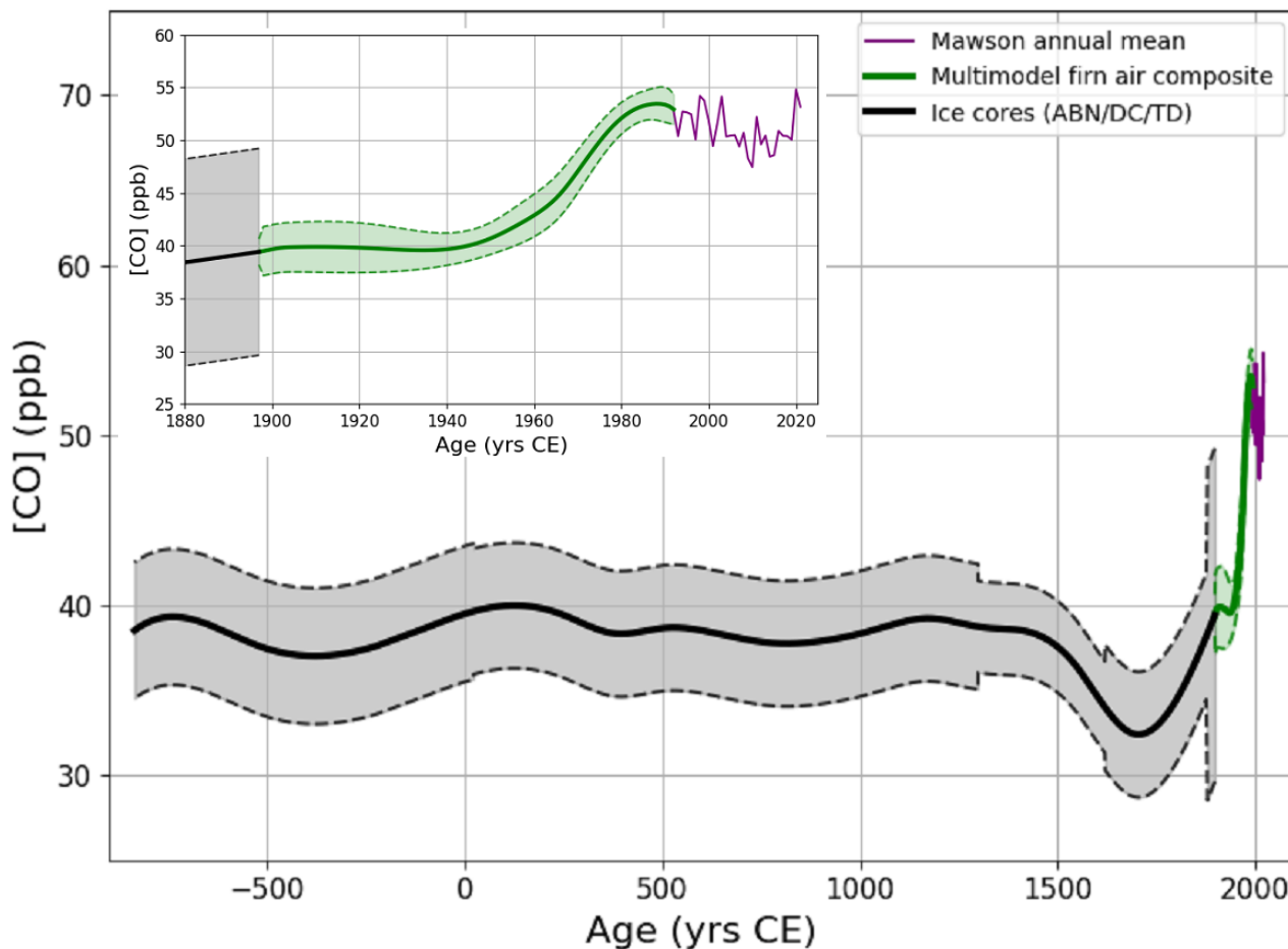
515 Figure 3. Reconstructed CO mixing ratio in the Antarctic atmosphere for the last 3000 years: a multisite ice core composite (black line) spanning -835 to 1897 CE, and the multisite firn air reconstruction from Fig. 1 (green line) spanning 1897 to 1992 CE. The envelopes represent 2\sigma uncertainties. Annual mean [CO] at Mawson Station is shown in purple, calculated from a smooth fit at daily resolution to flask sample measurements since 1992. (see text and SI Sect. 2.1). The inset shows identical data but focuses on the last 170 yrs. The three data sources forming the reconstruction each have different intrinsic smoothing.
