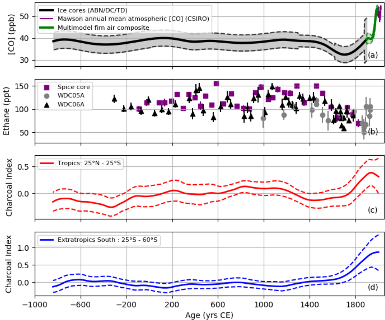
Figure 5. Antarctic Ice core and firn air CO (panel a; this study), and ethane (panel b; Nicewonger et al., 2018) records. Charcoal indexes for the intertropical 25° N-25° S latitudinal band (panel c) and the extratropical SH 25° S – 60 °S (panel d) for the last 3000 years, extracted from the Global Paleofire Database ( https://database.paleofire.org ). Charcoal indexes are average Z-scores of transformed charcoal influx per region (100 yr smoothing window/1000 yr bootstrap). Dotted-line envelopes on the charcoal indexes represent the upper and lower 95% confidence intervals from the bootstrap analysis.
