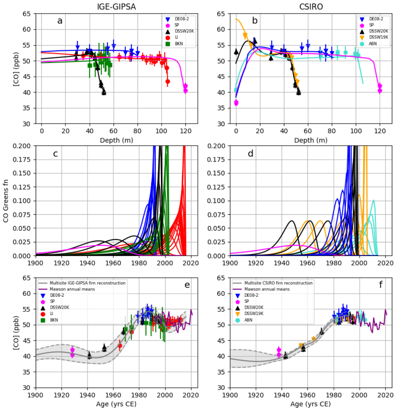
385 Figure 1. (a) and (b) Depth profiles of carbon monoxide mixing ratio in the firn air at seven Antarctic sites (Lock-In, DE08-2, DSSW20K, DSSW19K, Berkner, South Pole, ABN). Lines show forward model results using optimum atmospheric [CO] history (Sect. 3.3) as input; symbols are measurements with 2\sigma uncertainties. (a) reports IGE-GIPSA modeling results: the IGE-GIPSA model does not reconstruct the CO seasonality, and CO measurements above a depth ranging 30-40 m were excluded from the model inputs. (b) shows CSIRO modeling results. (c) and (d) show Green's functions from the IGE-GIPSA (c) and CSIRO (d) firn models
