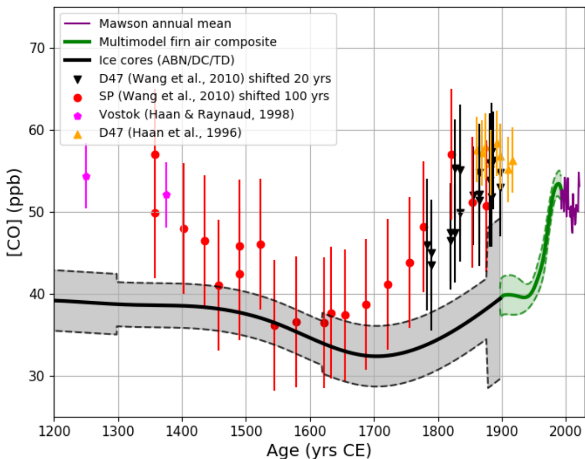
535 Figure 4. Comparison of the [CO] atmospheric reconstruction based on ABN, DC12, and TD ice core with previously published CO ice core datasets reported with 2\sigma uncertainties: South Pole (Wang et al., 2010), Vostok (Haan et al., 1998) and D47 (Haan et al., 1996; Wang et al., 2010) archives. Seven more Vostok data points are available in the time period spanning -236 to 1093 yrs CE, with [CO] ranging from 48 to 53 ppb (Haan et al., 1998).
