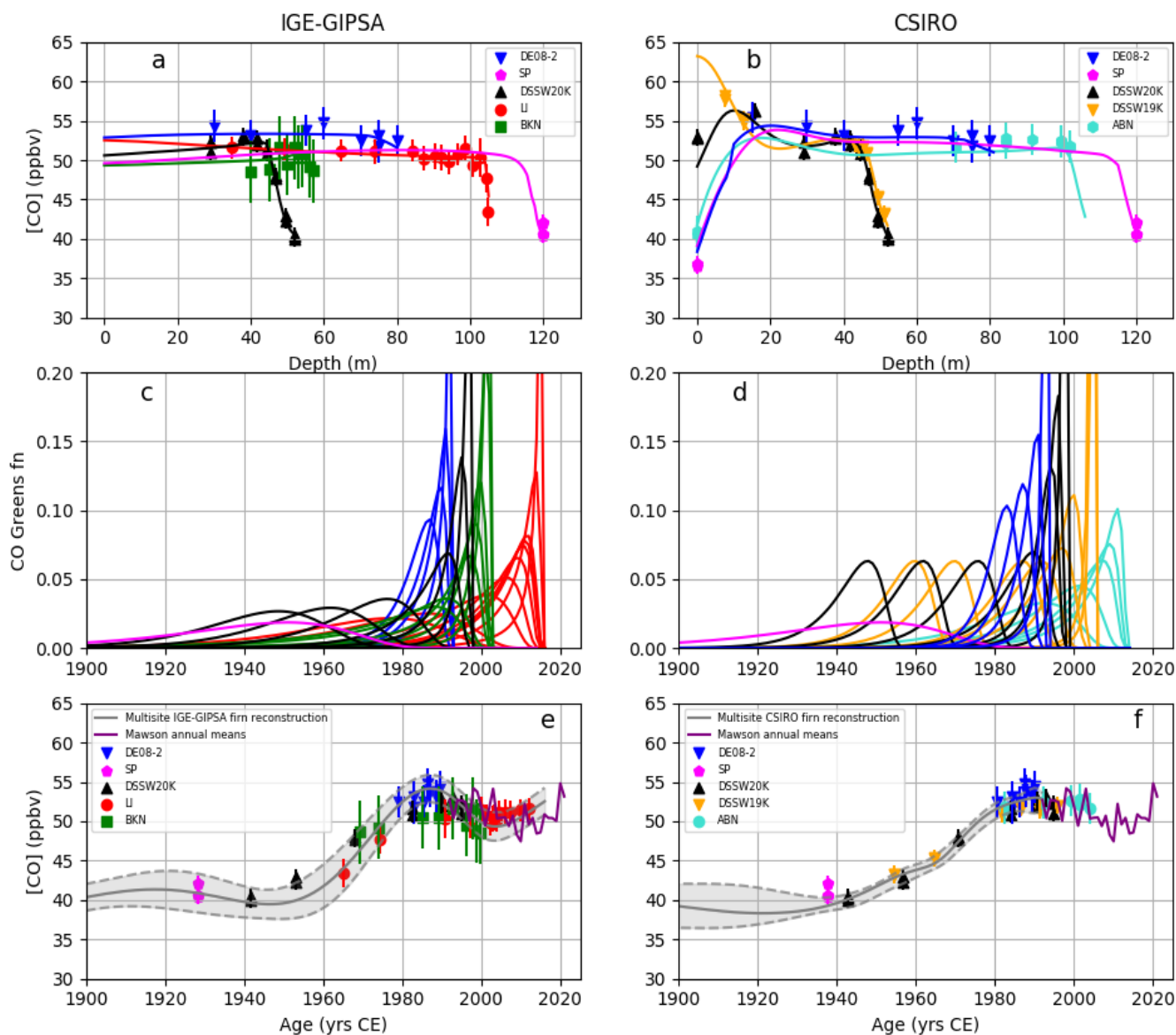
Figure 1. (a) and (b) Depth profiles of carbon monoxide mixing ratio in the firn air at seven Antarctic sites (Lock-In, DE08-2, DSSW20K, DSSW19K, Berkner, South Pole, ABN). Lines show forward model results using optimum atmospheric [CO] history (Sect. 3.3) as input; symbols are measurements with 2\sigma uncertainties. (a) reports IGE-GIPSA modeling results: the IGE-GIPSA model does not reconstruct the CO seasonality, and CO measurements above a depth ranging 30-40 m were excluded from the model inputs. (b) shows CSIRO modeling results. (c) and (d) show Green's functions from the IGE-GIPSA (c) and CSIRO (d) firn models (there is one line for each firn sampling depth, with the colors corresponding to those for different sites in panels (a) and (b)). (e) and (f) Best-fit atmospheric history of Antarctic [CO] obtained with the inverse modeling IGE-GIPSA (e) and CSIRO (f) technique (gray line, with the envelope representing 2\sigma uncertainty). Firn air measurements (symbols) are plotted as a function of mean ages extracted from the modeled age distributions (excluding the upper firn measurements strongly affected by seasonality). We note that firn air data plotted versus mean age are not strictly comparable with the modeled time trends which account for the age distribution widths in the samples. Annual mean [CO] at Mawson Station is shown in purple - the annual means are calculated from a smooth fit at daily resolution to measurements conducted by CSIRO since 1992 on flask samples of background air collected fortnightly (SI Sect. 2.1).
