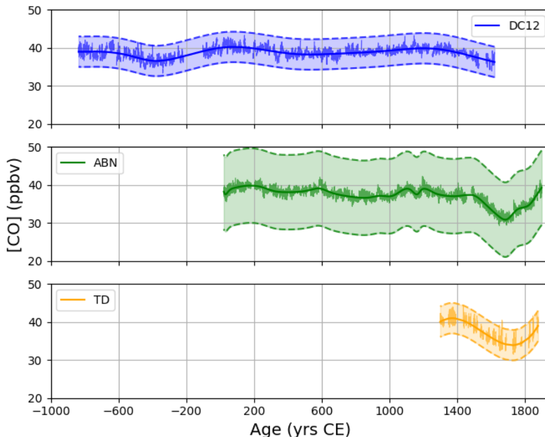
455 Figure 2. Continuous [CO] records collected along the DC12 (blue), ABN (green), and TD (orange) Antarctic ice cores. The integration time of high resolution datasets is 10 s. A spline is applied to each high resolution dataset. The noise displayed by high resolution solid lines only represents the internal precision, while the envelopes report 2\sigma uncertainties combining uncertainties on CO blanks, solubility calibration factors, and external precision of CO CFA measurements derived from the reproducibility measurements.
