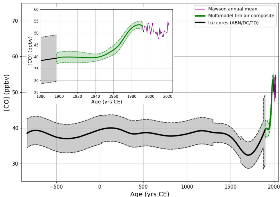
515 Figure 3. Reconstructed CO mixing ratio in the Antarctic atmosphere for the last 3000 years: a multisite ice core composite (black line) spanning -835 to 1897 CE, and the multisite firn air reconstruction from Fig. 1 (green line) spanning 1897 to 1992 CE. The envelopes represent 2\sigma uncertainties. Annual mean [CO] at Mawson Station is shown in purple, calculated from a smooth fit at daily resolution to flask sample measurements since 1992. (see text and SI Sect. 2.1). The inset focuses on the last 170 yrs. The three data sources forming the reconstruction each have different intrinsic smoothing.
