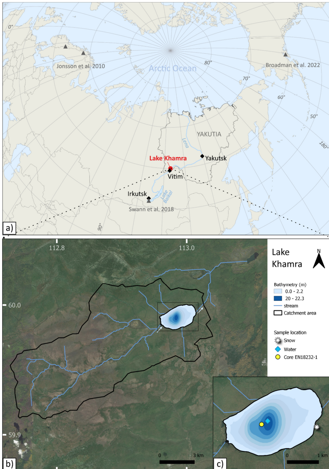
Figure 1. Study area. a) Position of Lake Khamra in the south-western part of Yakutia, close to the Lena river; closest weather station is located in Vitim, Lake Khamra lies in between the cities Yakutsk and Irkutsk. Other high-resolution study sites are indicated as grey triangles (Jonsson et al., 2010; Swann et al., 2018; Broadman et al., 2022). b) Catchment of Lake Khamra, main in- and outflow are indicated by arrows. c) Sample locations at Lake Khamra. (Service layer credits: © OpenStreetMap contributors 2023. Distributed under the Open Data Commons Open Database License (ODbL) v1.0.; Esri, Maxar, Earthstar Geographics, and the GIS User Community).
