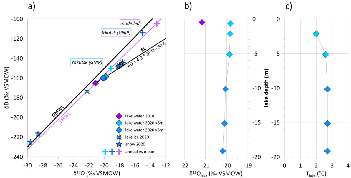
275 Figure 3. a) Co-Isotope plot ( \delta^{18}\text{O} - \delta\text{D} ) of lake water, ice and snow samples taken during the two field campaigns in August 2018 and March 2020, in relation to the GMWL (Craig, 1961) and the LMWL according to the modelled monthly mean values. Annual weighted mean values of precipitation modelled for the region (Bowen and Revenaugh, 2003; Bowen et al., 2005; Bowen, 2023; IAEA/WMO, 2023) and from the GNIP stations in Yakutsk and Irkutsk (IAEA/WMO, 2023) are marked as crosses. The intercept point of the local evaporation line (EL) and modelled LMWL is at \delta^{18}\text{O} -20.9‰ and \delta\text{D} -164.0‰. b) \delta^{18}\text{O} of a water-depth profile of Lake Khamra, sampled below lake ice in March 2020 c) T_{\text{lake}} of the water-depth profile, taken below ice cover in March 2020. 280
