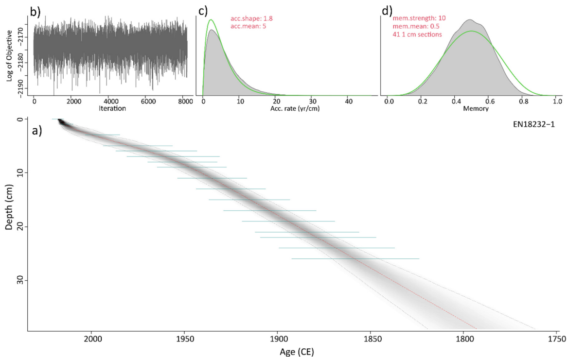
340 Figure 4. a) Bayesian accumulation model applying R package ‘rbacon’ (Blaauw and Christen, 2011) based on the ^{210}\text{Pb} and ^{137}\text{Cs} dating (green lines) of the short core EN18232-1 (grey lines= 2\sigma range; red line=median). b) Model iteration log. c, d) Prior (green line) and posterior (grey area) distributions for accumulation rate and memory, respectively.
