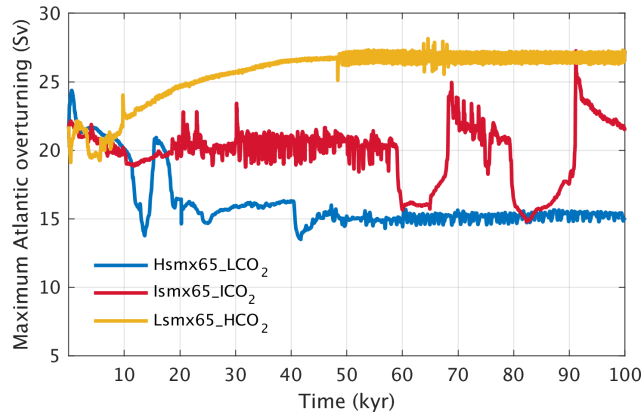
Figure 5. Maximum Atlantic Overturning (Sv) temporal evolution at the critical combination of smx65 and \text{CO}_2 for triggering glacial inception (threshold 15 msle level), for three selected experiments (see Table 1).
