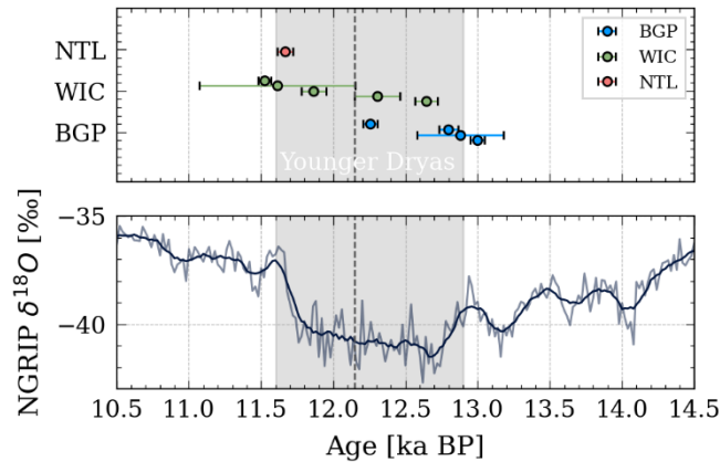
Fig. 2: Formation ages of CCCs in comparison to other proxy records the Greenland ice-core record. Upper panel: CCC formation ages from the studied cave sites. Error bars refer to the 2\sigma error of the respective isochron. Grey shaded area represents the defined limits of the Younger Dryas period. Caves are sorted by latitude (north is top) along the vertical axis and the position of individual data points is offset arbitrarily for better visibility. Lower panel: \delta^{18}\text{O} in Greenland precipitation from the NGRIP ice-core record (Rasmussen et al., 2014). The smoothed line represents a 100-year moving average. The dashed vertical line indicates the mid-Younger Dryas transition (12.15 ka BP).
