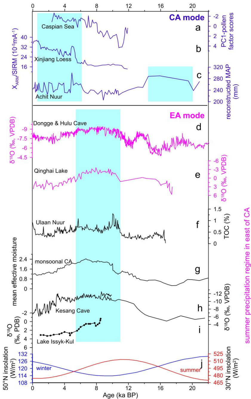
91 92 Figure 5. A comparison of proxy variability recorded in EA and CA. a Pollen record from the Caspian Sea (Leroy et al., 2014); b 93 X_{ARM}/SIRM in the LJW10 section of the Xinjiang Loess (Chen et al., 2016); c Reconstructed MAP (mean annual precipitation) from Achit 94 Nuur (Sun et al., 2013); d speleothem \delta^{18}O values records from Dongge Cave and Hulu Cave (Yuan et al., 2004; Wang et al., 2001); e \delta^{18}O 95 of ostracode shells from Qinghai Lake (Liu et al., 2007); f TOC (Total organic carbon) from Ulaan Nuur (Lee et al., 2013); g Mean 96 effective moisture from monsoonal Central Asia (Herzschuh, 2006); h \delta^{18}O from Kesang Cave (Cheng et al., 2016); i \delta^{18}O from Lake 97 Issyk-Kul (Ricketts et al., 2001); j Summer (red line) insolation at 30^{\circ}N and winter (blue line) insolation at 50^{\circ}N (Berger, 1978). Blue 98 shadows indicate the wet period of paleoclimate proxies.
