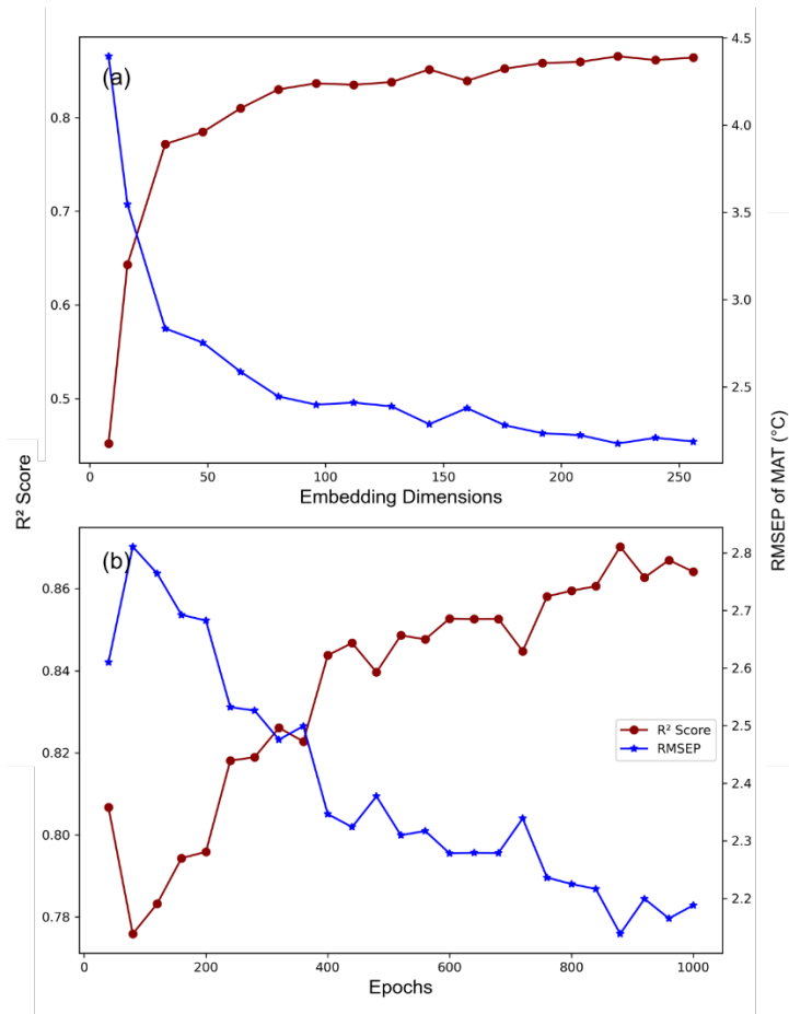
470 Figure A2: MEMLMe prediction performance under different GloVe hyper-parameter settings. a) Fix epoch = 1,000, set embedding dimensions from 8 to 256; b) Fix embedding dimensions = 256, set epoch from 40 to 1,000. The model is developed from the NIMBIOS set and trained on mean annual temperature (MAT).
