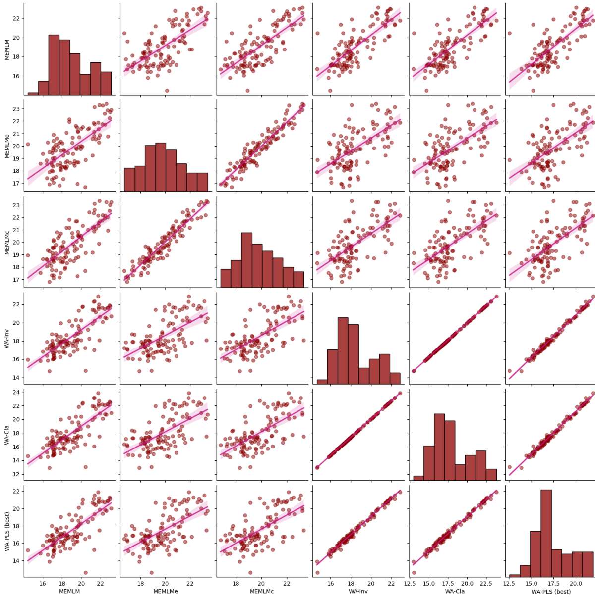
480 Figure A5: Inter-regression of MAT reconstructions for six different models for the Consuelo core.
