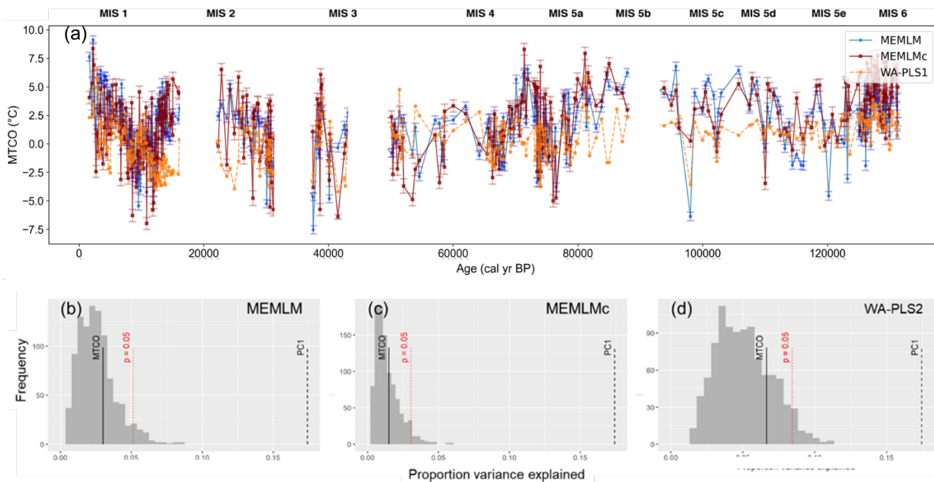
Figure 6: a) MTCO reconstruction for the Villarquemado core. b, c & d) statistical significance of MEMLM, MEMLMc, and WA-PLS2 reconstructions, respectively. MEMLM uncertainties are calculated using IBM UQ360 (section 2.3.3). These compare with cross-validated RMSEP errors of 2.353 (MEMLM), 2.434 (MEMLMc), and 2.923 (WA-PLS2) °C.
