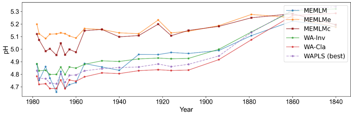
Figure A8: pH reconstructions based on six models for the Round Loch of Glenhead (RLGH) core.
