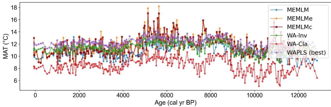
495 Figure A11: Mean annual temperature (MAT) reconstruction based on six models for the Llaviucu core.
