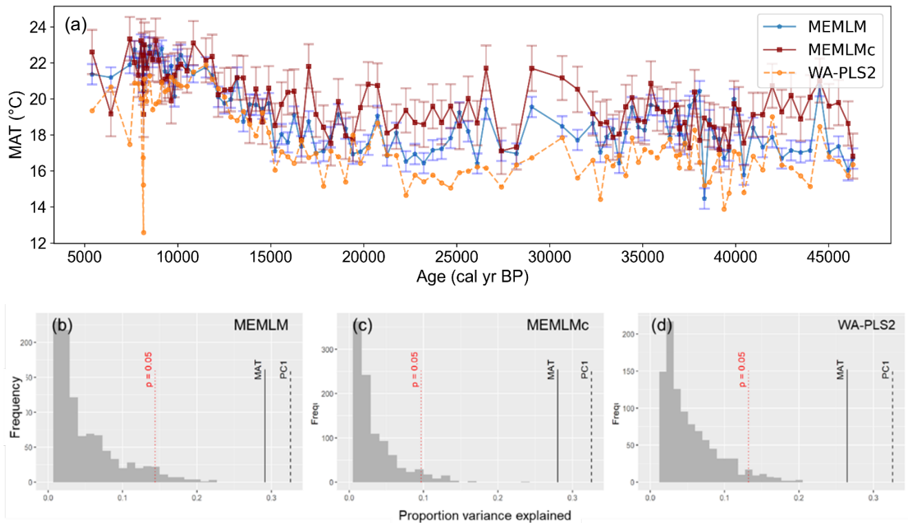
345 Figure 4: a) MAT reconstruction for the Consuelo core. b, c & d) statistical significance of MEMLM, MEMLMc, and WA.PLS2 reconstructions, respectively. MEMLM uncertainties are calculated using IBM UQ360 (section 2.3.3). These compare with cross-validated RMSEP errors of 2.254 (MEMLM), 2.094 (MEMLMc), and 4.979 (WA-PLS2) °C.
