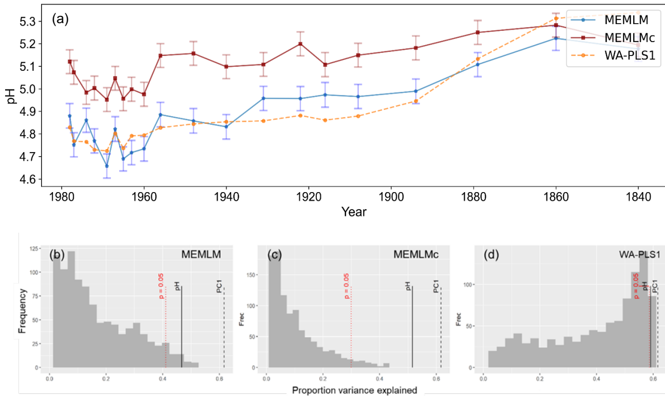
320 Figure 2: a) pH reconstruction for the RLGH core. b, c & d) statistical significance of MEMLM, MEMLMc, and WA-PLS1 reconstructions, respectively. MEMLM uncertainties are calculated using IBM UQ360 (section 2.3.3). These compare with cross-validated RMSEP errors of 0.292 (MEMLM), 0.294 (MEMLMc), and 0.308 (WA-PLS1) pH units.
