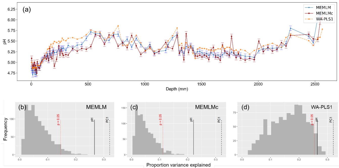
Figure 3: a) pH reconstruction for the RLGH3 core. b, c & d) statistical significance of MEMLM, MEMLMc, and WA-PLS1 reconstructions, respectively. MEMLM uncertainties are calculated using IBM UQ360 (section 2.3.3). These compare with cross-validated RMSEP errors of 0.292 (MEMLM), 0.294 (MEMLMc), and 0.308 (WA-PLS1) pH units.
