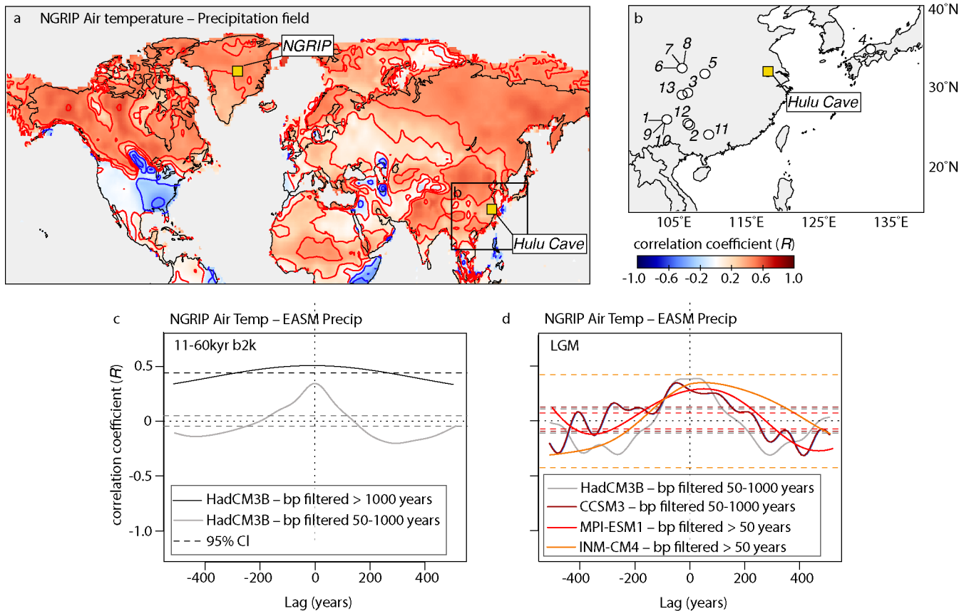
785 Figure 1. a. Instantaneous (lag 0) spatial correlation between mean decadal surface air temperature at the NGRIP site and mean decadal land surface temperatures during the last glacial period (11-60 kyr b2k) as simulated with the HadCM3B-M2.1 coupled general circulation model (Armstrong et al., 2019). The simulation incorporates Dansgaard-Oeschger cycles, Heinrich Events, and shorter-term variability, with a spatial climate fingerprint derived from a Last Glacial Maximum (LGM) freshwater hosing experiment applied over the North Atlantic Ocean. The location of NGRIP, the East Asian summer monsoon (EASM) region and Hulu Cave are also shown. b. EASM domain showing the location of speleothem records compiled by Corrick et al. (2020) and used in this study. Numbering: 1. Dashibao; 2. Dongge; 3. Furong; 790 4. Maboroshi; 5. Sanbao; 6. Shizi; 7. Songjia1; 8. Songjia3; 9. Wulu3; 10. Wulu32; 11. Xiaobailong; 12. Yamen; 13. Yangkou. Reference to the cave site is provided in Corrick et al. (2020). c. Cross-correlation between simulated NGRIP air temperature and EASM precipitation between 11 and 60 kyr ago. The EASM region is defined here as the average of 10-40°N and 95-125°E. The timeseries were bandpass filtered to quantify leads and lags at millennial and shorter timescales, respectively. d. Same as (c) but for the LGM using transient climate model simulations (Armstrong et al., 2019; Liu et al., 2009) and equilibrium experiments from CMIP6 (Kageyama et al., 2021). Results from 795 HadCM3B and CCSM3 span the interval ~17.5-21kyr b2k, whereas for CMIP6 only simulations longer than 200 years were considered for the cross-correlation analysis. Dashed lines reflect the 95% significance level against first order autoregressive (AR1) noise.
