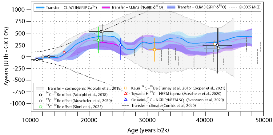
840 Figure 7. Posterior timescale transfer function based on the MCMC synchronizations presented in this study. Positive values indicate that the U-Th timescale is older than GICC05. The transfer function is presented with its median (thick lines) and pointwise 95% credible intervals (shading). The results are compared to the transfer function presented in Adolphi et al. (2018) (grey shading), which is based on a compilation of U-Th-dated ^{14}\text{C} records, including the low-resolution and less precisely dated Hulu Cave data (Southon et al., 2012). The markers with error bars ( \pm 2\sigma ) show discrete match points inferred from comparison of ice-core ^{10}\text{Be} records and absolutely dated ^{14}\text{C} data (Adolphi et al., 2018; Cooper et al., 2021; Muscheler et al., 2020; Sinnl et al., 2023; Turney et al., 2016), ^{14}\text{C} -dated volcanic eruptions identified in Greenland ice cores (Muscheler et al., 2020; Svensson et al., 2020), and climate tie points (Corrick et al., 2020). The dashed lines highlight the maximum 845 counting uncertainty of GICC05.
