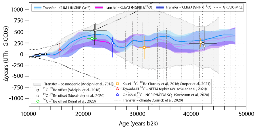
Figure 7. Posterior timescale transfer function based on the MCMC synchronizations presented in this study . Positive values indicate that the U-Th timescale is older than GICC05. The transfer function is presented with its median (thick lines) and pointwise 95% credible intervals (shading). The results are compared to the transfer function presented in Adolphi et al. (2018) ( grey shading ), which is based on a compilation of U-Th-dated ^{14}\text{C} records, including the low-resolution and less precisely dated Hulu Cave data (Southon et al., 2012). The markers with error bars ( \pm 2\sigma ) show discrete match points inferred from comparison of ice-core ^{10}\text{Be} records and absolutely dated ^{14}\text{C} data (Adolphi et al., 2018; Cooper et al., 2021; Muscheler et al., 2020; Sinnl et al., 2023; Turney et al., 2016), ^{14}\text{C} -dated volcanic eruptions identified in Greenland ice cores (Muscheler et al., 2020; Svensson et al., 2020), and climate tie points (Corrick et al., 2020) . The dashed lines highlight the maximum counting uncertainty of GICC05.
