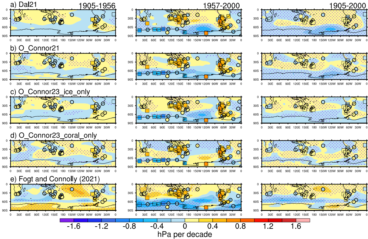
Figure 13. Linear near-surface annual mean pressure trends (hPa per decade) for 1905-1956 (left column), 1957-2000 (middle column), and 1905-2000 (right column) for various datasets in each row a) Dalaiden et al. (2021); b) O'Connor et al. (2021) proxy reconstruction c) O'Connor et al. (2023) reconstruction with only ice core proxies; d) O'Connor et al. (2023) reconstruction with only coral proxies; e) Fogt and Connolly (2021) station-based reconstruction. Trends from observation data, where available, are plotted using the same color scale on top of the gridded pressure trends. Stippling indicates gridded pressure trends significantly different from zero at p < 0.05 , boxes indicate trends in observations significantly different from zero at p < 0.05
