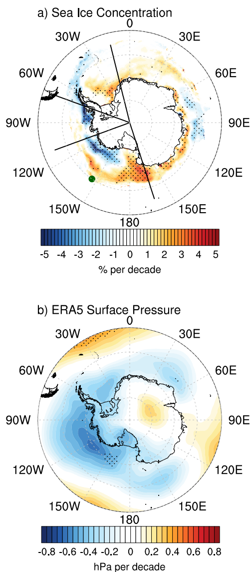
Figure 1. a) Annual mean sea ice concentration trends (% per decade) over 1979–2020. The solid black lines denote the sea ice sector boundaries Raphael and Hobbs (2014). The dark green dot marks the location of the ice edge approximated by the Thomas and Abram (2016) reconstruction. b) Annual mean ERA5 surface pressure trends (hPa per decade). In both plots, trends statistically different from zero at p < 0.05 are stippled.
