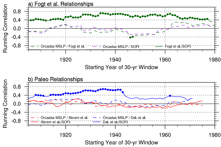
Figure 9. 30-year running correlations between pairs of the South Orkney Fast Ice (SOFI) duration from Murphy et al. (1995, 2014), various sea ice extent estimates, or Orcadas station mean sea level pressure. Correlations significantly different from zero at p < 0.05 are marked with a circle.
