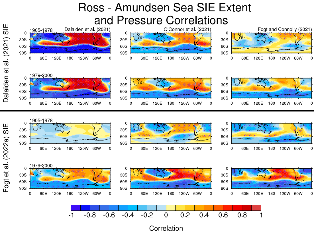
Figure 8. As in Fig. 7, but for the sea ice extent reconstructions for the Ross-Amundsen Seas sector.
