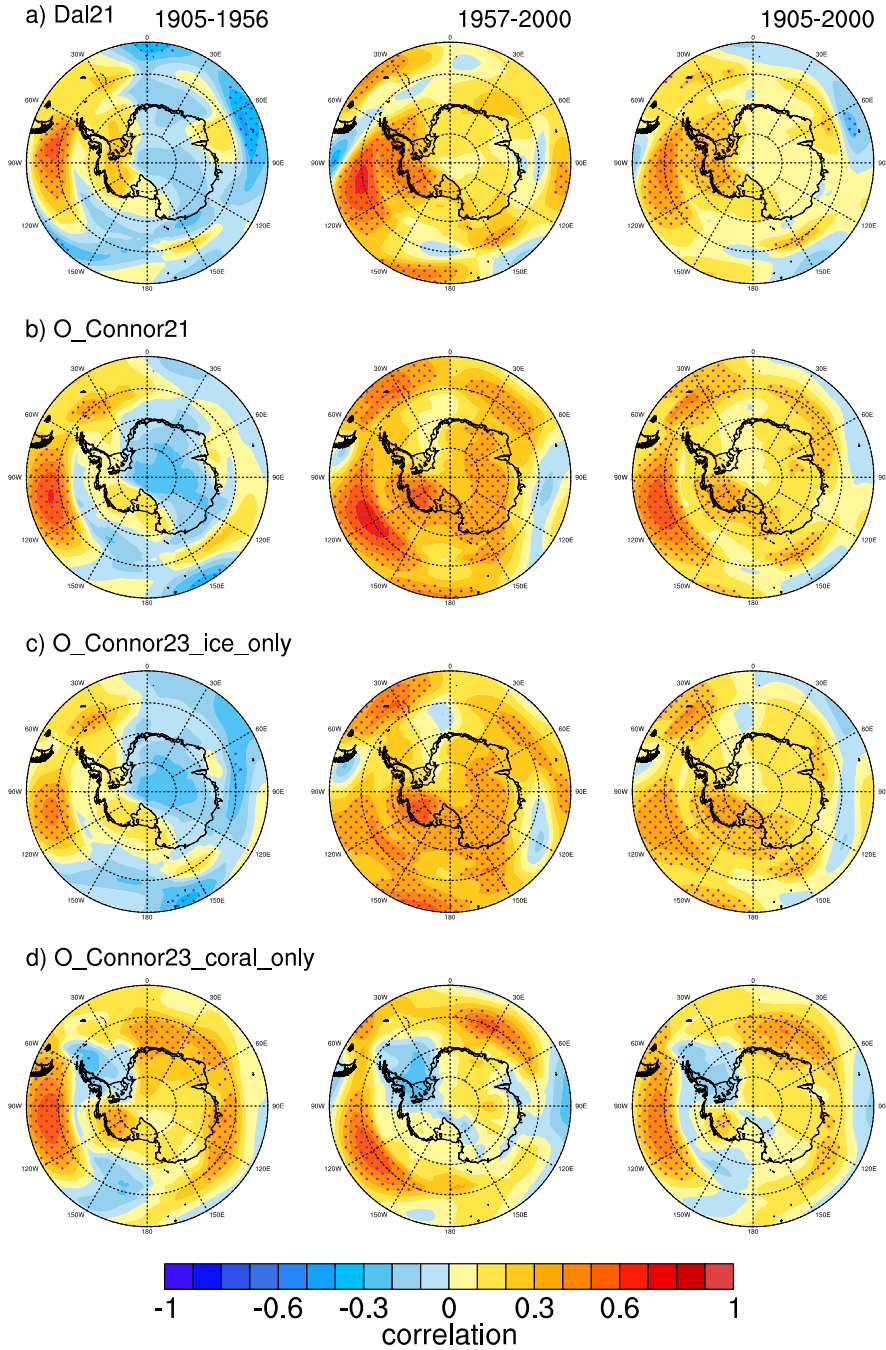
Figure 10. Correlations of annual mean pressure at each grid point between the various paleo-based reconstructions with the Fogt and Connolly (2021) reconstruction. a) Dalaiden et al. (2021); b) O'Connor et al. (2021); c) O'Connor et al. (2023) ice core-based proxies only; d) O'Connor et al. (2023) coral-based proxies only. The columns denote three time periods: 1905-1956 (left column, prior to Antarctic data), 1957-2000 (middle column), and the full period of overlap 1905-2000 (right column). Correlations statistically different from zero at p < 0.05 are stippled. All datasets were linearly detrended over the specific time period prior to calculating the correlations; further details on each dataset is provided in Table 1 and the proxy locations are given in Fig. 2.
