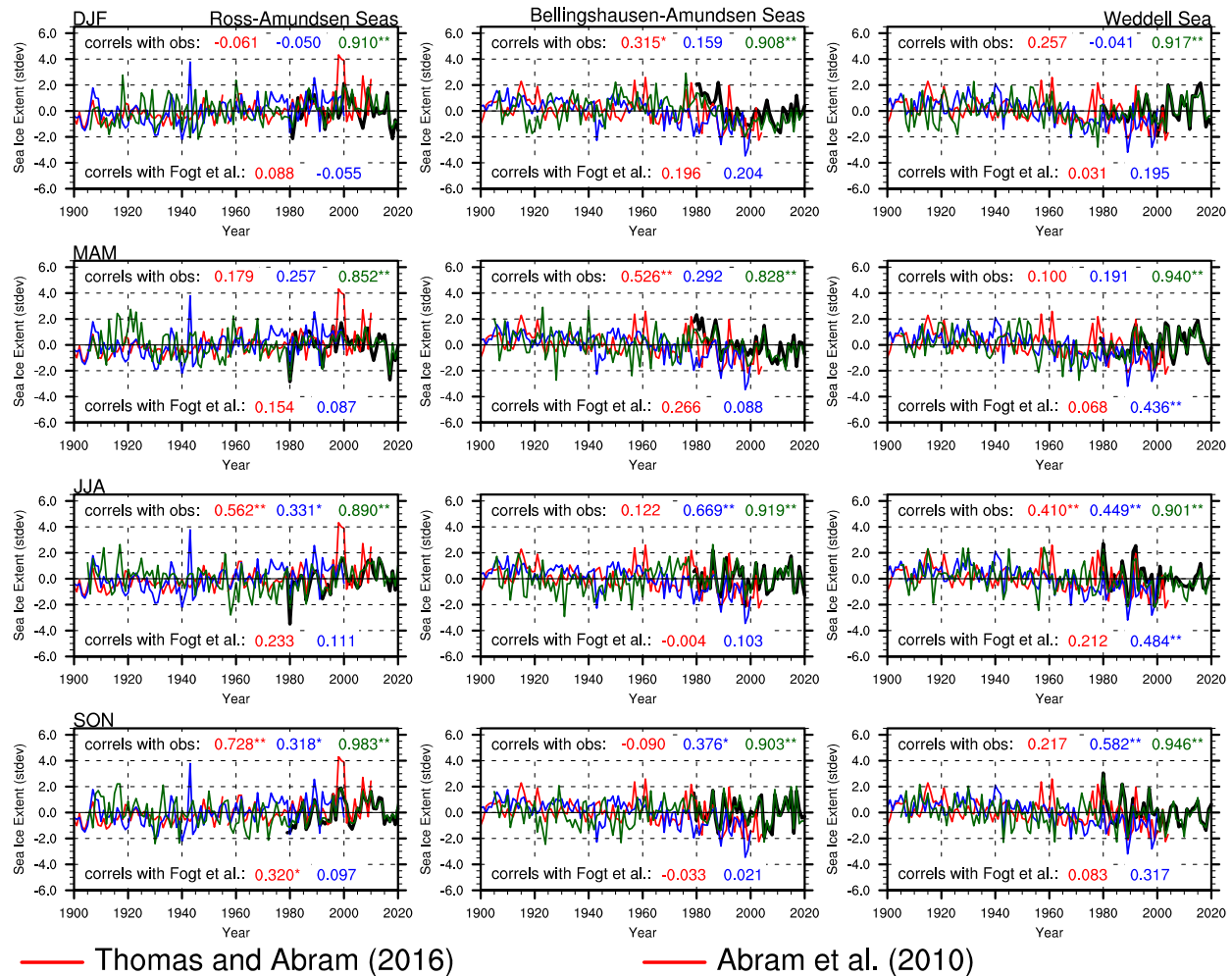
Figure 4. As in Fig. 3, but with the seasonal mean observations and reconstructions of Fogt et al. (2022a) with the annual mean paleo-based reconstructions. The Thomas and Abram (2016) paleo-based reconstruction is used for the Ross-Amundsen sector (left column), while the Abram et al. (2010) reconstruction is used for the other two sectors (middle and right columns). The correlations are color coded following the legend. Correlations with observations are given at the top of each panel, and correlations with seasonally-varying Fogt et al. (2022a) reconstructions are given at the bottom of each panel.
