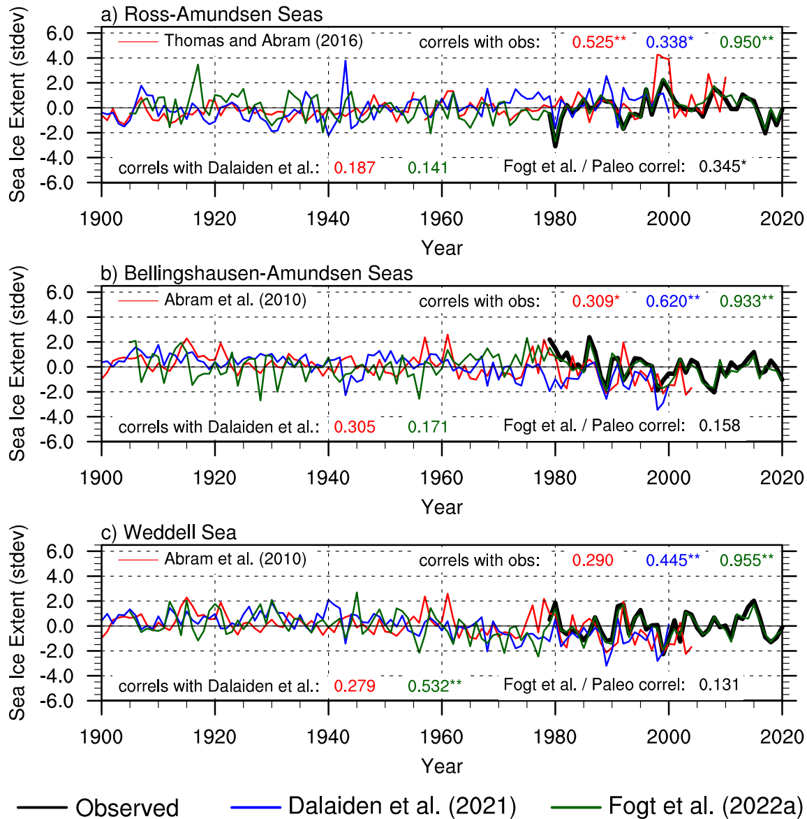
Figure 3. Annual mean sea ice extent timeseries from various reconstructions approximately related to the Raphael and Hobbs (2014) sea ice boundaries in Fig. 1 for the a) Ross-Amundsen Seas; b) Bellingshausen-Amundsen Seas; c) Weddell Sea; paleo-based reconstructions are given in red and labeled separately for each panel. The correlations with satellite observations (in black) during the period of overlap are given in the top of each panel, with the colors denoting the individual timeseries as given in the legend. At the bottom, correlations with the Dalaiden et al. (2021) and Fogt et al. (2022a) reconstructions are similarly provided. In each case, after adjusting the sample size by the lag1 correlation as needed, correlations significantly different from zero at p < 0.05 and p < 0.01 are marked with * and **, respectively.
