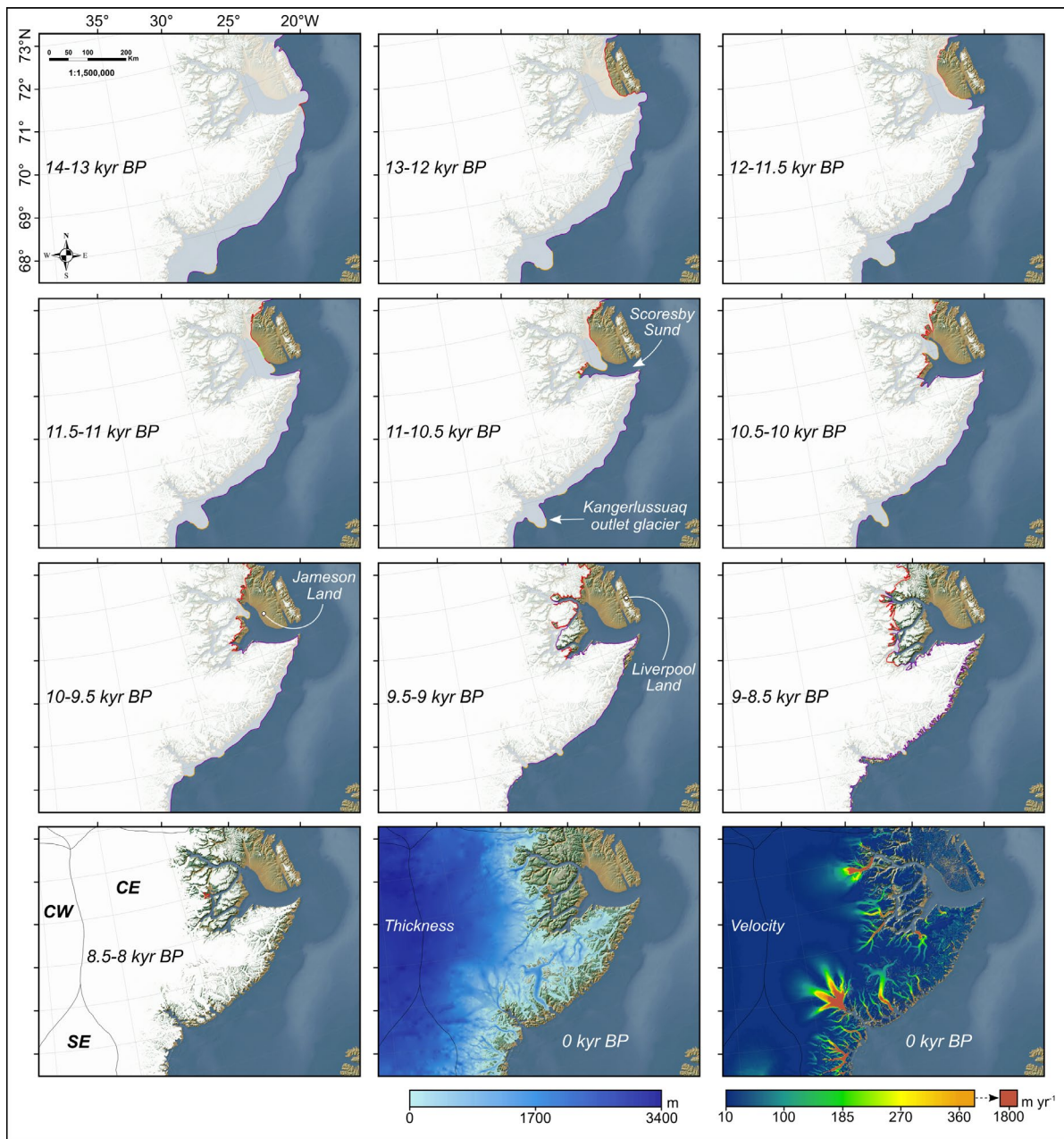
Figure 10. Time slice maps of the PaleoGrIS 1.0 isochrone reconstruction in the Scoresby Sund and Kangerlussuaq region. The reconstructed ice sheet areal extent for each given time slice is displayed in each sub-panel as a white transparent polygon, while the underlying opaque white layer is the present-day ice cover from BedMachine v4. The reconstructed ice sheet margins are highlighted by our isochrone polylines, which feature different colour schemes (see Fig. 8 for key) relating to our four isochrone confidence levels (see section 2.3.5). Bottom panels also feature present-day ice-sheet thickness (Morlighem et al., 2017) and surface velocity data (Joughin et al., 2018). Topography and bathymetry are from the GEBCO 2022 release. For a more complete figure legend, the reader is advised to consult Figure 8.
