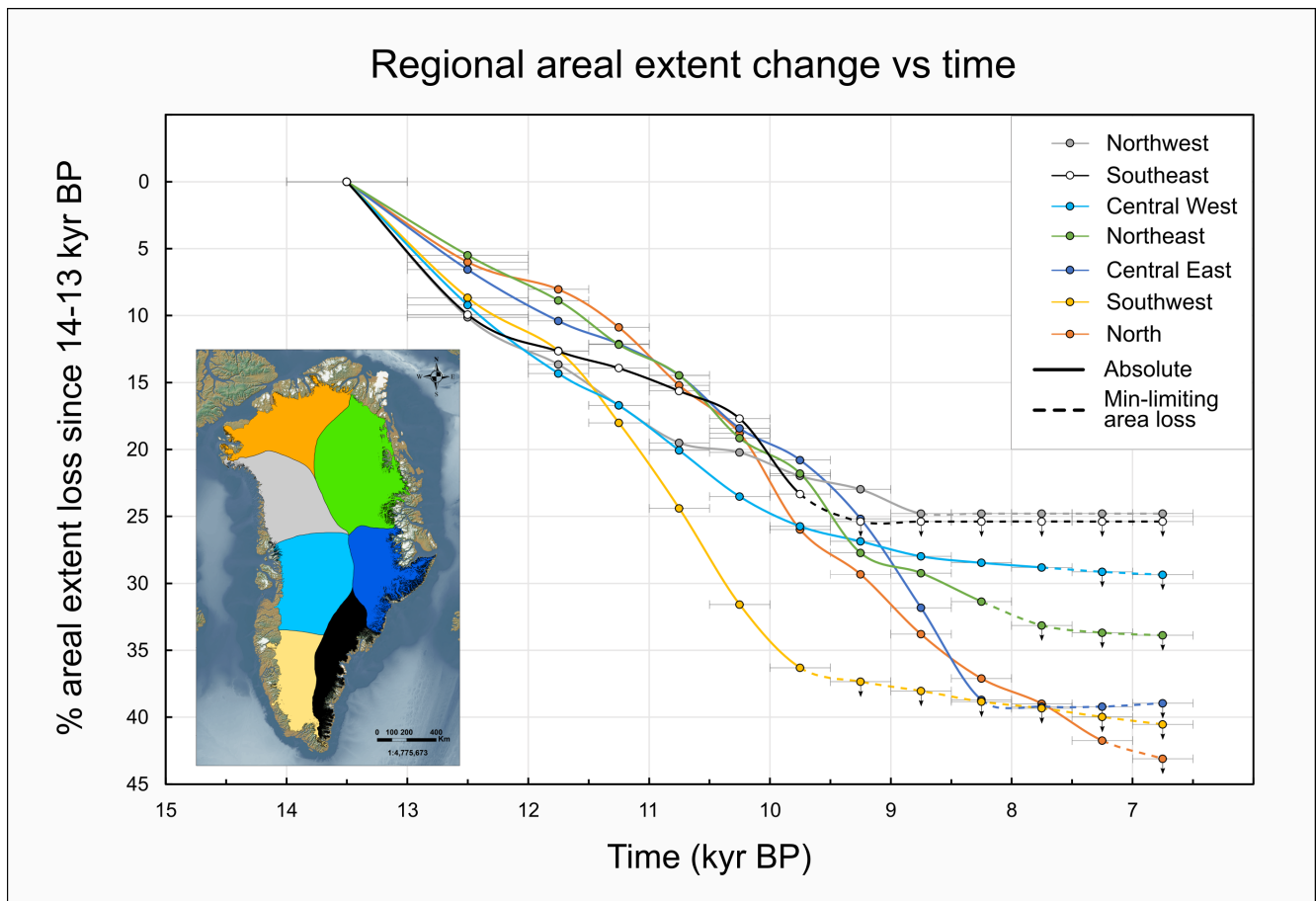
Figure 17. The PaleoGrIS 1.0 reconstruction of percentage ice-sheet areal extent loss between ~14 kyr BP (0%) and ~6.5 kyr BP, for each of the seven ice sheet regions spatially divided as displayed in inset map, after Rignot & Mouginot (2012). The colour code of individual time series matches the inset map polygons. Importantly, we use a different symbol to highlight whether the percentage areal extent loss, for a given region, is an absolute areal extent estimate (straight line), or a minimum-limiting areal extent loss estimate (dashed line with downward pointing arrows). The switch from straight to dashed lines thus represents, for each region, the youngest isochrone to feature a more-extensive-than-present ice-sheet extent along the full region-specific ice margin.
