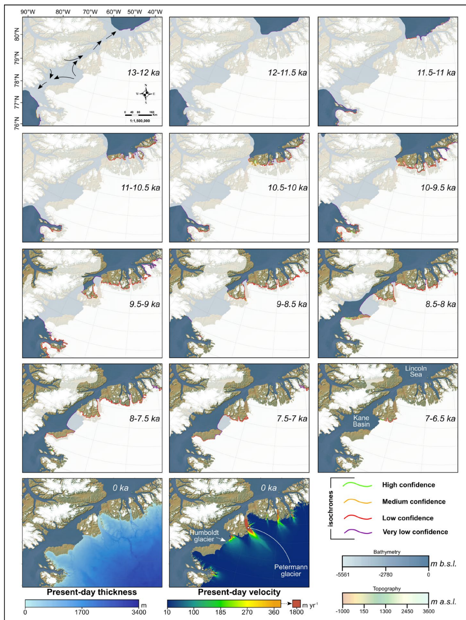
1175 Figure 8. Time slice maps of the PaleoGrIS 1.0 isochrone reconstruction in Nares strait region. The reconstructed ice sheet areal extent for each given time slice is displayed in each sub-panel as a white transparent polygon, while the underlying opaque white layer is the present-day ice cover from BedMachine v4. The reconstructed ice sheet margins are highlighted by our isochrone polylines, which feature different colour schemes relating to our four isochrone confidence levels (see section 2.3.5). We merge our isochrones with the reconstruction of former ice extent over Ellesmere Island (Innuitian Ice Sheet) from Dalton et al. (2020). While 1180 no modifications were applied to the margin extent of that dataset, the timing of Dalton et al. (2020) isochrones was in some cases modified (by less than 1 kyr at most) to match our reconstruction. Bottom panels also feature present-day ice-sheet thickness (Morlighem et al., 2017) and surface velocity data (Joughin et al., 2018). Topography and bathymetry are from the GEBCO 2022 release.
