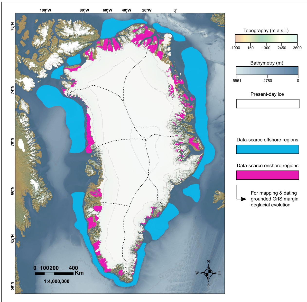
2150 Figure 20. Map of offshore and onshore regions that we interpret as data-scarce for the specific purpose of mapping and dating the deglacial evolution of the grounded Greenland Ice Sheet margin. We thus believe these regions would most benefit from new geomorphological and geochronological data. They were identified by locating regions dominated by very low or low confidence isochrones in our PaleoGrIS 1.0 reconstruction. Two polygon shapefiles associated with these highlighted regions can be found in the online database.
