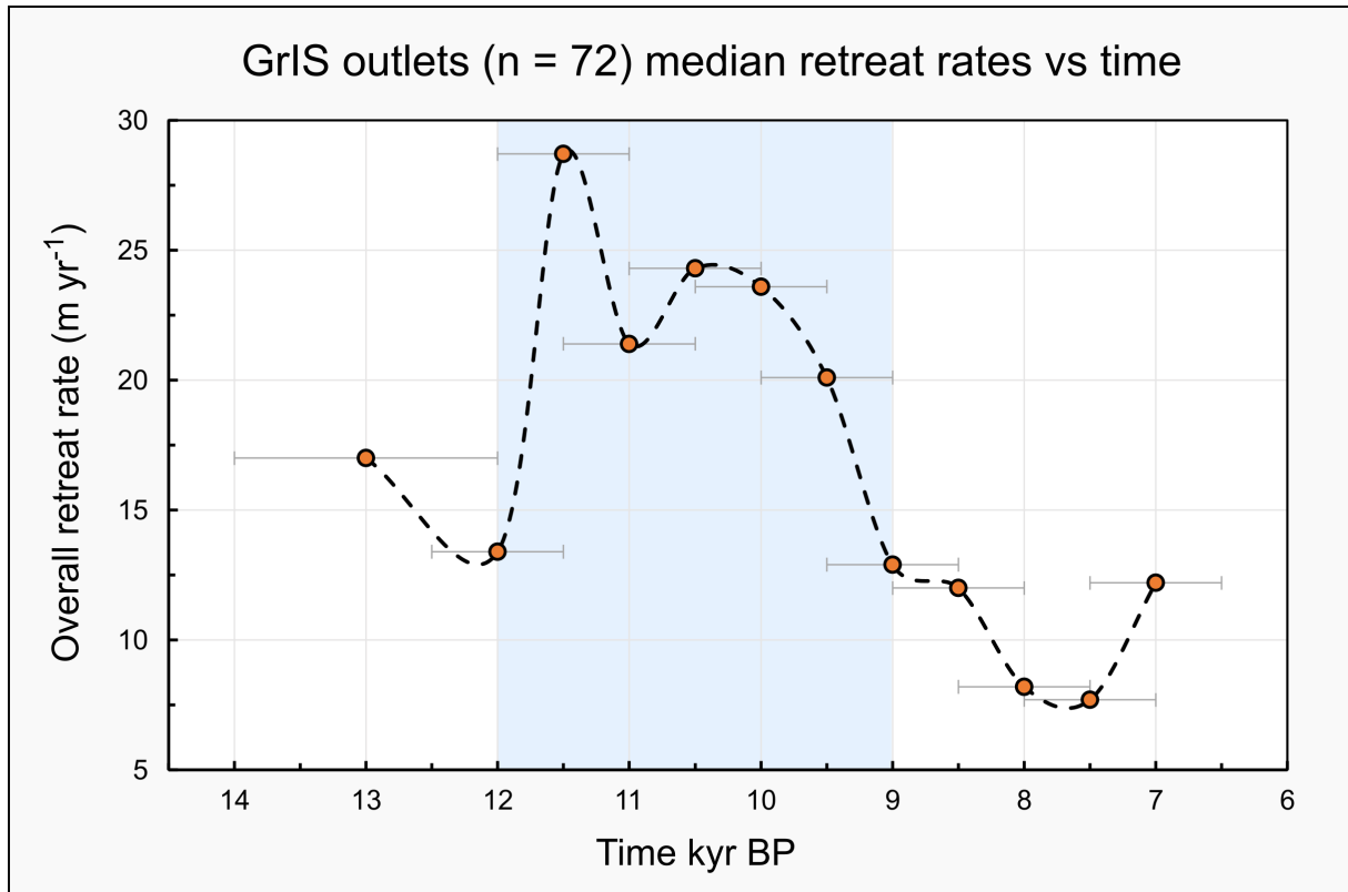
2095 Figure 19. Time series denoting the evolution of the median retreat rate for all outlet glaciers sampled over the full reconstruction period (14-6.5 kyr BP). The blue polygon highlights a period of general acceleration in Greenland Ice Sheet outlet glacier retreat speed (see section 3.4). It is important to note that the youngest time slices are here associated with less than 72 data points, as our reconstruction features certain outlet glacier margins reaching present-day extent before others.
