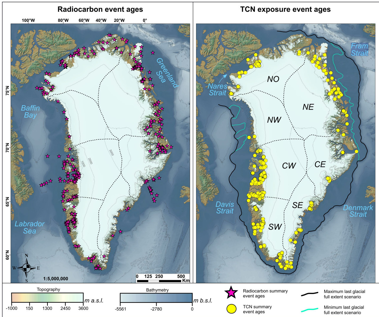
480 Figure 5. Spatial distribution of radiocarbon - derived (left-hand panel) and TCN exposure age - derived (right-hand panel) 485 summary event ages (post filtering and statistics) used to produce the PaleoGrIS 1.0 isochrone reconstruction. Topographic and bathymetric data (GEBCO 2022 release) is overlaid with 1000 m interval contour lines. The dashed line shows our division scheme of the ice-sheet in seven main drainage regions that we refer to throughout the paper and in associated quantitative analyses, after the drainage basin sampling scheme of Rignot & Mouginot (2012), labelled on the right hand panel. The right-hand panel also features lines denoting our estimations of maximum and minimum scenarios of last full glacial Greenland Ice Sheet extent (grounded ice only), based on a review of the literature (see section 2.6), and which informs the mapping of our outermost isochrones.
