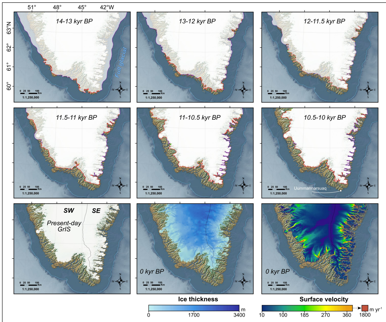
1475 Figure 11. Time slice maps of the PaleoGrIS 1.0 isochrone reconstruction in southernmost Greenland. The reconstructed ice sheet areal extent for each given time slice is displayed in each sub-panel as a white transparent polygon, while the underlying opaque white layer is the present-day ice cover from BedMachine v4. The reconstructed ice sheet margins are highlighted by our isochrone polylines, which feature different colour schemes (see Fig. 8 for key) relating to our four isochrone confidence levels (see section 2.3.5). Bottom panels also feature present-day ice-sheet thickness (Morlighem et al., 2017) and surface velocity data (Joughin et al., 2018). Topography and bathymetry are from the GEBCO 2022 release. For a more complete figure legend, the reader is advised to consult Figure 8.
