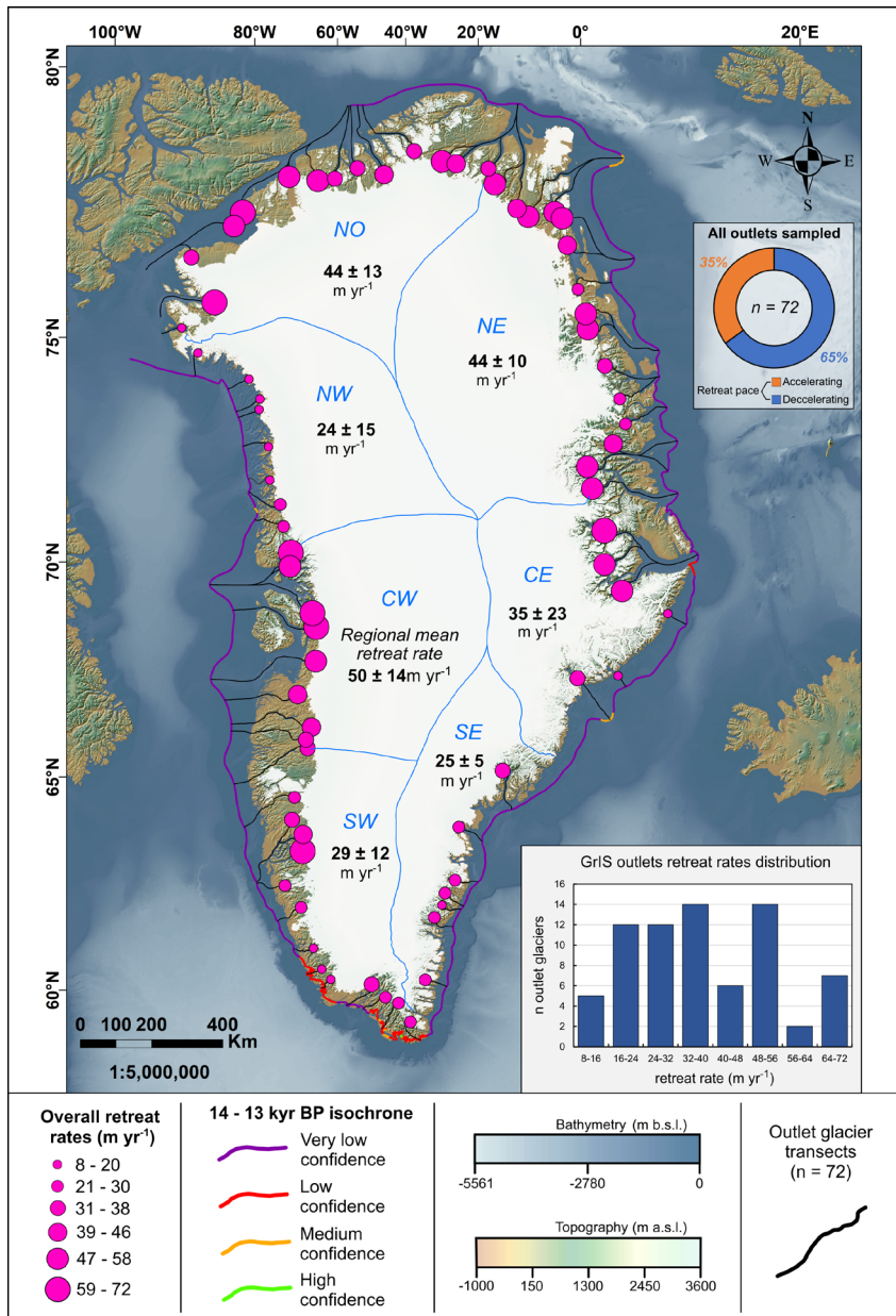
Figure 18. Map of Greenland Ice Sheet outlet glacier transects (black lines, n = 72 ) drawn to conduct a retreat rate analysis (see section 3.4.) using PaleoGrIS 1.0 isochrones, the main results of which are also shown here. Retreat rates over the full reconstruction period ( \sim 14 -6.5 kyr BP) are denoted using pink circles characterised by sizes proportional to overall retreat rate magnitudes. Our outermost isochrone (14-13 kyr BP), which marks the outer edge of our transect mapping, is shown with its spatially-variable colour-coded confidence levels. Towards the bottom right-hand corner, a histogram of overall retreat rate distribution is shown as split in eight bins of retreat rate magnitude. Moreover, bold black numbers indicate the regional mean overall retreat rate ( \pm 1\sigma S.D.) for each of the seven ice-sheet regions sampled. Towards the top right-hand corner, a doughnut diagram highlights the relative proportions of outlet glacier retreat rates indicating decelerating (65%) vs accelerating (35%) trends over the full reconstruction period.
