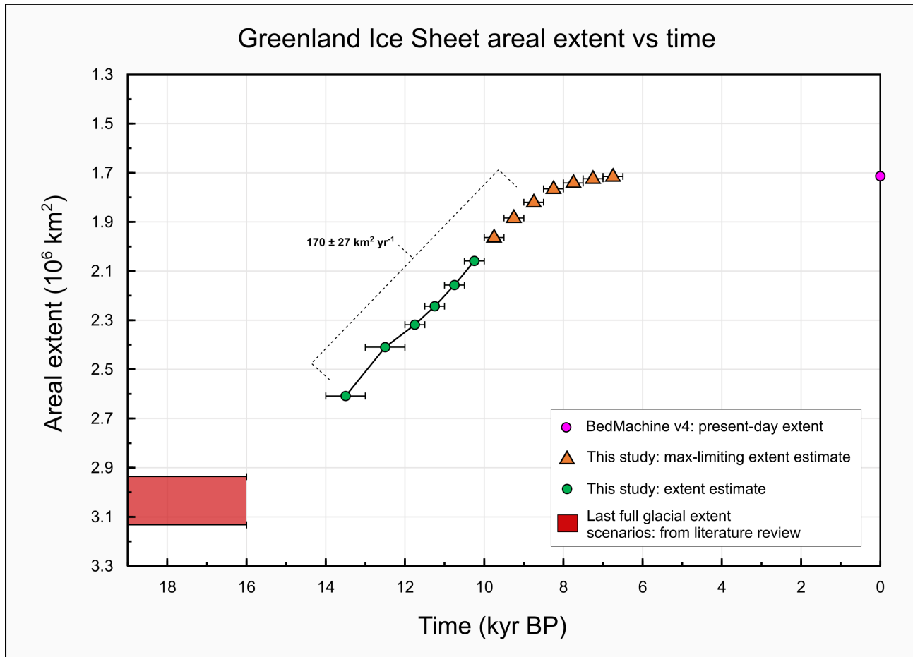
Figure 16. Empirical estimation of the Greenland Ice Sheet areal extent evolution between ~18 kyr BP and present. The ice sheet extent during last full glacial configuration (red box) is here estimated by bracketing maximum (at continental shelf break everywhere) and minimum extent scenarios reconstructed after consulting the relevant literature, in an attempt to highlight the uncertainties in several debated regions (more details in section 2.6). The hypothetical timing of such full glacial extent is crudely associated with maximum atmospheric and oceanic cooling over Greenland during Heinrich Stadial 1 (Buizert et al., 2018), but we stress the timing of maximum extent is unknown and could have been reached before 18 kyr BP, and until Bølling–Allerød warming started after ~16 kyr BP, as highlighted by our conservative range (red box). Ice sheet areal extent estimates from the PaleoGrIS 1.0 isochrone reconstruction are shown with green circles (actual extent estimates) and orange triangles (maximum-limiting extent: pointing upwards). This differentiation is due to our isochrones not covering the full ice-sheet perimeter during the ~10–6.5 kyr BP interval, when some sections of the ice sheet margin are estimated to have been as- or more-retreated-than-present margins.
