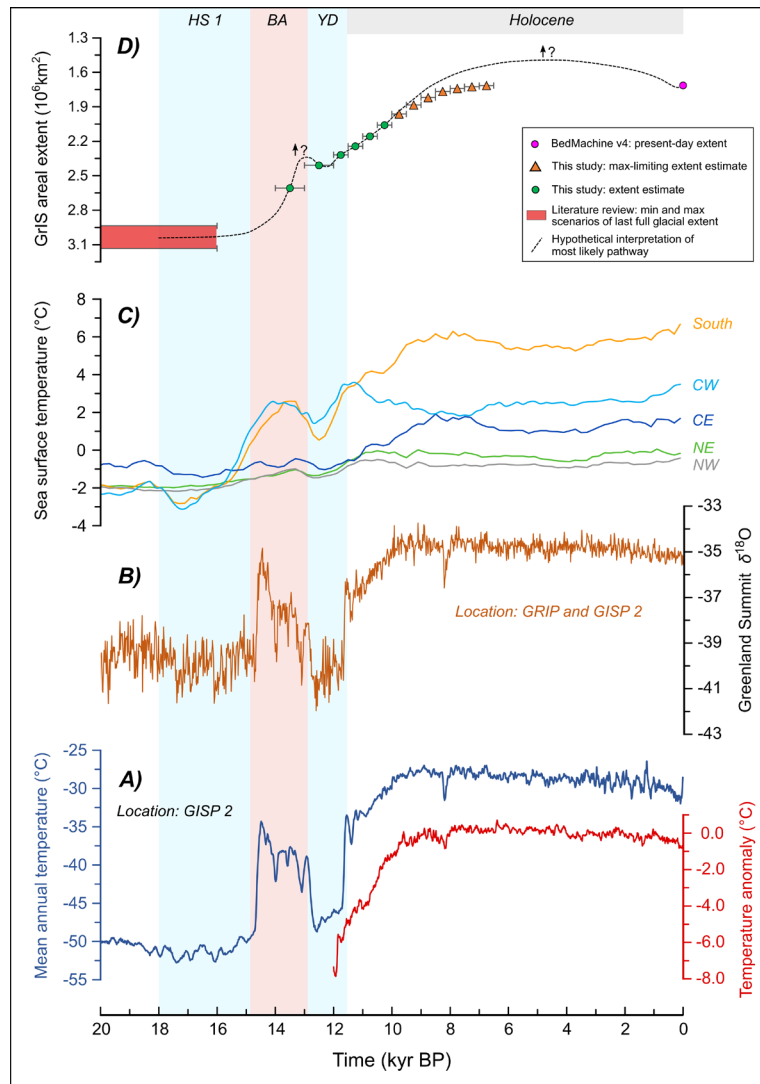
Figure 21. Comparison between our reconstruction of Greenland Ice Sheet areal extent evolution and past atmospheric / sea surface temperature reconstructions from proxy and model data, between 20 kyr BP and present. A) Blue curve: reconstruction of mean annual near-surface temperature at location of the GISP 2 ice core (72.58°N; -38.48°W) by Buizert et al. (2018a), who merged Greenland ice core temperature reconstructions (GISP2, NGRIP, NEEM) with the TraCE-21ka simulations. Red curve: ensemble mean reconstruction of mean annual temperature anomaly (towards GISP 2 ice core location) relative to a 5-3 kyr BP reference period, by Erb et al. (2022), who use the global Holocene paleo-temperature proxy database of Kaufman et al. (2020) to conduct data assimilation on HadCM3 and TraCE-21ka simulations. B) The Greenland Summit \delta^{18}\text{O} record (Buizert et al., 2018b) that averages the GISP2 and GRIP \delta^{18}\text{O} records. C) Reconstructions of sea surface temperature at different locations offshore Greenland, using the ensemble mean ( n=500 ) from the LGMR global dataset of Osman et al. (2021), who use a paleoclimate data assimilation scheme to correct biases in climate simulations of the iCESM (versions 1.2 and 1.3). Coordinates for time series: ‘South’ (Cape Farewell): 58.34°N; -43.25°W, ‘CW’ (Davis Strait): 64.72°N; -56.53°W, ‘CE’ (Denmark Strait): 66.64°N; -27.26°W, ‘NE’ (Nordic Sea): 72.25°N; -10.10°W, ‘NW’ (Baffin Bay): 73.17°N; -62.65°W. D) Greenland Ice Sheet areal extent reconstruction from literature review (LGM - HS 1 period), the PaleoGrIS 1.0 isochrones (this study: ~14-6.5 kyr BP), and BedMachine v4 (Morlighem et al., 2017).
