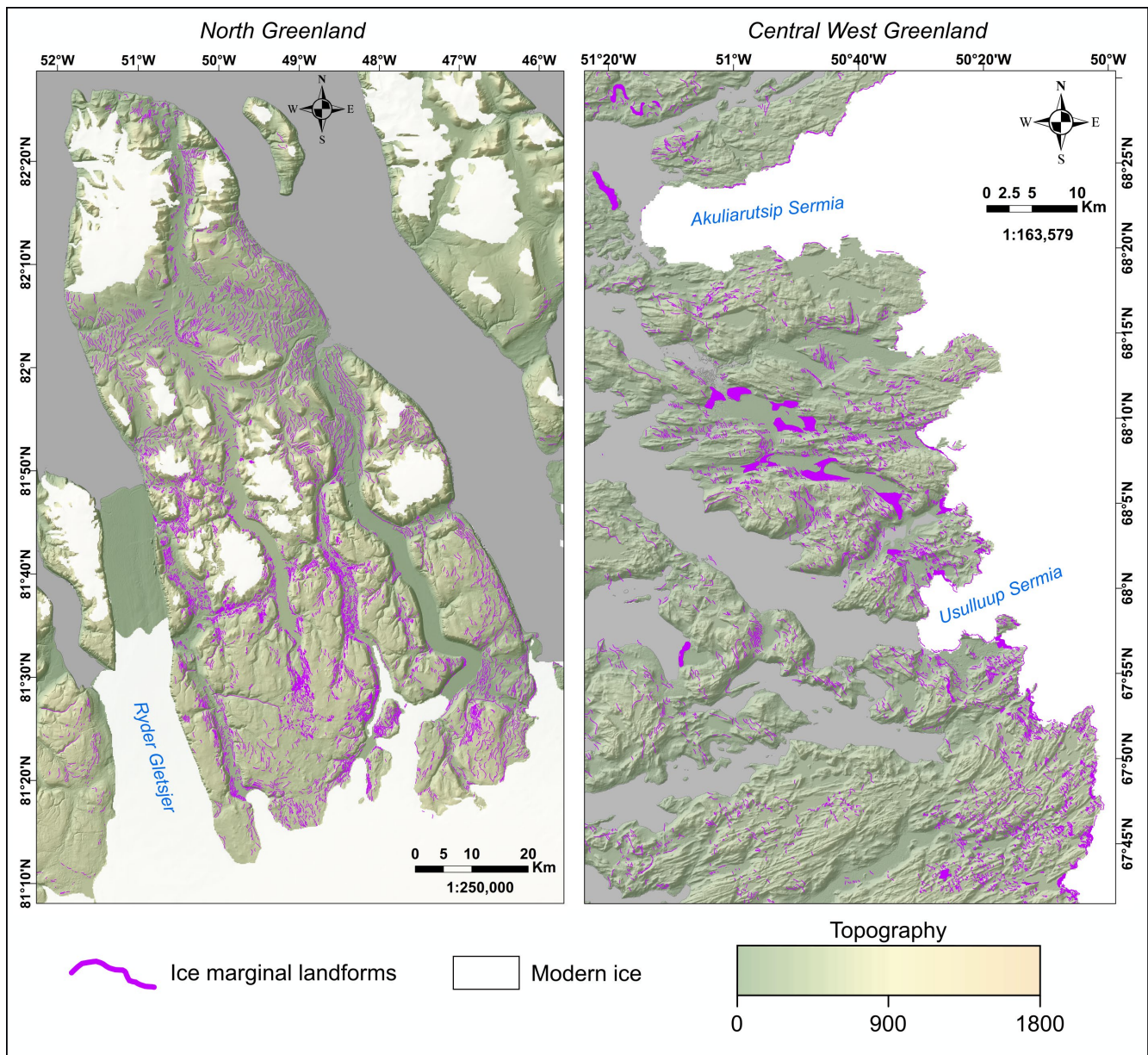
270 Figure 3. Examples of mapped ice-marginal landforms in two distinct regions displaying high density and preservation of ice-marginal glacial deposits. The mapped landforms are displayed overlaying topographic data from the AW3D30 DEM (30 m resolution). The left-hand panel presents mapping in a region of North Greenland (also referred to as Wulffs Land), while the right-hand panel focuses on the deglaciated region directly South of Disko Bay, in central West Greenland.
