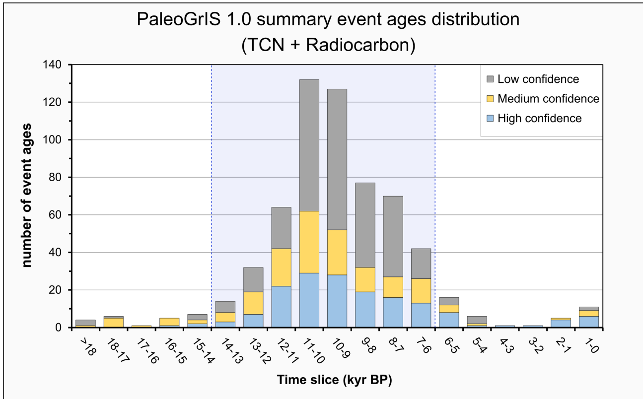
Figure 7. Histogram displaying the temporal distribution of all summary event ages calculated in the PaleoGrIS 1.0 database. Colour-coded relative proportions of the three quality control categories are shown for each thousand-year bin. A light-blue polygon highlights the time period covered by the PaleoGrIS 1.0 isochrone reconstruction. This Late-Glacial-to-mid-Holocene period (14-6.5 kyr BP) features the large majority (>90%) of compiled event ages dating the deglacial evolution of former Greenland Ice Sheet margins.
