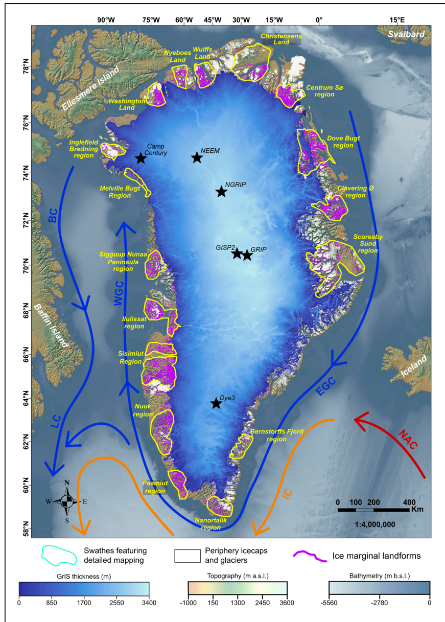
160 Figure 1. Greenland geographical context, present-day ice sheet thickness (BedMachine v4; Morlighem et al., 2017), and location of 18 regions (boxes outlined in light green) where detailed ice-marginal landform mapping (displayed in purple) was conducted as part of this study. Note few areas were mapped in detail in the southeast due to relative lack of ice-free land. A simplified pattern of contemporary ocean circulation is represented, after Yang et al. (2016; Fig. 1); whereby red and orange arrows symbolize warmer Atlantic-origin water while blue arrows represent colder Arctic-origin water. NAC, IC, EGC, WGC, BC, and LC stand for North Atlantic, Irminger, East Greenland, West Greenland, Baffin, and Labrador Currents, respectively. The Digital Elevation Model (DEM) displaying both topographic and bathymetric data is from the GEBCO 2022 release (450 m resolution). Geographical extent of Greenland periphery icecaps and glaciers (white polygons) is from BedMachine v4. The locations of main Greenland ice cores (further mentioned in text) are shown by black stars. All data (here and in subsequent figures) are displayed projected to the WGS 84 / NSIDC Sea Ice Polar Stereographic North coordinate reference system.
