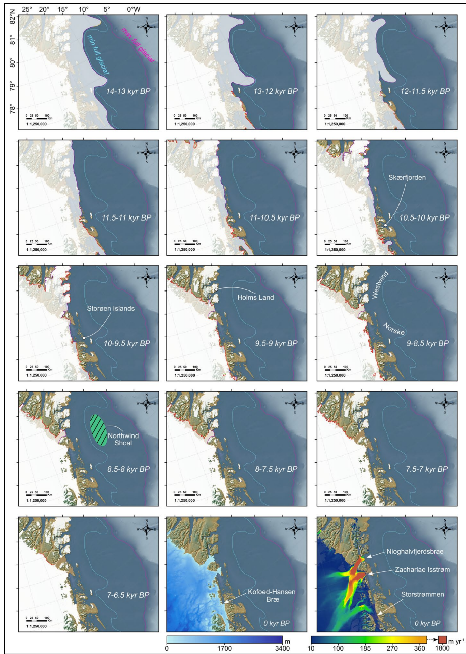
1280 Figure 9. Time slice maps of the PaleoGrIS 1.0 isochrone reconstruction in the Nioghalvfjordsfjorden and Jøkelbugten region. The 1285 reconstructed ice sheet areal extent for each given time slice is displayed in each sub-panel as a white transparent polygon, while the underlying opaque white layer is the present-day ice cover from BedMachine v4. The reconstructed ice sheet margins are highlighted by our isochrone polylines, which feature different colour schemes (see Fig. 8 for key) relating to our four isochrone confidence levels (see section 2.3.5). Bottom panels also feature present-day ice-sheet thickness (Morlighem et al., 2017) and surface velocity data (Joughin et al., 2018). Topography and bathymetry are from the GEBCO 2022 release. For a more complete figure legend, the reader is advised to consult Figure 8.
