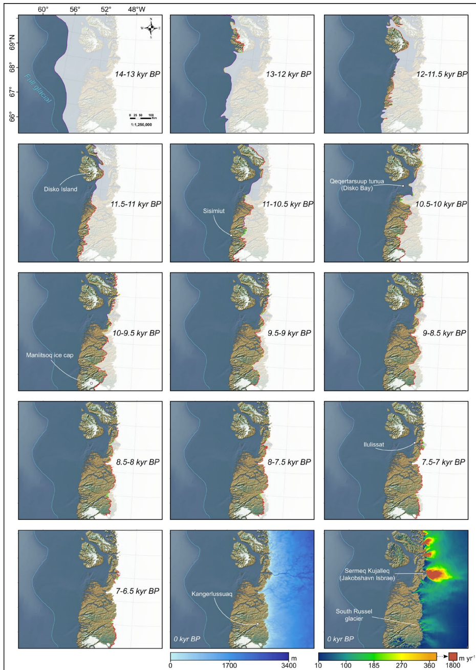
1680 Figure 13. Time slice maps of the PaleoGrIS 1.0 isochrone reconstruction in Sisimiut and Disko Bay region. The reconstructed ice sheet areal extent for each given time slice is displayed in each subpanel as a white transparent polygon, while the underlying opaque white layer is the present-day ice cover from BedMachine v4. The reconstructed ice sheet margins are highlighted by our isochrone polylines, which feature different colour schemes (see Fig. 8 for key) relating to our four isochrone confidence levels (see section 2.3.5). Bottom panels also feature present-day ice-sheet thickness (Morlighem et al., 2017) and surface velocity data (Joughin et al., 2018). Topography and bathymetry are from the GEBCO 2022 release. For a more complete figure legend, the reader is advised to consult Figure 8. 1685
