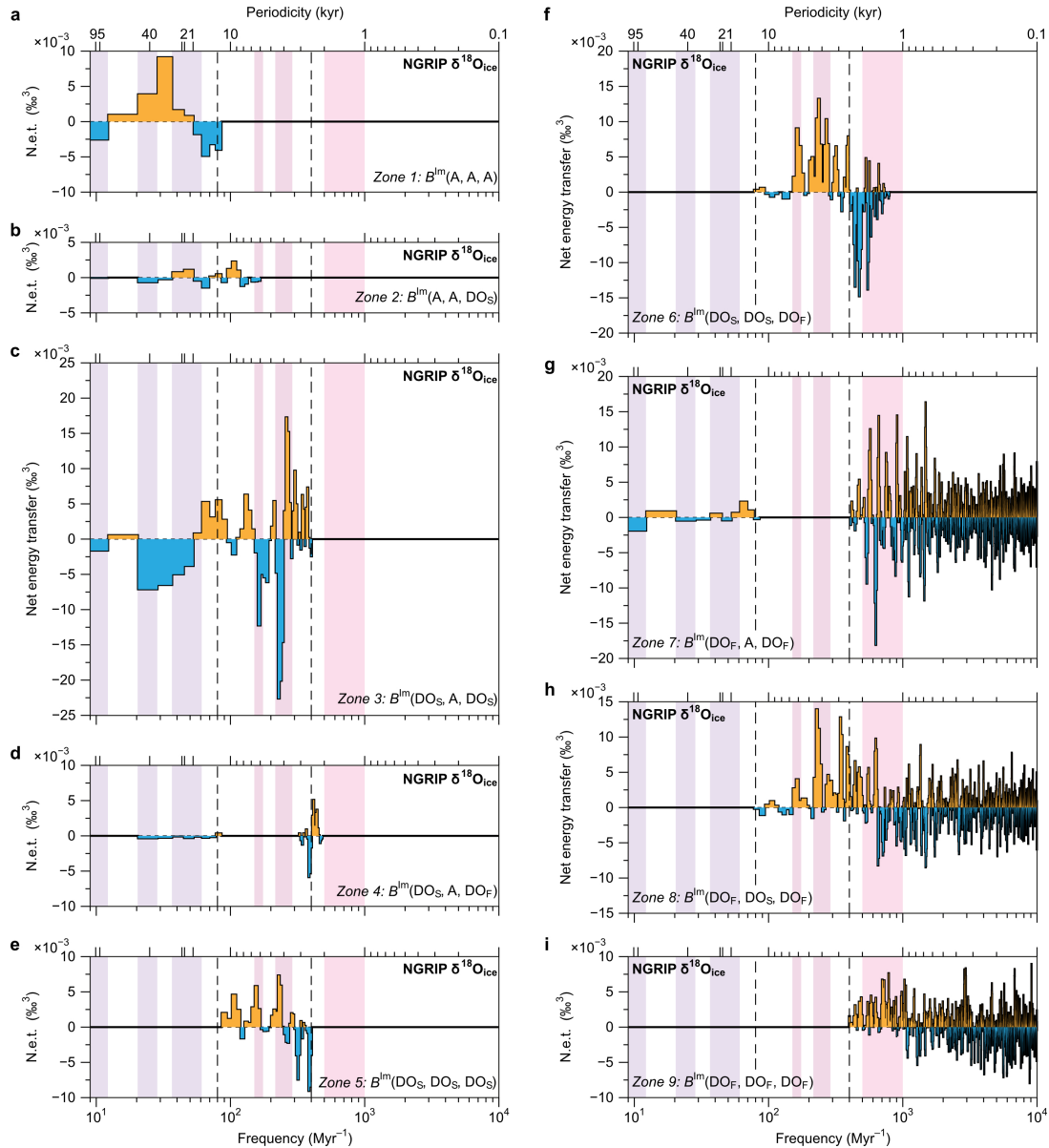
Figure 4: Zonal integrations of the bispectrum. Integrations of (a) Zone 1: B^{\text{lm}}(\text{A}, \text{A}, \text{A}) , (b) Zone 2: B^{\text{lm}}(\text{A}, \text{A}, \text{DOs}) , (c) Zone 3: B^{\text{lm}}(\text{DOs}, \text{A}, \text{DOs}) , (d) Zone 4: B^{\text{lm}}(\text{DOs}, \text{A}, \text{DOF}) , (e) Zone 5: B^{\text{lm}}(\text{DOs}, \text{DOs}, \text{DOs}) , (f) Zone 6: B^{\text{lm}}(\text{DOs}, \text{DOs}, \text{DOF}) , (g) Zone 7: B^{\text{lm}}(\text{DOF}, \text{A}, \text{DOF}) , (h) Zone 8: B^{\text{lm}}(\text{DOF}, \text{DOs}, \text{DOF}) , and (i) Zone 9: B^{\text{lm}}(\text{DOF}, \text{DOF}, \text{DOF}) . “ B^{\text{lm}} ” stands for the imaginary part of the bispectrum. “A” stands for astronomical periodicities, “DOs” stands for slow-DO periodicities, “DOF” stands for fast-DO and centennial periodicities. Orange indicates net energy gains, blue net energy losses. Dashed vertical black lines mark the zone boundaries between the main periodicity bandwidths, with the main astronomical periodicities highlighted in purple, slow-DO periodicities in plum, and fast-DO periodicities in pink.
