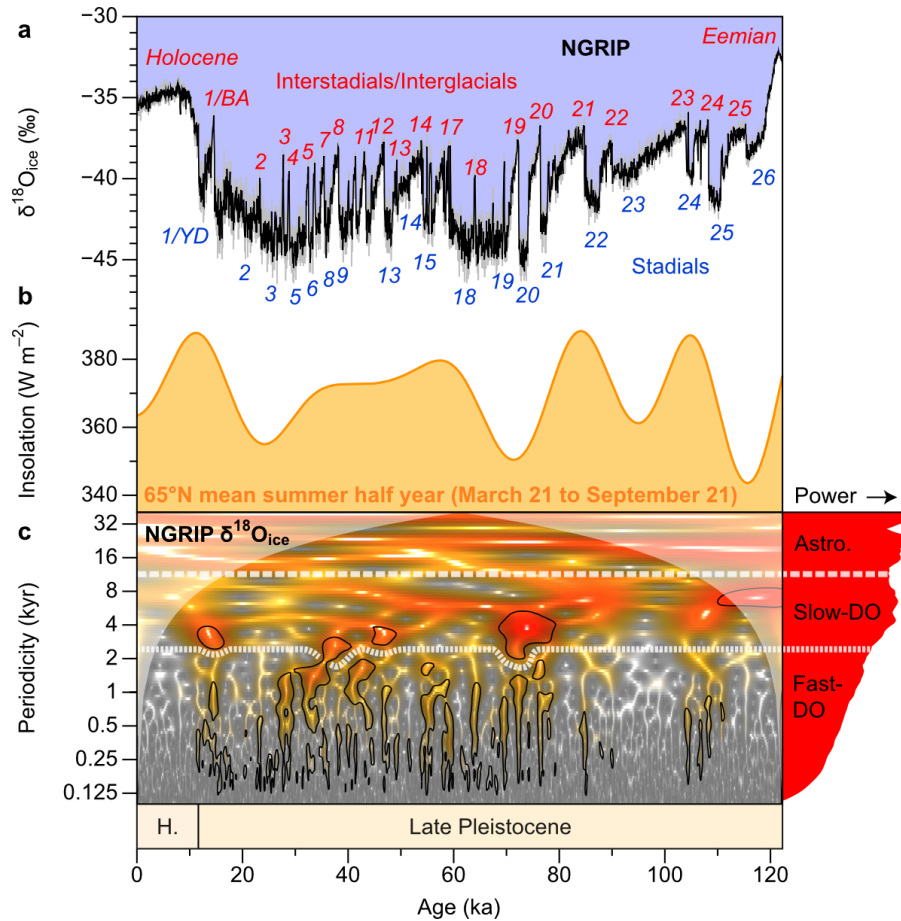
Figure 1: The NGRIP \delta^{18}\text{O}_{\text{ice}} record versus summer insolation at 65° N. (a) The NGRIP \delta^{18}\text{O}_{\text{ice}} record on the 230 “GICC05modelext” age model (Vinther et al., 2006; Rasmussen et al., 2006; Andersen et al., 2006; Svensson et al., 2008; Wolff et al., 2010) versus (b) mean summer half year insolation at 65° N (March 21 to September 21) for the past 123 ka (Laskar et al., 2004). In panel (a): grey line represents the NGRIP \delta^{18}\text{O}_{\text{ice}} record with 20-year sample spacing, used for bispectral analyses (Fig. 2–4). Black line represents the NGRIP \delta^{18}\text{O}_{\text{ice}} record with a 50-year sample spacing, used for the wavelet analysis (panel c). (c) Wavelet analysis of the Gaussian filtered NGRIP \delta^{18}\text{O}_{\text{ice}} record (see Methods ). Black contours 235 represent the 95% significance level with respect to a red noise model. The colours of the wavelet indicate amplitude (white/grey = low amplitude, yellow/orange/red = high amplitude). We note that colour/amplitude does not equate to statistical significance with respect to the red noise model. An average of the entire wavelet spectrum is shown on the right- hand side in red. The two white dashed lines indicate the spectral gaps between astronomical and slow-DO periodicities (broad dashes), and between slow-DO and fast-DO periodicities (narrow dashes). “H” stands for Holocene, “BA” stands for 240 Bølling–Allerød, and “YD” stands for Younger Dryas. The latter two together correspond to DO Cycle-1.
