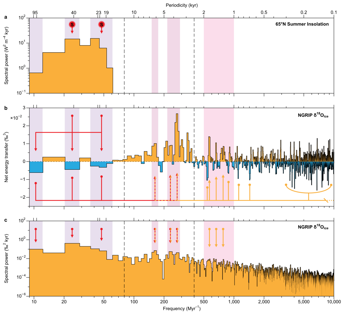
255 Figure 3: Linking DO cycles to energy sources. Comparison of (a) power spectrum of mean summer half year insolation record at 65°N (March 21 to September 21), to (b) total integration of the bispectrum of the NGRIP \delta^{18}\text{O}_{\text{ice}} record, and (c) the power spectrum of the NGRIP \delta^{18}\text{O}_{\text{ice}} record. Orange indicates spectral power (panel a and c), or net energy gains (panel b), and blue indicates net energy losses (panel b). Red and orange arrows indicate the two main energy transfer pathways across the spectral continuum to slow- and fast-DO cycles. These interpretative arrows are derived from both the total (this figure) and the zonal integration (see also Fig. 4). Dashed vertical black lines mark the zone boundaries between astronomical periodicities (purple), slow- (plum), and fast-DO (pink) and centennial periodicities. “S” stands for sun/solar forcing, indicating at which frequencies summer insolation provides energy. No 123 kyr long record of sunspot cycles exist, which is why we do not show a spectrum of this energy source here. Furthermore, the highest amplitude spectral power of the solar cycle over the past 123 kyr is expected to fall at around the annual and \sim 11 -year periodicities. These cycles are not resolved in the NGRIP \delta^{18}\text{O}_{\text{ice}} record, which is marked by a 20-year sample spacing. 260 265
