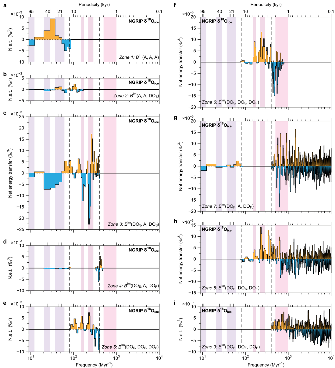
Figure 4: Zonal integrations of the bispectrum. Integrations of (a) Zone 1: B^{\text{lm}}(\text{A}, \text{A}, \text{A}) , (b) Zone 2: B^{\text{lm}}(\text{A}, \text{A}, \text{DO}_S) , (c) Zone 3: B^{\text{lm}}(\text{DO}_S, \text{A}, \text{DO}_S) , (d) Zone 4: B^{\text{lm}}(\text{DO}_S, \text{A}, \text{DO}_F) , (e) Zone 5: B^{\text{lm}}(\text{DO}_S, \text{DO}_S, \text{DO}_S) , (f) Zone 6: B^{\text{lm}}(\text{DO}_S, \text{DO}_S, \text{DO}_F) , (g) Zone 7: B^{\text{lm}}(\text{DO}_F, \text{A}, \text{DO}_F) , (h) Zone 8: B^{\text{lm}}(\text{DO}_F, \text{DO}_S, \text{DO}_F) , and (i) Zone 9: B^{\text{lm}}(\text{DO}_F, \text{DO}_F, \text{DO}_F) . “ B^{\text{lm}} ” stands for the imaginary part of the bispectrum. “A” stands for astronomical periodicities, “ \text{DO}_S ” stands for slow-DO periodicities, “ \text{DO}_F ” stands for fast-DO and centennial periodicities. Orange indicates net energy gains, blue net energy losses. Dashed vertical black lines mark the zone boundaries between the main periodicity bandwidths, with the main astronomical periodicities highlighted in purple, slow-DO periodicities in plum, and fast-DO periodicities in pink.
