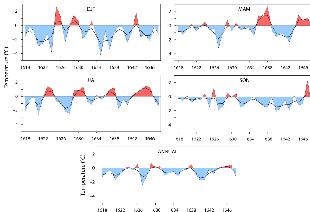
Figure 1: Fluctuations in mean seasonal and annual temperatures in Central Europe during 1618–1648 expressed as anomalies with respect to the 1961–1990 reference (further as w.r.t. 1961–1990). Smoothed by 5-year Gaussian filter (data: Dobrovolný et al., 2010).
