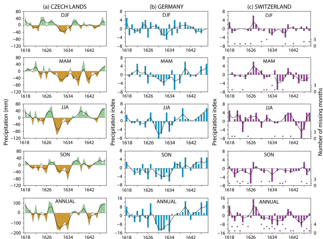
275 Figure 3: Precipitation fluctuations in Central Europe during 1618–1648: (a) anomalies in mean seasonal and annual precipitation totals in the Czech Lands w.r.t. 1961–1990 (data: Dobrovolný et al., 2015); (b) documentary-based seasonal and annual precipitation indices for Germany (data: https://www.tambora.org ); (c) same as (b), but for Switzerland (data: https://www.euroclimhist.unibe.ch/ ); points declare the number of missing months in calculation of seasonal or annual indices. Smoothed by a 5-year Gaussian filter.
