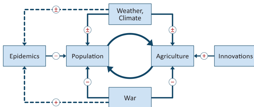
635 Figure 13: A simplified scheme of four main external determinants affecting population size in a largely self-sufficient, organic economy. The plus symbol “+” indicates an enhancement of relationship and the minus symbol “-” its weakening (© Pfister/Wanner, Climate and Society in Europe. The Last Thousand Years . Haupt Verlag, 2021, p. 251).
