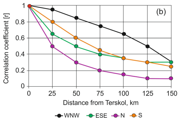
Figure 5. Spatial correlation function of the annual precipitation calculated relative to the Terskol meteorological station (red dot) (a): isolines of correlation coefficients calculated according to Student's t-test are given by white lines; dashed lines indicate the profiles for which the correlation function was calculated. Correlation function values along these profiles (b). ArcGIS World Imagery Basemap used as the background. Source: DigitalGlobe.
