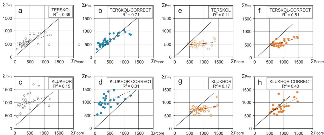
375 Figure 7. Regression relations between the accumulation layer on the West Elbrus plateau ( \Sigma P_{\text{core}} , mm) and precipitation amounts at the nearest weather stations ( \Sigma P_{\text{ws}} , mm) during 1979-2009 CE period: (a-d) for the cold season (a, c for October-March calendar period, b, d for the cold period highlighted by CAPE value thresholds); (e-h) for the warm season (e, f) for the April-September calendar period, (g, h) for the warm period highlighted by CAPE values).
