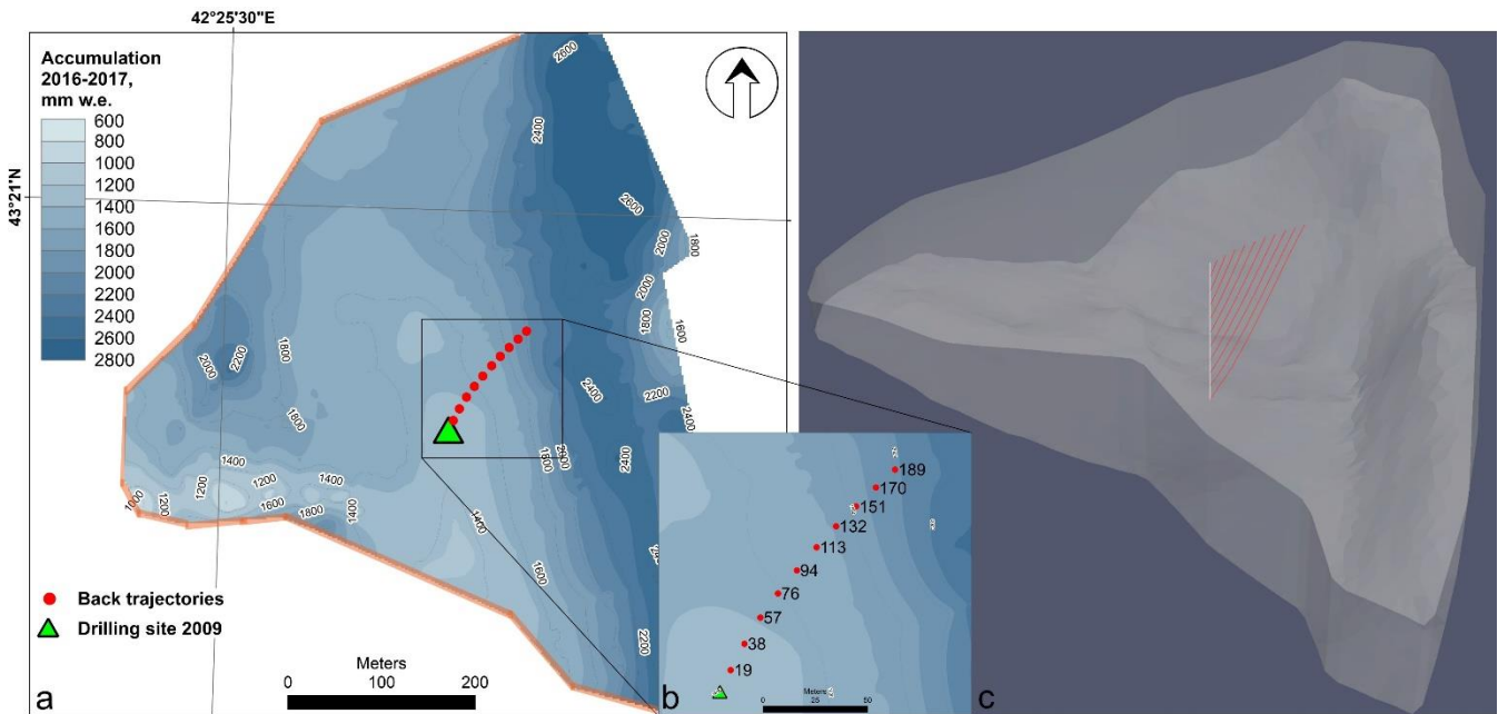
Figure 3. Accumulation map for the Western plateau of Elbrus in 2016–2017 CE (Lavrentiev et al., 2022) (a); the modeled catchment area for the 2009 CE ice core (b); and the computational domain (c) with the borehole position (white line) and the calculated backward trajectories (red lines). An orange line shows the outflow zone. The source points of the backward trajectories are marked with red dots; the corresponding borehole depths (rounded, in m) according to DEM (2017) are given as dot labels. The green triangle indicates the position of the ice core (2009).
