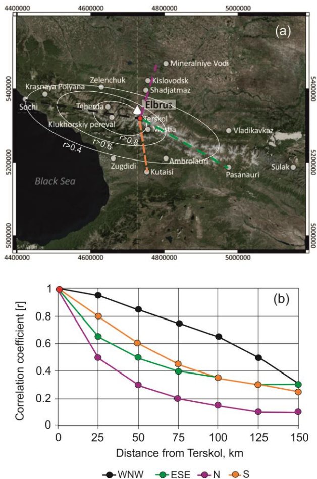
390 Figure 5. Spatial correlation function of the annual precipitation calculated relative to the Terskol meteorological station (red dot) (a): isolines of correlation coefficients calculated according to Student's t-test are given by white lines; dashed lines indicate the profiles for which the correlation function was calculated. Correlation function values along these profiles (b). ArcGIS World Imagery Basemap used as the background. Source: DigitalGlobe.
