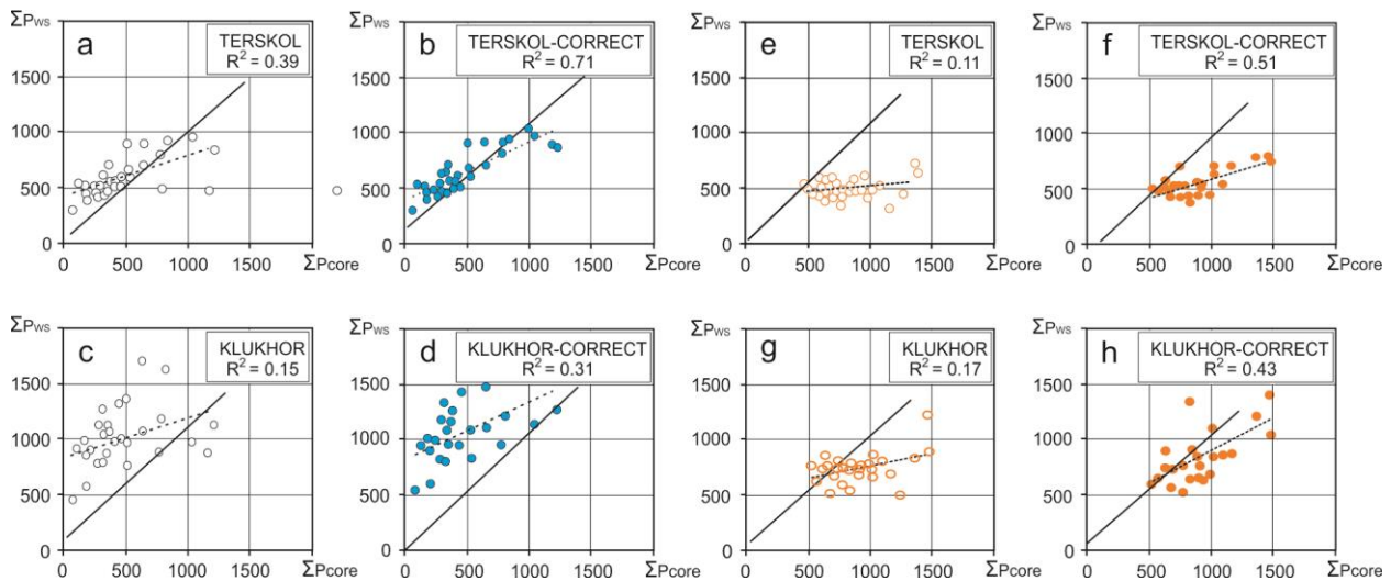
Figure 7. Regression relations between the accumulation layer on the West Elbrus plateau ( \Sigma P_{core} , mm) and precipitation amounts at the nearest weather stations ( \Sigma P_{ws} , mm) during 1979-2009 CE period: (a-d) for the cold season (a, c for October-March calendar period, b, d for the cold period highlighted by CAPE value thresholds); (e-h) for the warm season (e, f) for the April-September calendar period, (g, h) for the warm period highlighted by CAPE values).
