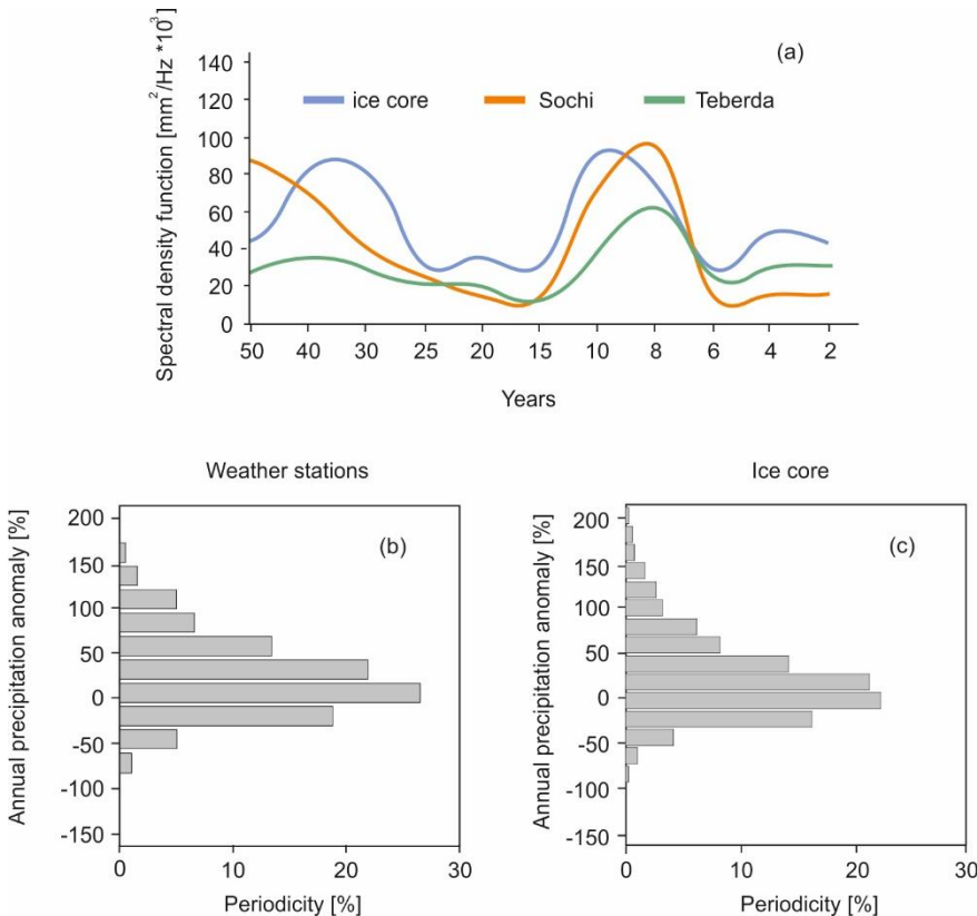
Figure 6. Statistical analysis of the data time series on the longest-range weather stations and ice cores: (a) spectral analysis of the series, (b) empirical distribution function of annual precipitation anomalies compared to the period 1981-1951-2010-1980 , averaged between data from the longest-row weather stations Sochi, Krasnaya Polyana , Teberda and Sulak-Vysokogornaya , (c) empirical
