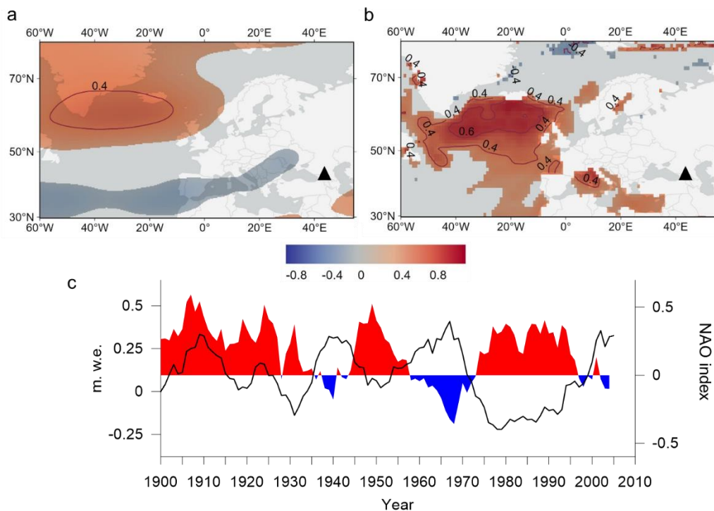
510 Figure 10. Spatial correlation of the detrended winter (October-March) annual accumulation at WP with ERA5 500 mb geopotential height data (a) and sea surface temperature (HadISST1) data in 1950-2009 (b). Ten-year moving average of winter
