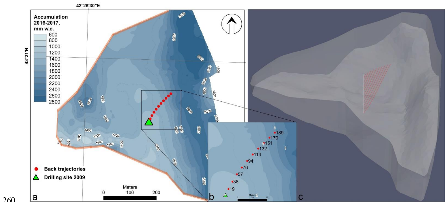
260 Figure 3. Accumulation map for the Western plateau of Elbrus in 2016–2017 CE (Lavrentiev et al., 2022) (a); the modeled catchment area for the 2009 CE ice core (b); and the computational domain (c) with the borehole position (white line) and the calculated backward trajectories (red lines). An orange line shows the outflow zone. The source points of the backward trajectories are marked with red dots; the corresponding borehole depths (rounded, in m) according to DEM (2017) are given as dots labels. The green triangle indicates the position of the ice core (2009). 265
