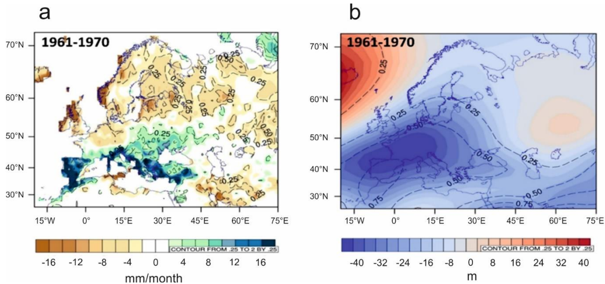
505 Figure 9 An average winter precipitation anomalies in 1961 – 1970 (GPCC) compared to 1981 – 2010 (a) and average 500 hPa isobaric surface height anomalies (NCEP/NCAR) (b).
