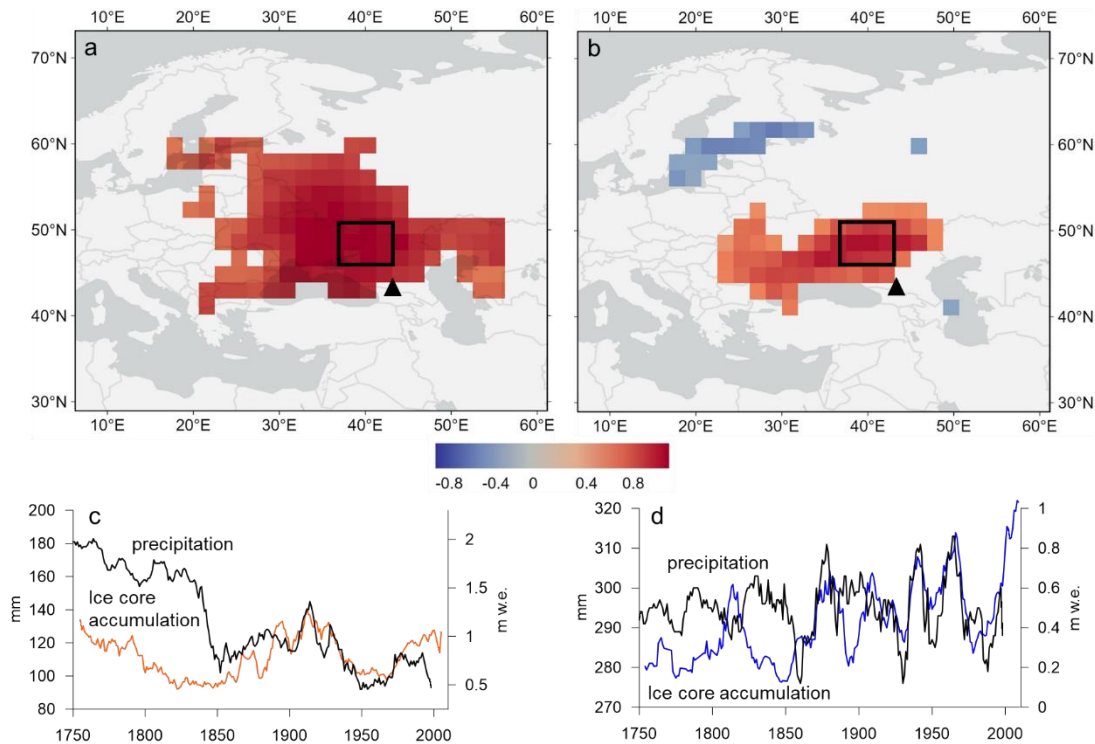
590 Figure 1011. Spatial correlation of the 10-year moving average of summer (a) (April-September) and winter (b) (October-March) WP accumulation with EK400v2 paleo reanalysis ensemble mean precipitation data over 1900-2003 period, time series of the precipitation data averaged over the area indicated by the black box for summer (c) and winter (d) shown together with WP accumulation data. Location of the Elbrus Mt. is shown by black triangle.
