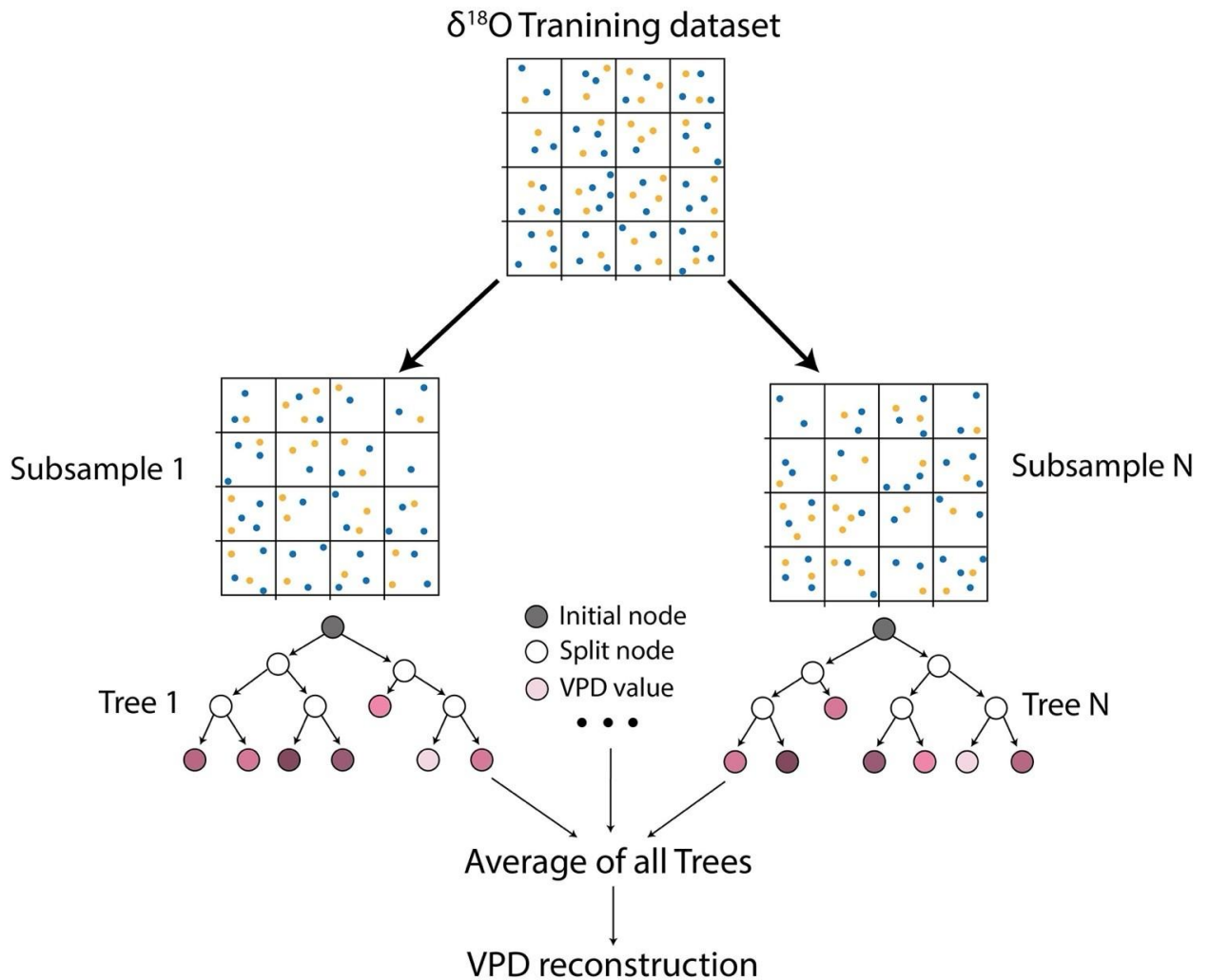
Figure S1: Simplified illustration of the RF approach for our VPD reconstruction
