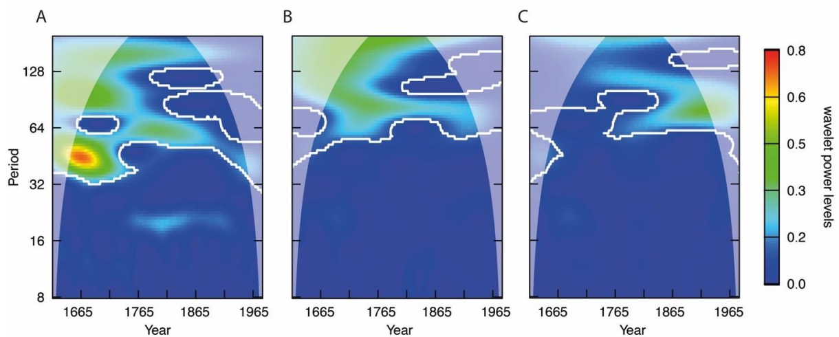
Figure S2: Investigation of the different spectra of the rolling mean time series of the three reconstructed areas. A, North Europe, B, Central Europe and C, Mediterranean region. The white contour lines indicate significant frequencies ( p < 0.01 ). All the plots are done with the WaveletComp package in R (Rosch and Schmidbauer, 2018).
