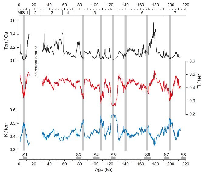
Figure 4: XRF data from core KL11 (5-point running average). Terr/Ca gives the ratio between the sum of terrigenous elements and Ca. Ti and K were normalised by calculating their portion on the terrigenous elements. No data are available from the calcareous crust. The main peak humid periods as inferred from the XRF data are indicated by vertical grey bars. Marine isotope stages (MIS) are indicated at the top; horizontal bars at the bottom indicate sapropel layers S1–S8 in the eastern Mediterranean Sea associated with the African Humid Periods.
