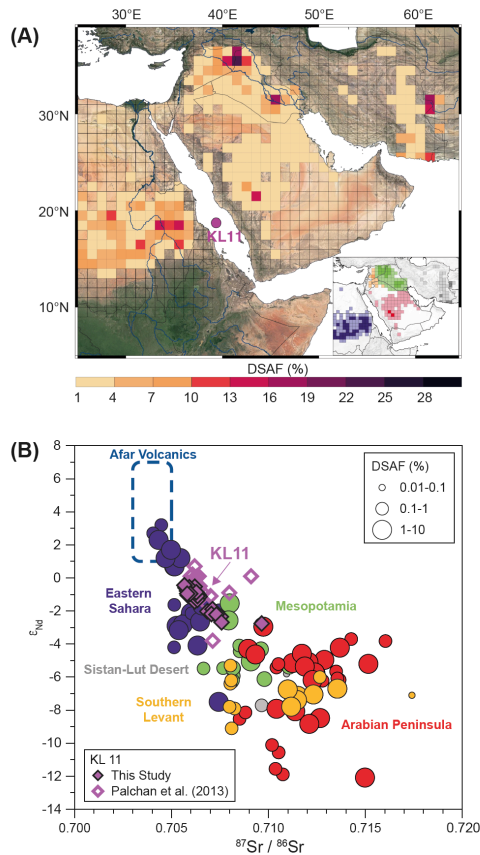
335 Figure 6: Fingerprinting the provenance and transport pathway of the terrigenous fraction supplied to the central Red Sea (core KL11) using its Sr and Nd isotope composition. (A) Dust source activation frequency map of Northeast Africa and Southwest Asia (DSAF, calculated as the percentage of days wherein one or more dust events are recorded in a 1° x 1° grid cell; after Kunkelova et al., 2022, and references therein). Background: © Google Earth. Inset shows the preferential dust source areas defined by Kunkelova et al. (2022) colour coded as in panel B. (B) Comparison of Sr and
