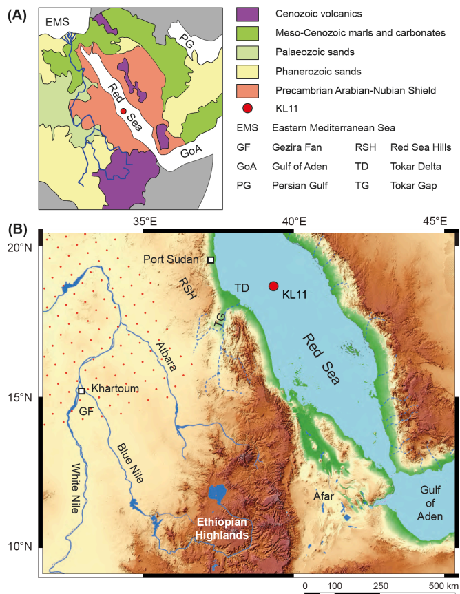
75 Figure 1: Location of the investigated marine sediment core KL11 in the Red Sea. (A) Overview of the Red Sea and the geology of its hinterland (after Stein et al., 2007, and Palchan et al., 2013). (B) Topography of the area around the central and southern Red Sea. The main dust source of the Eastern Saharan Potential Source Area (ESPSA) is indicated by hachures (after Kunkelova et al., 2022). Topographic map source: OpenTopoMap (CC-BY-SA).
