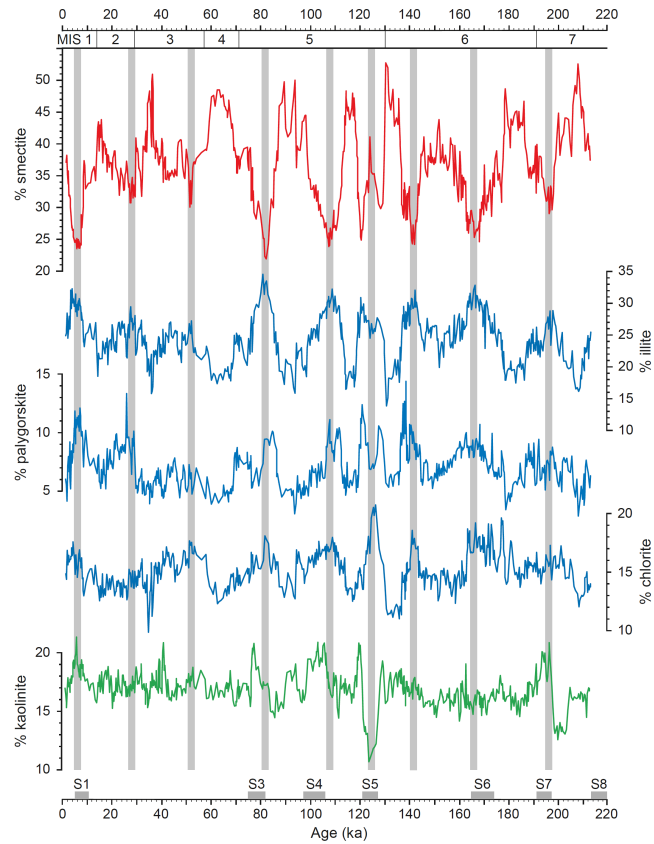
245 Figure 3: Clay mineral composition of sediments from core KL11. The main peak humid periods as inferred from minima in the smectite concentrations are indicated by vertical grey bars. Marine isotope stages (MIS) are indicated at the top; horizontal bars at the bottom indicate sapropel layers S1–S8 in the eastern Mediterranean Sea associated with the African Humid Periods.
