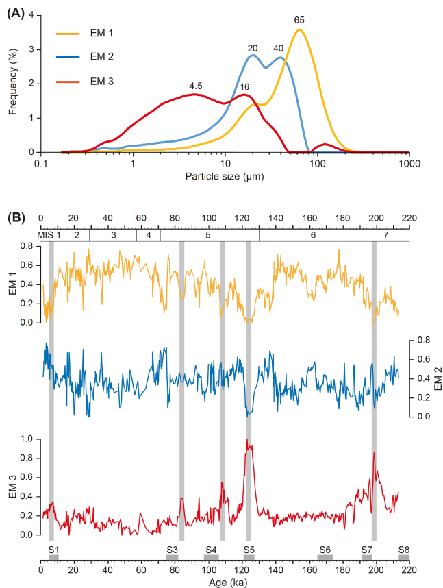
240 Figure 2: Results of endmember modelling on the grain size distribution of the terrigenous sediment fraction, core KL11. (A) Grain size distributions of the three endmembers. The respective modes are given in \mu\text{m} . (B) Loading patterns of the grain size endmembers. The main peak humid periods as inferred from EM3 are indicated by vertical grey bars. Marine isotope stages (MIS) are indicated at the top; horizontal bars at the bottom indicate sapropel layers S1–S8 in the eastern Mediterranean Sea associated with the African Humid Periods.
