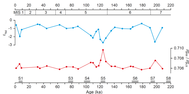
Figure 5: Strontium and neodymium isotope records of the bulk terrigenous fraction in core KL11. Analytical uncertainty on the isotope data is smaller than the size of the data points (see section 2.3). Marine isotope stages (MIS) are indicated at the top; horizontal bars at the bottom indicate sapropel layers S1–S8 in the eastern Mediterranean Sea associated with the African Humid Periods.
