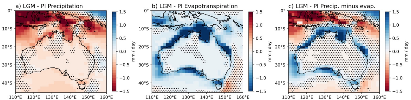
400 Figure 11: LGM – PI mean annual (a) precipitation (b) evapotranspiration and (b) P-E (in mm/day) simulated by the ensemble of CMIP5 and CMIP6 models over Australian region. Stippling indicates areas where less than 70% of ensemble members agree on the sign of the anomaly.
