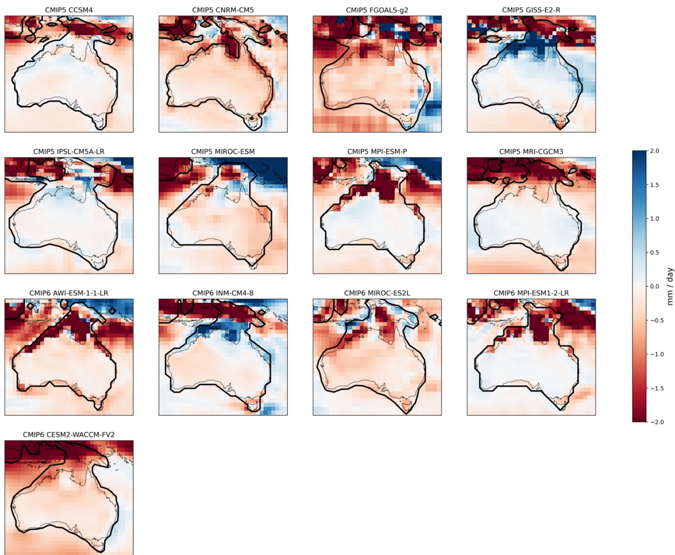
365 Figure 9: LGM – PI mean annual precipitation anomaly (mm/day) simulated by individual CMIP5 and CMIP6 models over the Australian domains. The thick black lines denote the coastlines in LGM prescribed in each model, and the thin black lines denoted the coastlines in piControl. 30% land area fraction was selected for plotting the LGM contours in models.
