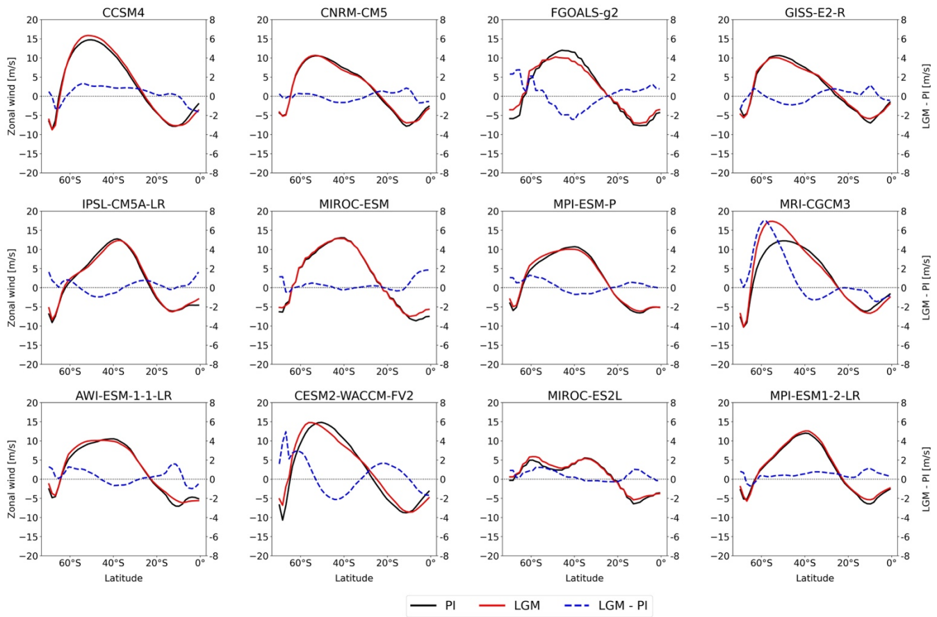
335 Figure 8: JJA zonal-mean zonal wind (m/s) at 850 hPa simulated by individual CMIP5 and CMIP6 models (except INM-CM4-8 model which provided only near-surface winds) averaged over Australian longitudes (defined as 110°E -160°E) for SH (0 to 70°S). PI in black colour and LGM in red colour, blue dashed line is LGM anomalies (LGM - PI). The LGM - PI zonal wind anomaly (m/s) for each model is displayed on a secondary y-axis. Zonal mean is calculated over all longitudes.
