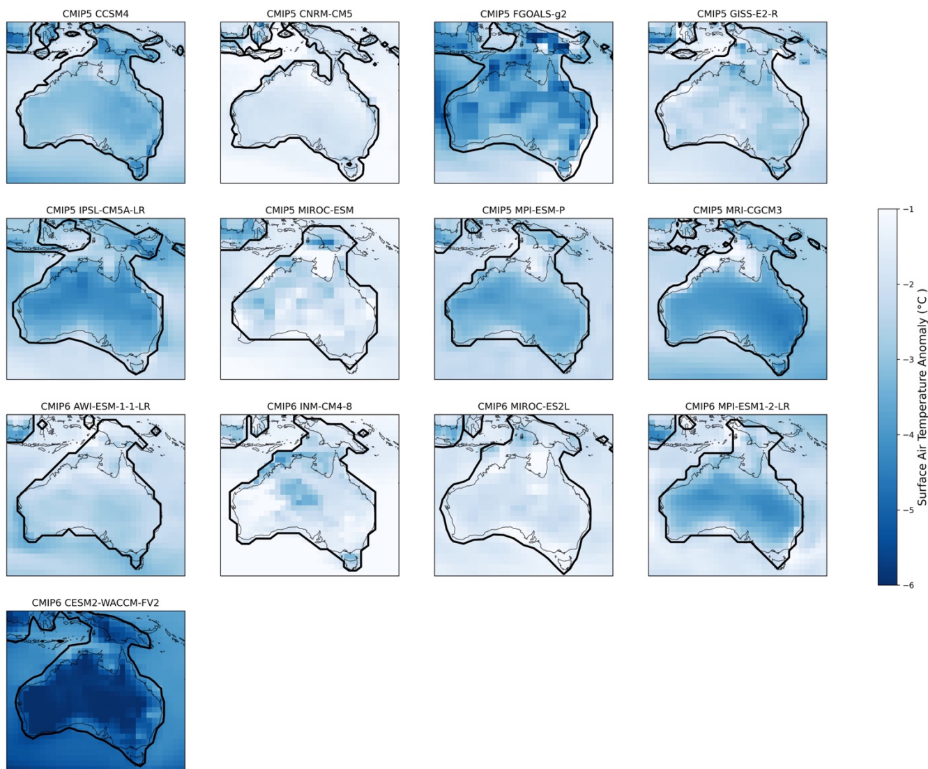
Figure 4: LGM - PI mean annual surface air temperature anomaly ( ^{\circ}\text{C} ) simulated by individual CMIP5 and CMIP6 models over Australian region. The thick black lines denote the coastlines in LGM prescribed in each model, and the thin black lines denoted the coastlines in piControl. 30% land area fraction was selected for plotting the LGM land mask contours in models.
