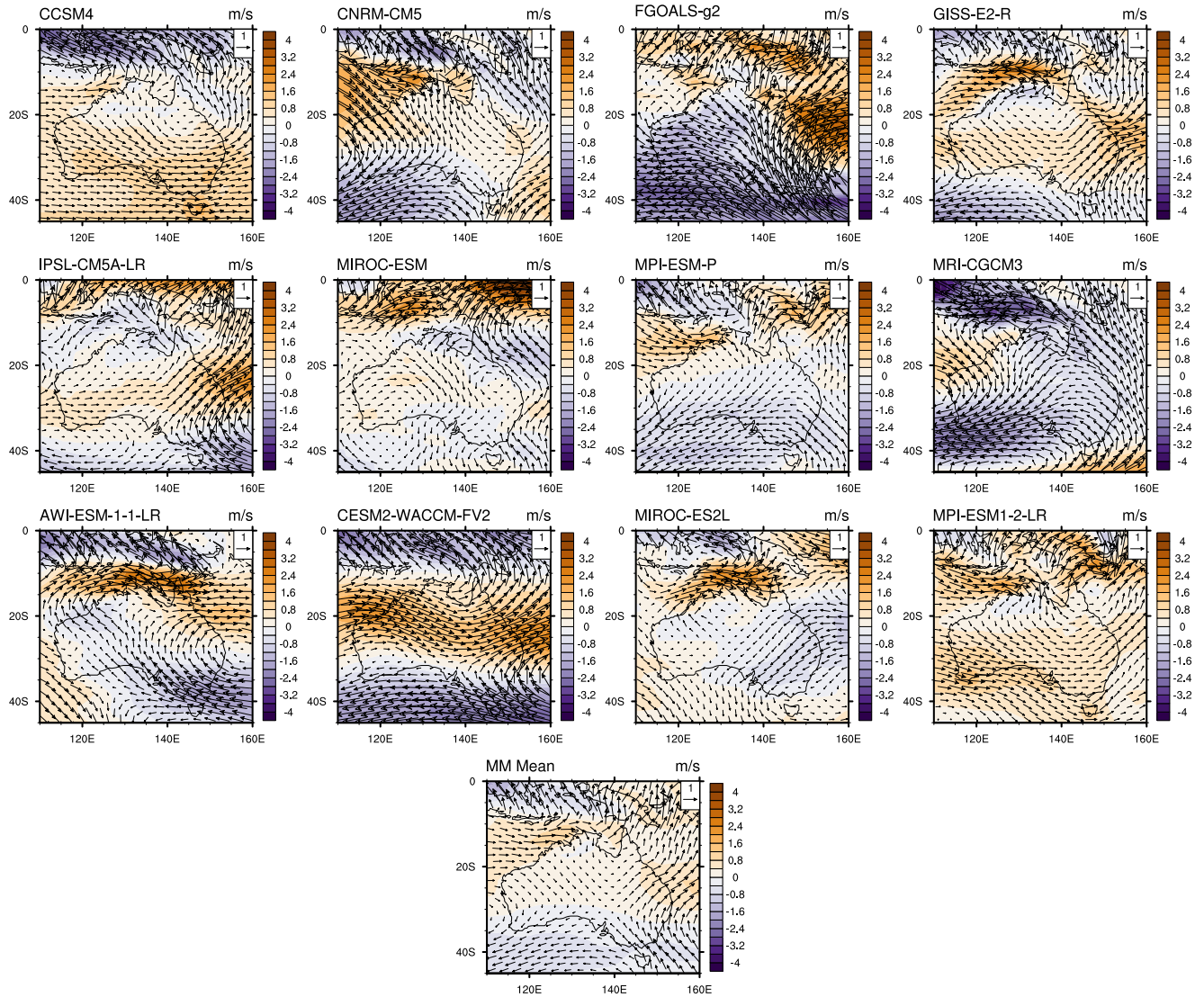
335 Figure 7: Change in JJA 850 hPa winds (Igm – piControl) for each model and multi-model mean over the Australian domains. Wind change is shown as vectors and zonal (westerly) wind change is shown as colored contours (m/s).
