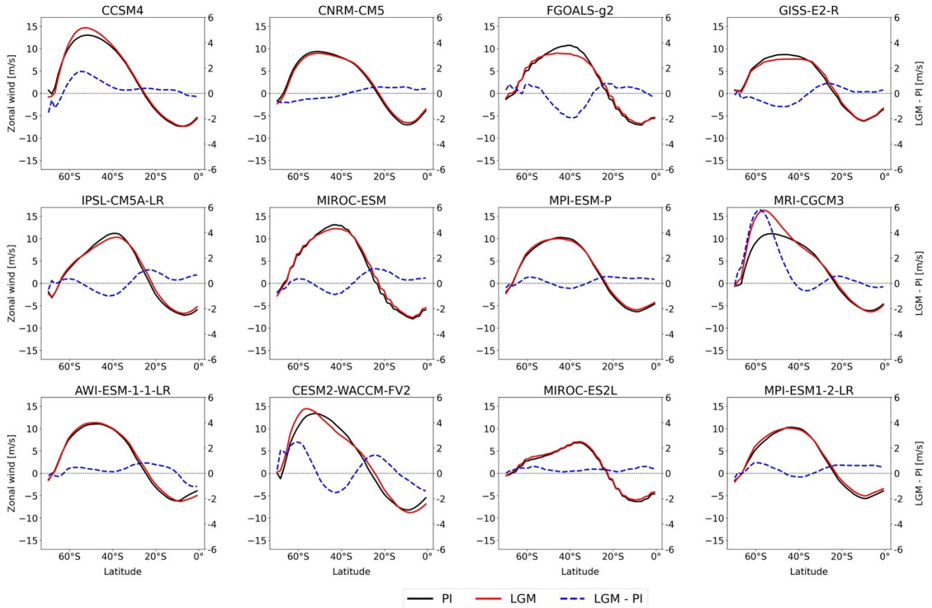
Figure 8: JJA Zonal-mean zonal wind (m/s) at 850 hPa simulated by individual CMIP5 and CMIP6 models (except INM-CM4-8 model which provided only near-surface winds) for SH (0 to 70°S). PI in black colour and LGM in red colour, blue dashed line is LGM anomalies (LGM - PI). The LGM - PI zonal wind anomaly (m/s) for each model is displayed on a secondary y-axis. Zonal mean is calculated over all longitudes.
