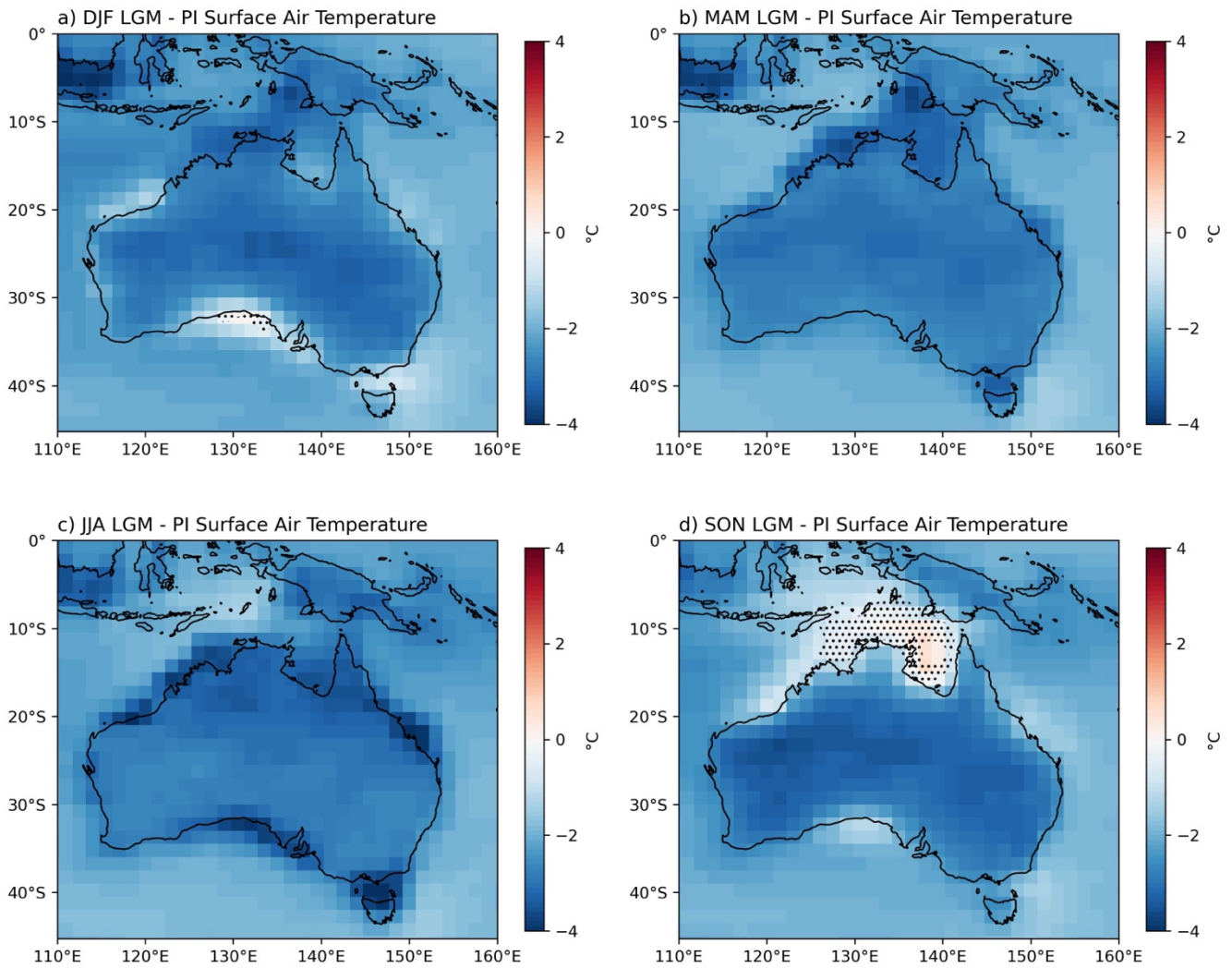
Figure 4: MMM seasonal anomalies for LGM - PI surface air temperatures (°C) simulated by the ensemble of CMIP5 and CMIP6 models for (a) DJF, (b) MAM, (c) JJA and (d) SON seasons over Australian region. Stippling indicates areas where less than 70% of ensemble members agree on the sign of the anomaly.
