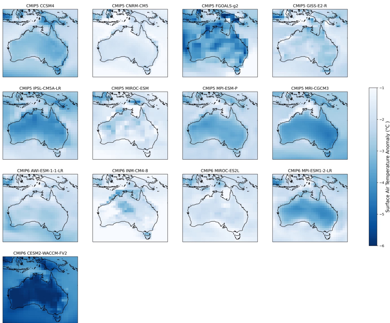
Figure 3: LGM - PI mean annual surface air temperature anomaly ( ^{\circ}\text{C} ) simulated by individual CMIP5 and CMIP6 models over Australian region.
