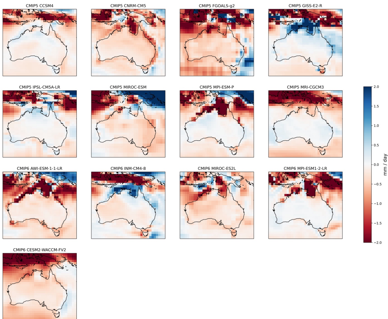
Figure 9: LGM – PI mean annual precipitation anomaly (mm/day) simulated by individual CMIP5 and CMIP6 models over the Australian domains.
