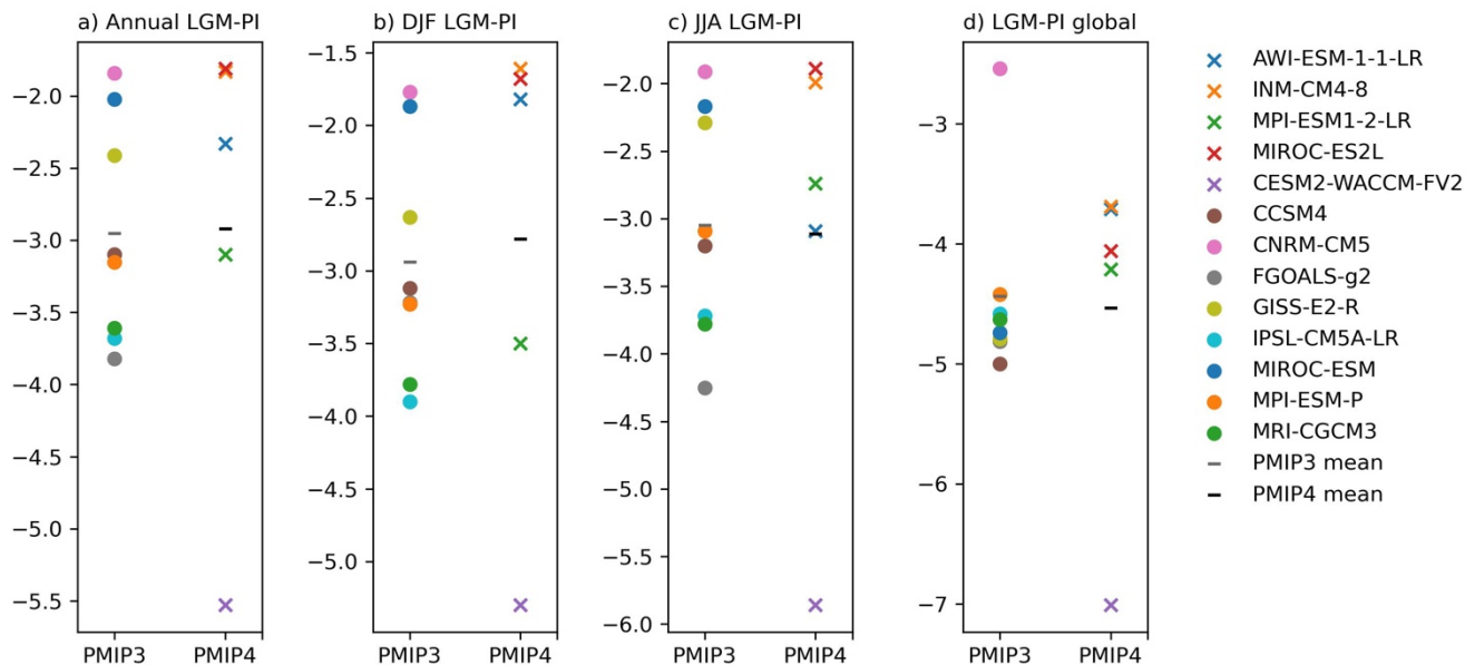
300 Figure 5: LGM – PI surface air temperature (tas) anomalies ( ^{\circ}\text{C} ) for (a) annual mean, (b) DJF, (c) JJA seasons over Australia (land areas within domain 0\text{-}45^{\circ}\text{S} , 110^{\circ}\text{E}\text{-}160^{\circ}\text{E} ), and (d) global annual mean surface air temperature anomalies ( ^{\circ}\text{C} ) for each CMIP5 and CMIP6 model and the multi-model mean (MMM).
