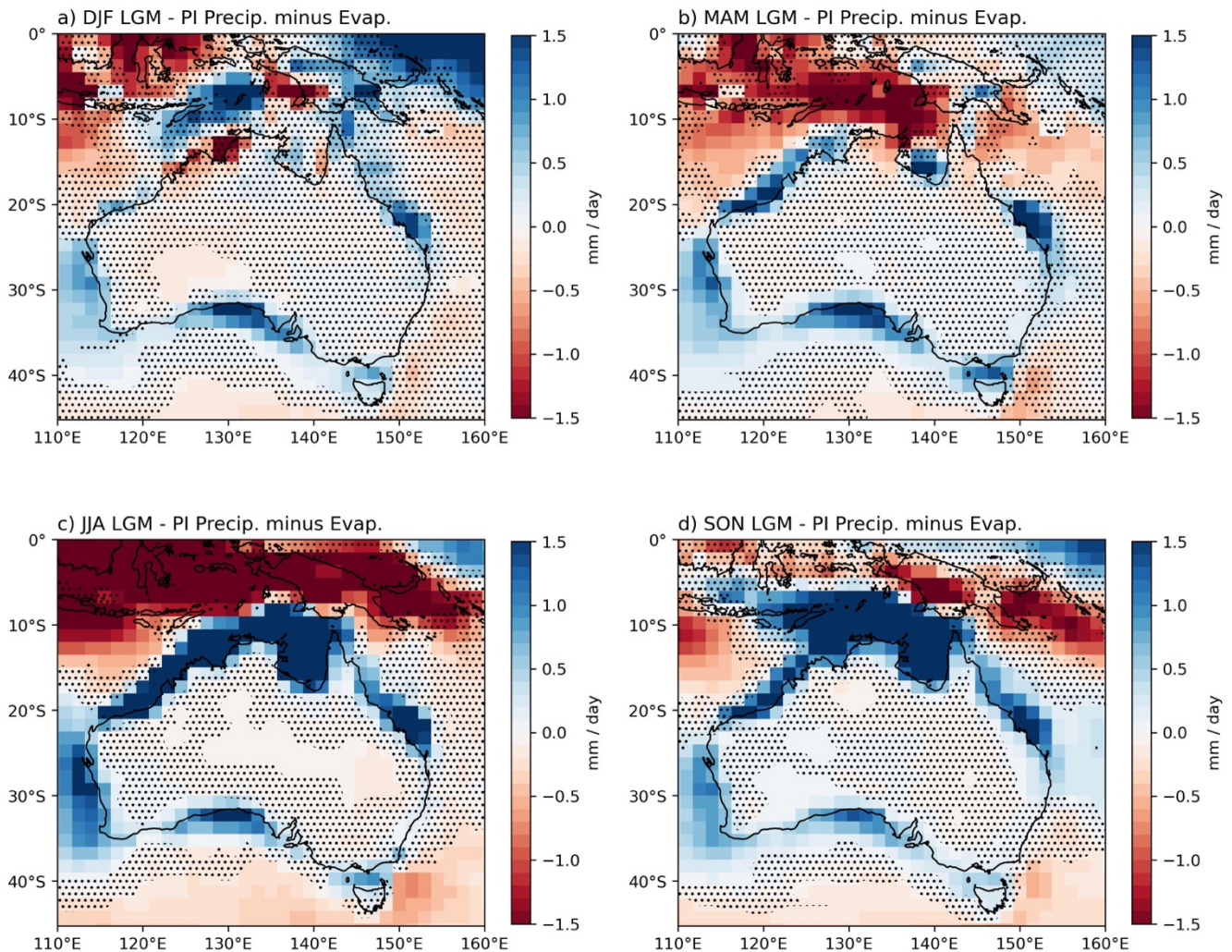
435 Figure 12: MMM seasonal anomalies for LGM – PI precipitation-evapotranspiration (P-E, mm/day) simulated by the ensemble of CMIP5 and CMIP6 models for (a) DJF, (b) MAM, (c) JJA and (d) SON seasons over Australian region. This can be compared with MMM seasonal precipitation shown in Figure 10 and MMM seasonal evapotranspiration shown in Supplementary Figure S4. Stippling indicates areas where less than 70% of ensemble members agree on the sign of the anomaly.
