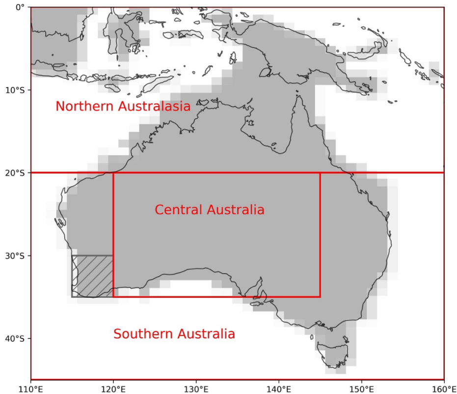
40 Figure 1: Classification of Northern Australasia, Central, and Southern Australia domains shown by red rectangles with modern day coastlines. The Central Australia domain is a subset of the larger Southern Australia domain. The south-west box for detecting JJA frontal precipitation that is most sensitive to westerlies is also indicated in hashes in the Southern Australia domain. The background grey shading indicates LGM land mask from CCSM4 model, plotted over modern coastlines.
