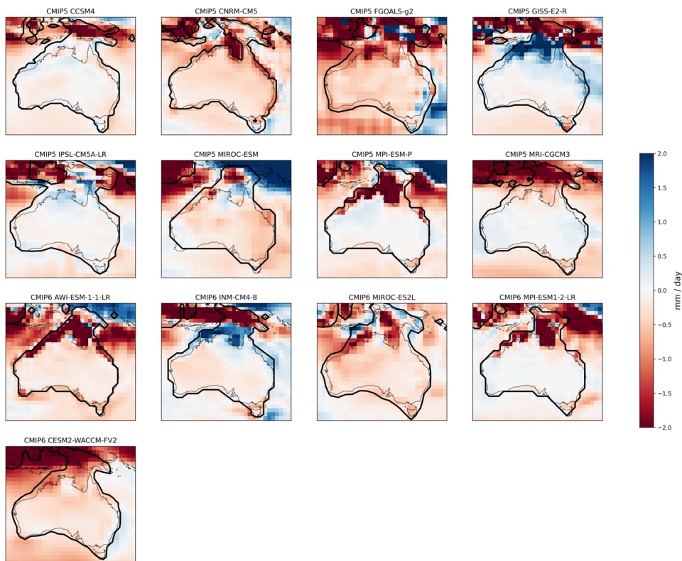
410 Figure 9: LGM – PI mean annual precipitation anomaly (mm/day) simulated by individual CMIP5 and CMIP6 models over the Australian domains. The thick black lines denote the coastlines in LGM prescribed in each model, and the thin black lines denoted the coastlines in piControl. 30% land area fraction was selected for plotting the LGM contours in models.
