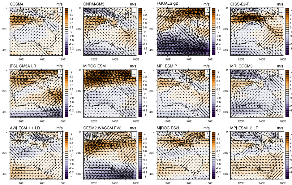
365 Figure 7: Change in mean annual 850 hPa winds (lgm – piControl) for each model and multi-model mean over the Australian domains. Wind change is shown as vectors and zonal (westerly) wind change is shown as colored contours (m/s).
