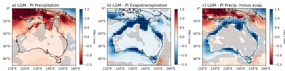
445 Figure 11: LGM – PI mean annual (a) precipitation (b) evapotranspiration and (b) P-E (in mm/day) simulated by the ensemble of CMIP5 and CMIP6 models over Australian region. Stippling indicates areas where less than 70% of ensemble members agree on the sign of the anomaly.
