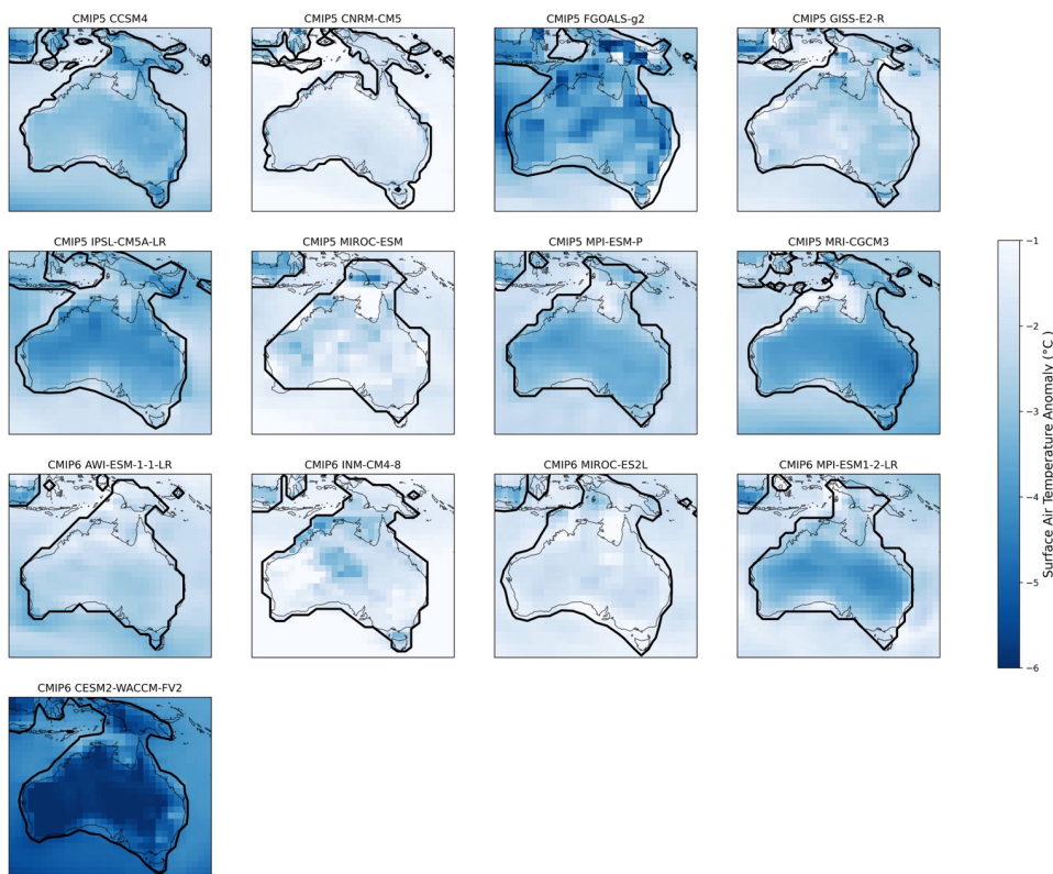
315 Figure 4: LGM - PI mean annual surface air temperature anomaly (°C) simulated by individual CMIP5 and CMIP6 models over Australian region. The thick black lines denote the coastlines in LGM prescribed in each model, and the thin black lines denoted the coastlines in piControl. 30% land area fraction was selected for plotting the LGM land mask contours in models.
