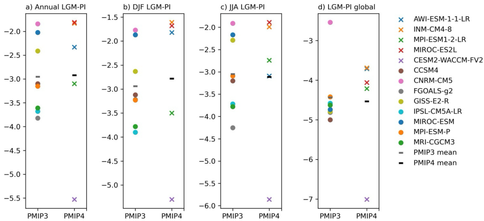
300 Figure 3: LGM – PI surface air temperature (tas) anomalies ( ^{\circ}\text{C} ) for (a) annual mean, (b) DJF, (c) JJA seasons over Australia (land areas within domain 0\text{-}45^{\circ}\text{S} , 110^{\circ}\text{E}\text{-}160^{\circ}\text{E} ), and (d) global annual mean surface air temperature anomalies ( ^{\circ}\text{C} ) for each PMIP3 and PMIP4 model and the multi-model mean (MMM).
