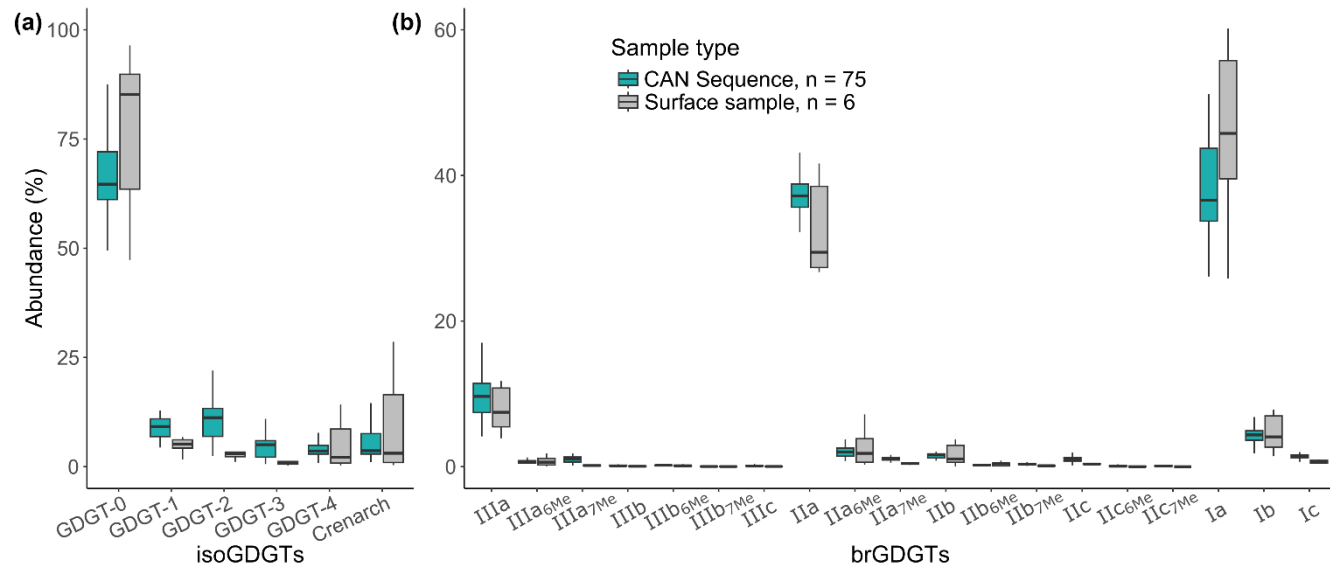
340 Figure 4: GDGT results: Fractional abundances (%) of (a) isoGDGT and (b) brGDGT compounds for the CAN02 sequence ( n = 75 , blue) and surface samples ( n = 6 , grey).
