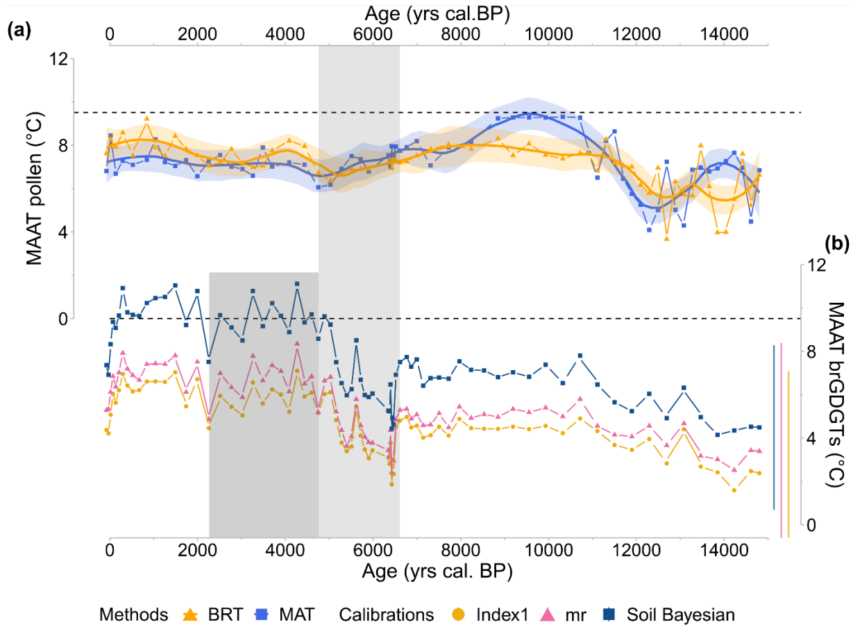
695 Figure 109: CAN02 temperature reconstructions (MAAT, in °C) obtained from (a) pollen assemblages obtained with using BRT (yellow triangles and yellow-curve) and MAT (blue squares and curve) methods based on the TEMPSCAND calibration. For both curves, the solid line corresponds to locally estimated scatterplot smoothing (loess) regression curves, the shaded area corresponds to its 95 % confidence interval, and (b) brGDGT signal for the 3-three selected soil calibrations: Soil Bayesian DCF, (dark blue squares and dark blue line, Dearing Crampton-Flood et al., 2020), Mrs DJ-mr (triangle symbol and light blue/pink line, De Jonge et al., 2014b) and Index1-DJ (yellow circle and red line, De Jonge et al., 2014b). On the right, lateral lines represent calibration errors (RMSE) are represented by lateral lines on the right side. Finally, the black dashed line corresponds to the modern MAAT at Canroute's modern MAAT. The time highlighted in light grey reveals a large fall in tetramethylated brGDGT abundance (6,600-4,700 cal. BP) and a shift in accumulation rate. The era shown in dark grey highlights the significant decrease in IR (4,700-2,300 cal. BP). The shaded period highlights the period of significant decrease in tetramethylated brGDGT abundance (6,600-5,000 cal. BP) and a shift in accumulation rate.
