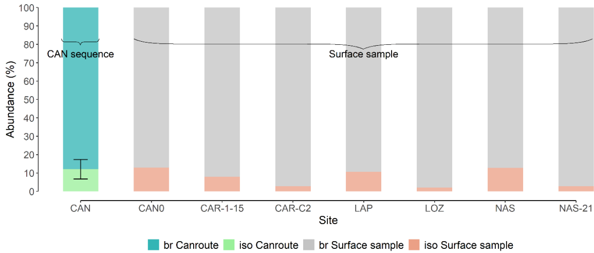
805 Figure C: Relative abundance (%) of isoGDGTs (pink) and brGDGTs (grey) for surface samples and average relative abundance of isoGDGTs (green) and brGDGTs (blue) in the CAN core (n = 75).
