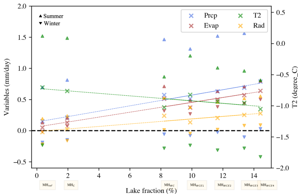
290 Figure 5: Statistical relationship between regionally averaged hydroclimate variables anomaly and grid lake fraction over Northern Africa (20°W–40°E, 0–35°N) for MH lake experiment anomalies (relative to PI_{ref} ) on the annual (cross), JJAS (upward triangle), and JAM (downward triangle) averages. The hydroclimatic variables include precipitation (Prpc [mm/day]), evaporation (Evap [mm/day]), 2 m air temperature (T2 [°C]), and radiation (Rad [mm/day], downward as positive). The p-value is <0.05 for all relationships.
