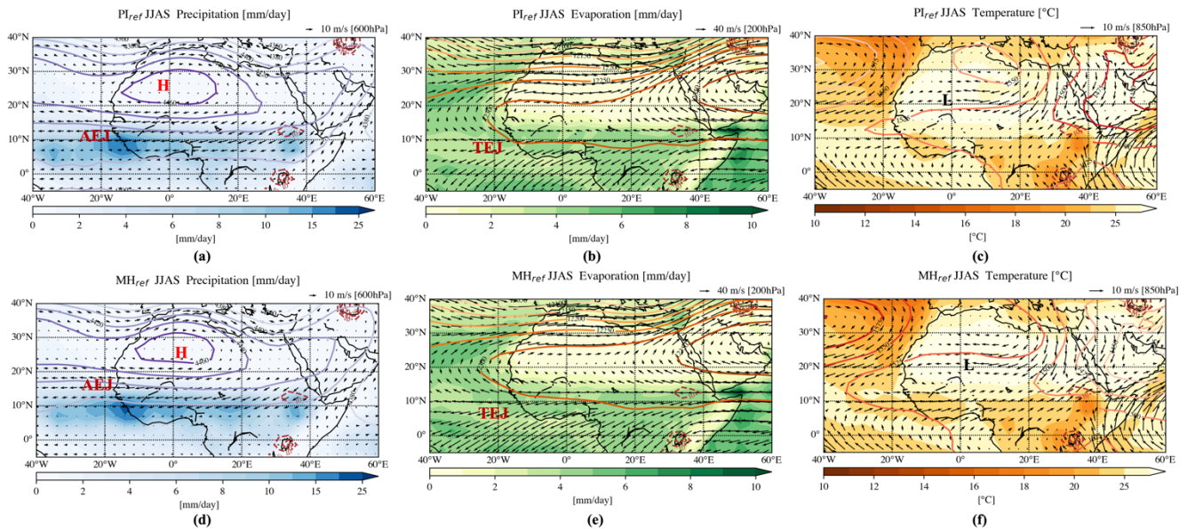
205 Figure 2: Simulated climatological precipitation and temperature responses for the Pre-industrial (PI) and MH reference experiments during the summer season (June-July-August-September, JJAS). For the PI experiment, (a) is the precipitation with 600 hPa wind (arrow) geopotential height (counters), (b) is the evaporation with 200 hPa wind and geopotential height, and (c) is the surface temperature with 850 hPa wind and geopotential height. Subplots (d), (e), and (f) are the same as (a), (b) and (c), respectively, but for the MH experiment. For (a–f), lake fraction (%) contours of the respective lake sensitivity experiment are shown with red dashed lines and the respective reference scale for the arrow is shown at the right top of each panel. The corresponding high pressure lines and the respective reference system, Africa Easterly Jet, and Tropical Easterly Jet are marked as ‘H’, ‘L’, ‘AEJ’ and ‘TEJ’, respectively. 210
