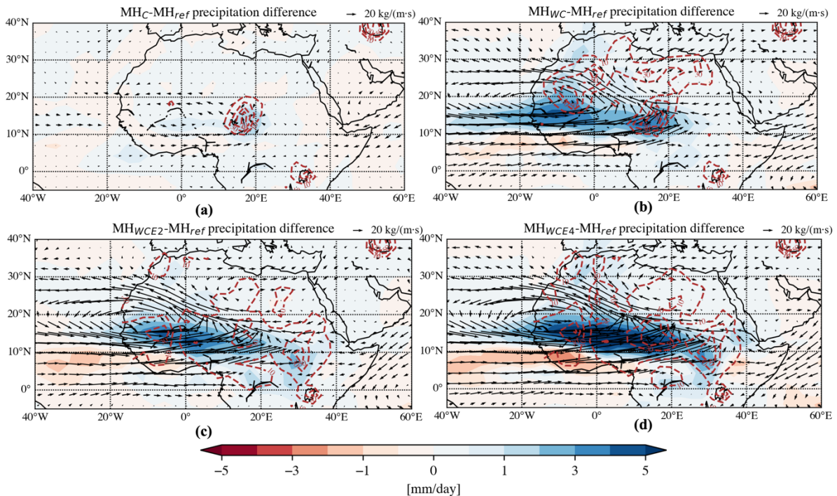
230 Figure 3: Anomalies relative to MH_{ref} in the simulated MH climatological summer mean (JJAS) precipitation (shades) and integrated vapor transportation (arrows) for (a) MH_C , (b) MH_{WC} , and (c) MH_{WCE2} and MH_{WCE4} , respectively. For (a)–(d), the lake fraction (%) contours of the respective lake sensitivity experiment are shown as red dashed lines (contour spacing: 10%, 30%, 50%, 70%, 100%), and the respective reference scale for the arrow is shown at the right top of each panel.
