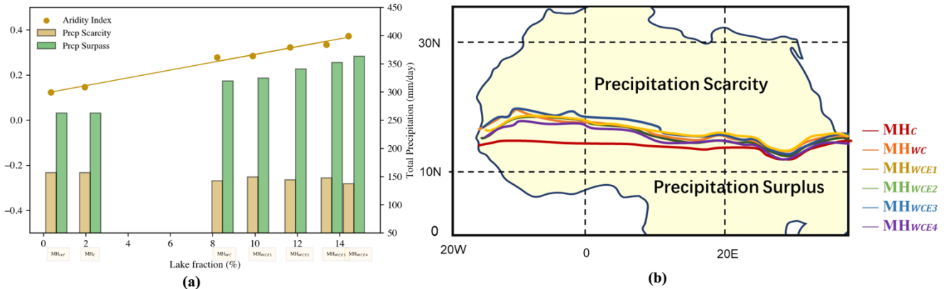
Figure 6: (a) Budyko Aridity index anomaly between PI_{ref} and MH simulations (left y-axis; unitless) with different averaged grid lake fractions and total precipitation scarcity and surplus amounts (brown and green bars, respectively; mm/d) corresponding to the right y-axis. All the variables are climatological mean annual values. (b) Border between regions of precipitation scarcity zones and precipitation surplus zones for all the MH experiments.
