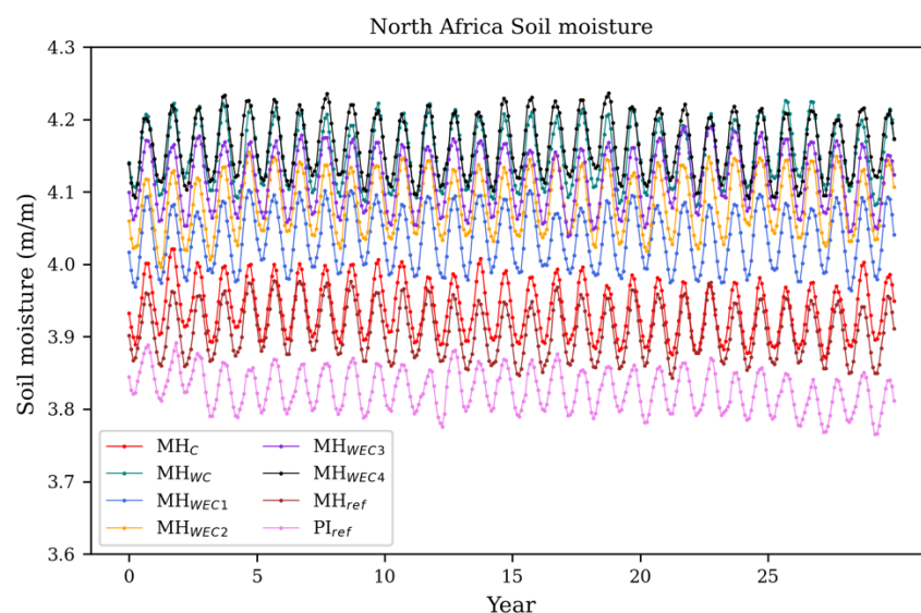
Figure R1. North African monthly soil moisture time series for all the experiments during the calculation period.
