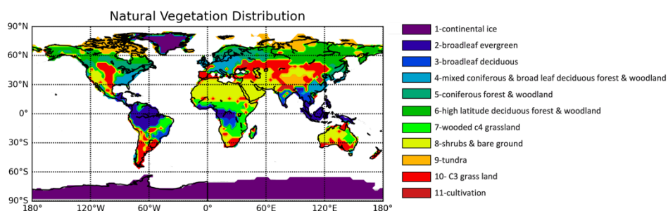
Figure R0. Vegetation type distribution map for all the experiments.
