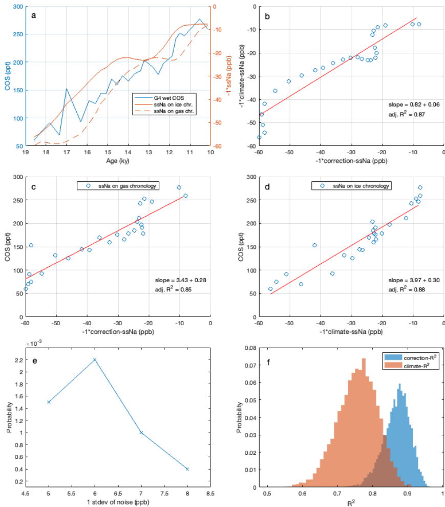
1030 Figure A10. a) The corrected COS (G4) during the deglaciation (left y-axis), and the correction-ssNa and climate-ssNa (right y-axis). b) The regression of the correction-ssNa (x-axis) versus the climate-ssNa (y-axis). c) The regression of the correction-ssNa versus COS. d) The regression of the climate-ssNa versus COS. e) The conditional probability of the climate- R^2 being higher than the correction- R^2 , given the climate- R^2 is at least 0.88, at different levels of random noise. f) The PDFs of the correction- R^2 and the climate- R^2 at 6 ppb noise.
