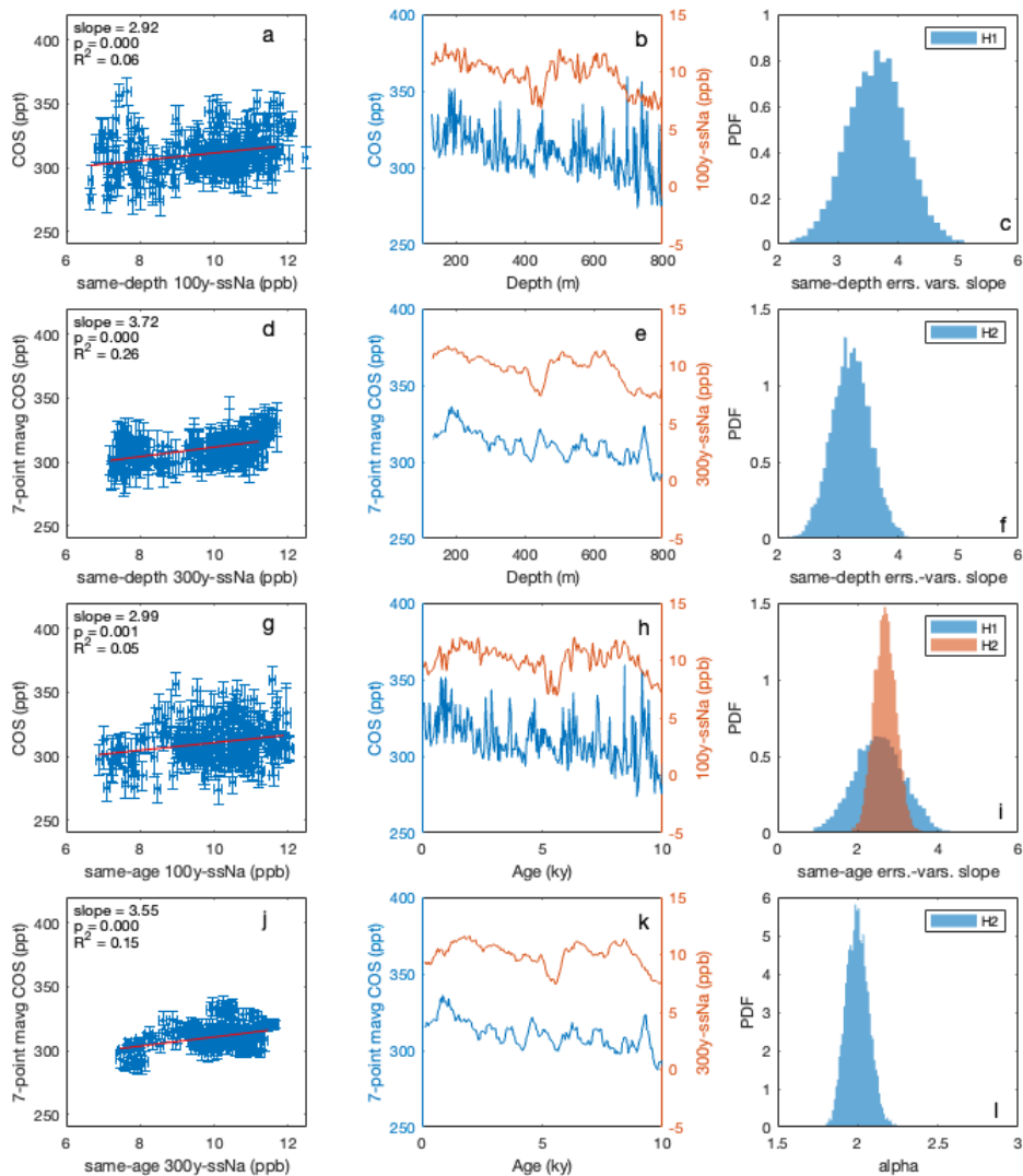
Figure A7. Same-depth and same-age correlations between ssNa and COS for different Holocene (< 800 m) analysis scenarios. 1005 a) H1: Same-depth 100-y ssNa versus COS with least-squares regression results. b) The data from (a) shown versus depth. c) Errors-in-variables PDF for (a). d) H2: Same-depth 300-y ssNa versus 7-point moving average COS with least-squares regression results. e) The data from (d) shown versus depth. f) Errors-in-variables PDF for (d). g) H1: Same-age 100-y ssNa versus COS with least-squares regression results. h) The data from (g) shown versus age. i) Errors-in-variables PDFs for (g) and (j). j) H2: Same-age 300-y ssNa versus COS with least-squares regression results. k) The data from (j) shown versus age. 1010 l) Errors-in-variables PDF for the H2 alpha parameter.
