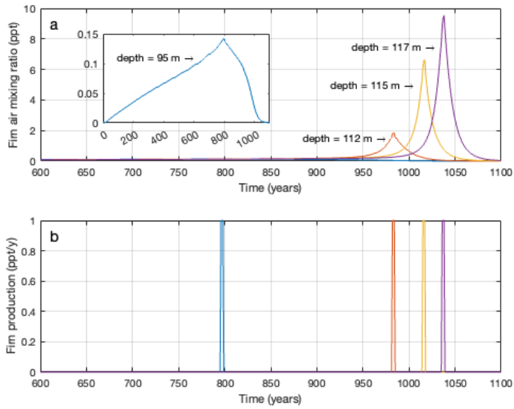
Figure 6. Modeled trace gas production in the South Pole firn from an impurity layer. a) Firm air trace gas mixing ratio (y-axis) vs time (x-axis) at 95 m (blue), 112 m (red), 115 m (yellow), and 117 m (purple). The 95 m profile is shown in the inset because the excess gas peak at this depth is not visible at the scaling of the parent plot. Note that the gas mixing ratio at any given depth peaks when the production occurs at that depth. b) Gas production vs. time at the same depths as (a).
