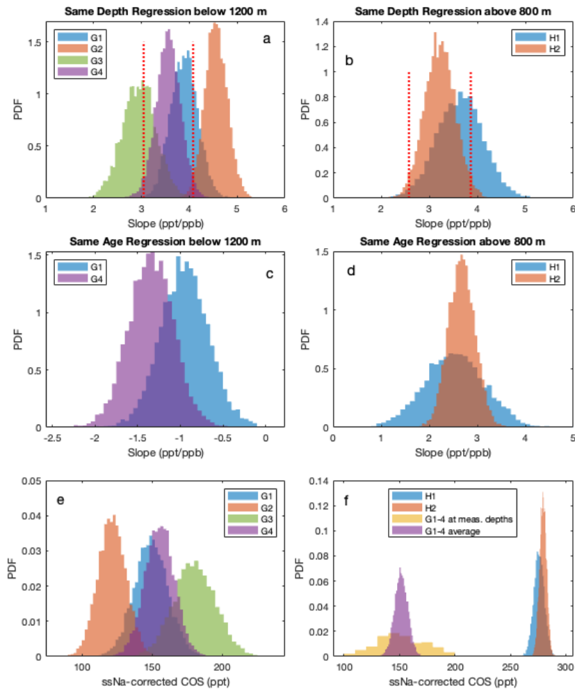
915 Figure 3. a) PDFs of the same-depth errors-in-variables regressions for the glacial period (below 1200 m) dry extraction COS measurements under four different analysis scenarios (section 3.1). b) Same as (a) for the two Holocene (above 800 m) scenarios. In (a) and (b), the \pm 2\sigma (95%) confidence intervals (red dashed lines) for the G4 and H2 regressions are shown to demonstrate the high statistical significance (being different from zero) of the PDFs for all scenarios. c-d) Same as (a) and (b) but for the same-age errors-in-variables linear regressions. e) Distributions of all dry COS measurements from 52 – 23 ky after 920 correction with ssNa under G1 through G4 scenarios. f) Distributions of dry COS measurements after correction with ssNa under H1 (blue) and H2 (red) scenarios. For comparison, distributions of the average across G1 through G4 (purple, n=8000) and the average of all scenarios at discrete depths (yellow, n=177) are also shown. During the LGM, the ssNa-corrected wet COS measurements reach lower levels than what is displayed here for the 52 – 23 ky period (Fig. 4b).
