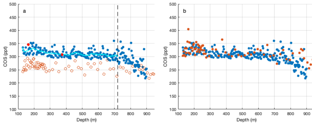
965 Figure A2. The dry (blue) and wet (red) extraction based COS measurements from the top 950 m of the SPC14 ice core. a) The wet extraction measurements from above 720 m (shallower than vertical dashed line) are smoothed before being used to determine the solubility correction parameters (Fig. A3). The smooth dry extraction record (cyan line) is linearly interpolated to wet extraction measurement depths to estimate COS_{dry} in Eq. (3). Solid red circles denote two outlier wet extraction measurements, which were not included in determination of C_3 and C_4 in Eq. (3). b) Solubility corrected wet extraction 970 measurements (red) versus the dry extraction measurements from (a).
