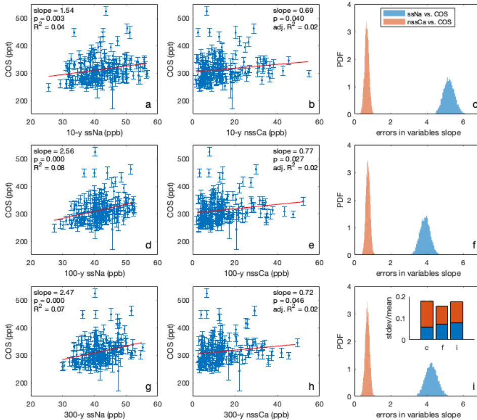
980 Figure A4. Same-depth regression analyses between ssNa and nssCa versus dry extraction COS below 1200 m. a) 10-y ssNa versus COS with least-squares regression results. b) 10-y nssCa versus COS with least-squares regression results. c) Errors-in-variables regression results for a and b. d-e) Same as (a) and (b) but for 100-y ssNa and nssCa. f) Errors-in-variables regression results for (d) and (e). g-h) Same as (a) and (b) but for 300-y ssNa and nssCa. i) Errors-in-variables regression results for g and h. The inset displays stdev/mean (a significance metric) for the PDFs shown in c, f, and i.
