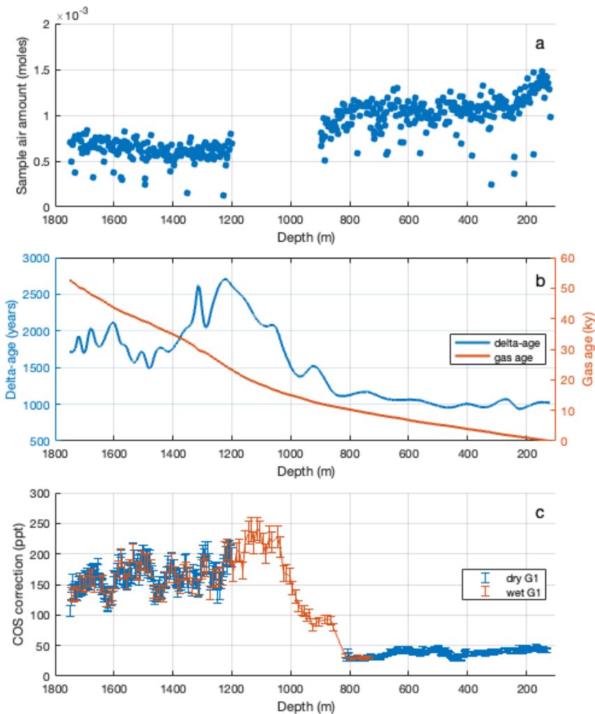
Figure A1. a) Amount of air extracted from the SPC14 ice core samples used for COS analysis with dry extraction. The low 945 outliers are due to smaller ice samples that were commonly half as long. Average amount of air extracted from samples below 1200 m is lower primarily because of a drop in extraction efficiency of dry extraction for full clathrate ice because of the smaller size of clathrates with respect to the bubbles. The presumed bubble-clathrate transition zone from 900 m to 1200 m was not analyzed with dry extraction because of expected experimental artifacts. The actual start depth of BCTZ is around 800 m as evidenced by the downcore decrease in sample air amount. b) The delta-age (left y-axis) and gas age (right y-axis) for 950 the SPC14 ice core (Epifanio et al., 2020). c) The correction applied to the COS measurements under the G1 scenario.
