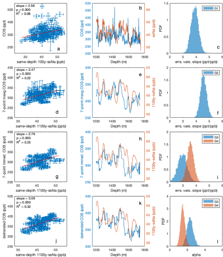
975 Figure A5. Same-depth correlations between ssNa and COS for different glacial period (>1200 m) analysis scenarios. a) G1: 100-y ssNa versus COS with least-squares regression results (same as Fig. 2c). b) Data from (a) vs. depth. c) Errors-in-variables PDF for (a) (same as in Fig. A4f). d) G2: 1100-y ssNa versus 7-point moving average COS with least-squares regression results. e) Data from (d) vs. depth. f) Errors-in-variables PDF for (d). g) G3: 1100-y ssNa versus 7-point moving median COS with least-squares regression results. h) Data from (g) vs. depth. i) Errors-in-variables PDFs for (g) and (j). j) G4: 1100-y ssNa versus 7-point moving median COS detrended for same-age correlation with ssNa, shown with least-squares regression results. 980 k) Data from (j) vs. depth. l) Errors-in-variables PDFs for the G3 and G4 alpha parameters.
