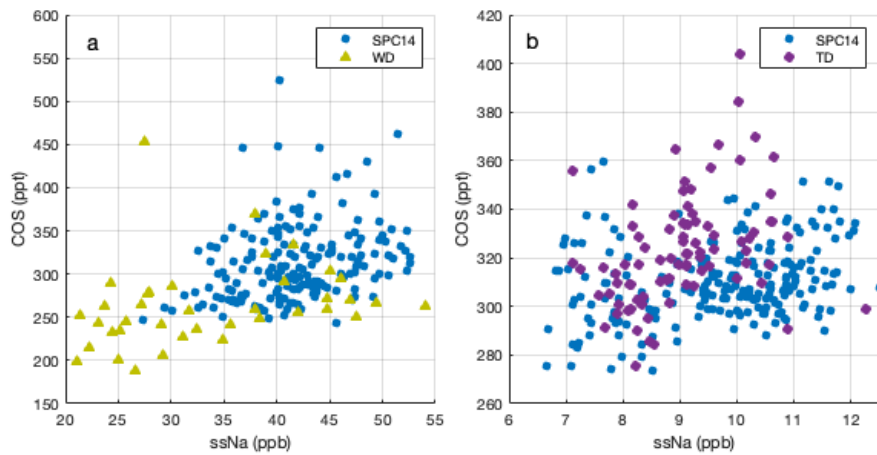
1025 Figure A11. 100-y ssNa vs. measured COS levels. ssNa for the WD and TD ice cores is calculated using \text{Na}^+ and \text{Ca}^{2+} measurements from the respective cores (McConnell et al., 2017; Steig et al., 2000). a) The data used in the G1 scenario (Fig. 2c) for SPC14 is compared with all data from WD older than 11 ky. b) The data used in the H1 scenario (Fig. 2d) for SPC14 is compared with TD data younger than 8 ky.
