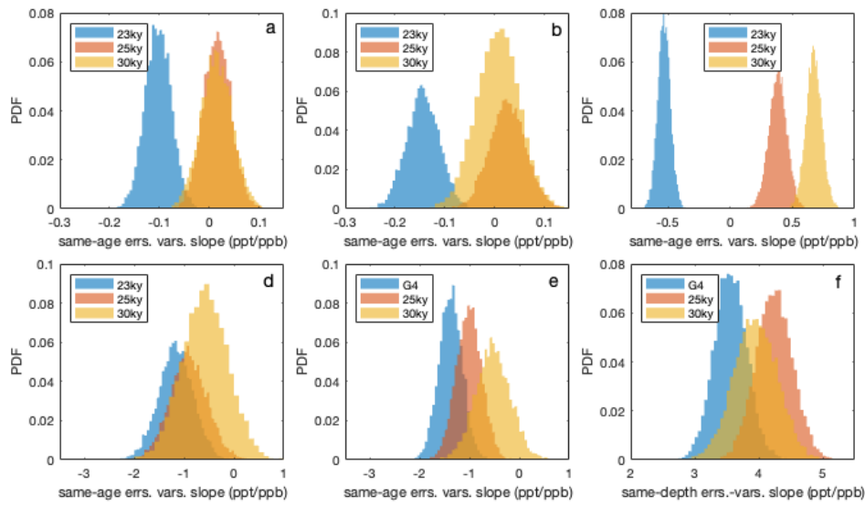
1010 Figure A9. a) The errors-in-variables PDFs for the regression of the inverted 100-y ssNa interpolated to the SPC14 gas chronology at annual resolution versus the 100-y ssNa record on ice chronology at annual resolution during three periods (>23 ky, >25 ky, and >30 ky). b) Same as (a) except using 1100-y ssNa. c) Same as (b) but at the ages of the COS measurements. d) The errors-in-variables PDFs for the regression of the mean of the G4 corrected COS from Fig. 4b with the 1100-y ssNa. e) The same-age results from a repeat of the G4 regression (Fig. 3c) for different temporal cut-offs. f) The same-depth results 1015 from a repeat of the G4 regression (Fig. 3a) for different temporal cut-offs.
