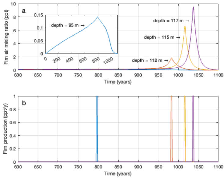
930 Figure 6. Modeled trace gas production in the South Pole firn from an impurity layer. a) Firn air trace gas mixing ratio (y-axis) vs time (x-axis) at 95 m (blue), 112 m (red), 115 m (yellow), and 117 m (purple). The 95 m profile is shown in the inset because the excess gas peak at this depth is not visible at the scaling of the parent plot. Note that the gas mixing ratio at any given depth peaks when the production occurs at that depth. b) Gas production vs. time at the same depths as (a).
