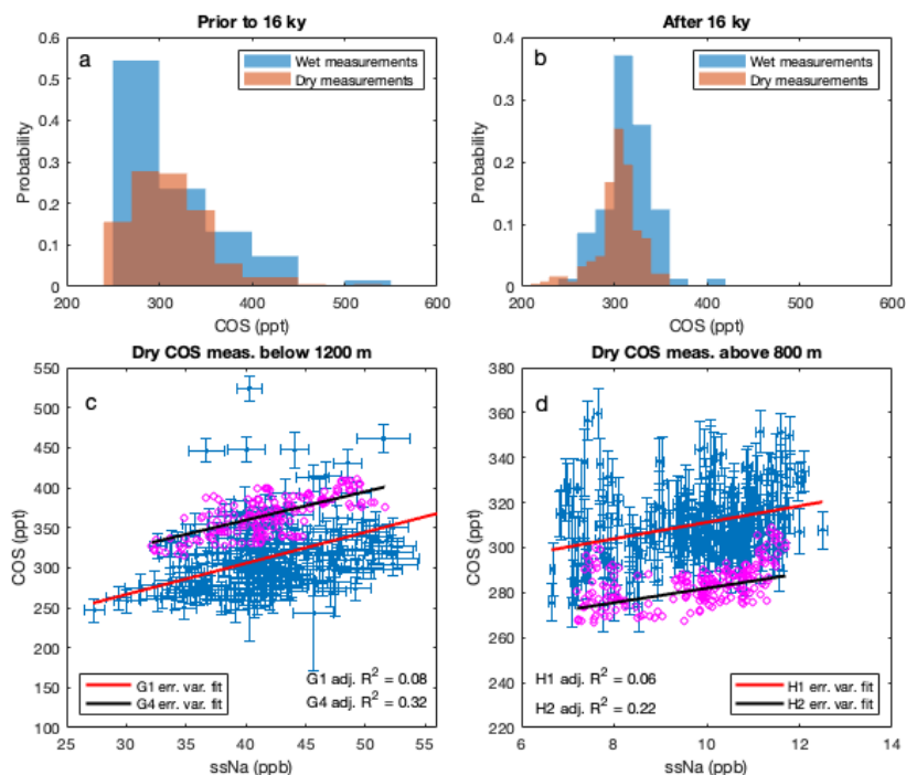
895 Figure 2: a) Distribution of SPC14 COS measurements before 16 ky. The dry measurements shown here are the basis for the regressions shown in (c). b) Distribution of SPC14 COS measurements after 16 ky. The dry measurements shown here are the basis for the regressions shown in (d). c) The ssNa vs. dry COS measurements for the glacial period (below 1200 m) used in the G1 (blue error bars) and the G4 (magenta circles) scenarios (Table 2). The linear fits to errors-in-variables regressions are calculated using the mean slopes and intercepts for G1 and G4 (also see Figs. A5 and A6). d) Same as (c) but for the Holocene 900 (above 800 m) H1 and H2 scenarios (also see Fig. A7).
