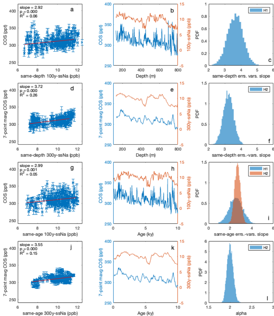
Figure A7. Same-depth and same-age correlations between ssNa and COS for different Holocene (< 800 m) analysis scenarios. a) H1: Same-depth 100-y ssNa versus COS with least-squares regression results. b) The data from (a) shown versus depth. c) Errors-in-variables PDF for (a). d) H2: Same-depth 300-y ssNa versus 7-point moving average COS with least-squares regression results. e) The data from (d) shown versus depth. f) Errors-in-variables PDF for (d). g) H1: Same-age 100-y ssNa versus COS with least-squares regression results. h) The data from (g) shown versus age. i) Errors-in-variables PDFs for (g) and (j). j) H2: Same-age 300-y ssNa versus COS with least-squares regression results. k) The data from (j) shown versus age. l) Errors-in-variables PDF for the H2 alpha parameter.
