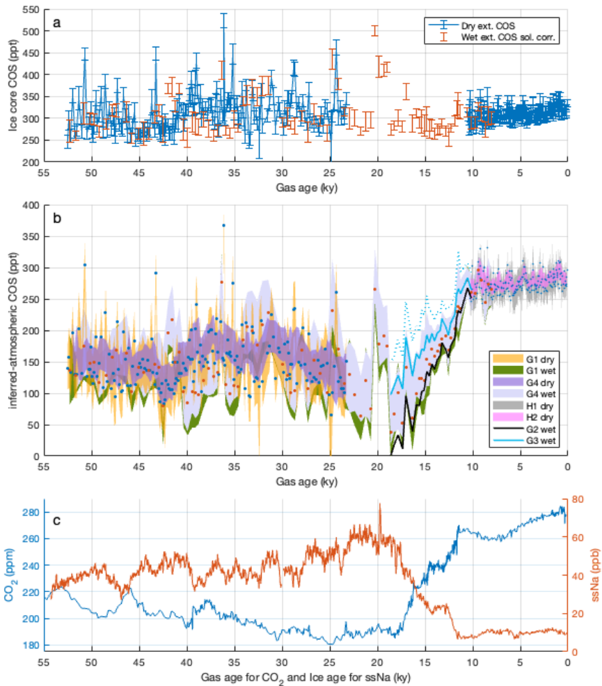
Figure 4. a) The SPC14 COS measurements from Fig. 1a with \pm 1\sigma measurement errors. b) The inferred (ssNa-corrected) atmospheric COS record. The filled markers denote the individual data points corrected with G1 and H1 scenarios for the dry (blue) and G1 for the wet (red) measurements. The colored bands (see legend) denote posterior \pm 2\sigma ranges (section 2.4) for all analysis scenarios shown in Fig. 3a-d; the full PDFs for G1 through G4 and H1 and H2 scenarios are shown in Fig. 3e, f. The wet G1 \pm 2\sigma range is mostly masked by the wet G4 \pm 2\sigma range. For clarity, only the posterior means (lines) through the deglaciation are shown for the wet G2 and G3. The dashed blue line is the +2\sigma range for the G3 scenario, representing an upper limit albeit at very low probability. c) A composite Antarctic ice core CO 2 record (blue – left y-axis) and the 100y-smooth ssNa record from the SPC14 ice core (red – right y-axis) versus gas age and ice age, respectively (Bereiter et al., 2015; Winski et al., 2021).
