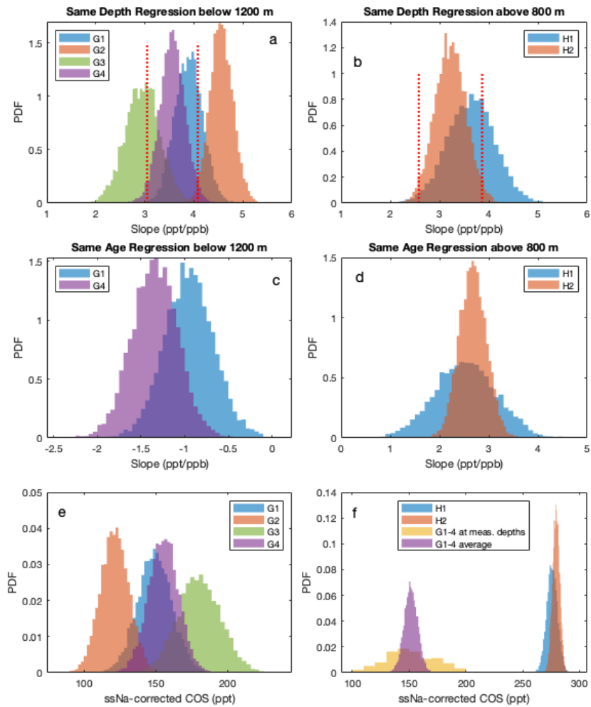
Figure 3. a) PDFs of the same-depth errors-in-variables regressions for the glacial period (below 1200 m) dry extraction COS measurements under four different analysis scenarios (section 3.1). b) Same as (a) for the two Holocene (above 800 m) scenarios. In (a) and (b), the \pm 2\sigma (95%) confidence intervals (red dashed lines) for the G4 and H2 regressions are shown to demonstrate the high statistical significance (being different from zero) of the PDFs for all scenarios. c-d) Same as (a) and (b) but for the same-age errors-in-variables linear regressions. e) Distributions of all dry COS measurements from 52 – 23 ky after correction with ssNa under G1 through G4 scenarios. f) Distributions of dry COS measurements after correction with ssNa under H1 (blue) and H2 (red) scenarios. For comparison, distributions of the average across G1 through G4 (purple, n=8000) and the average of all scenarios at discrete depths (yellow, n=177) are also shown. During the LGM, the ssNa-corrected wet COS measurements reach lower levels than what is displayed here for the 52 – 23 ky period (Fig. 4b).
