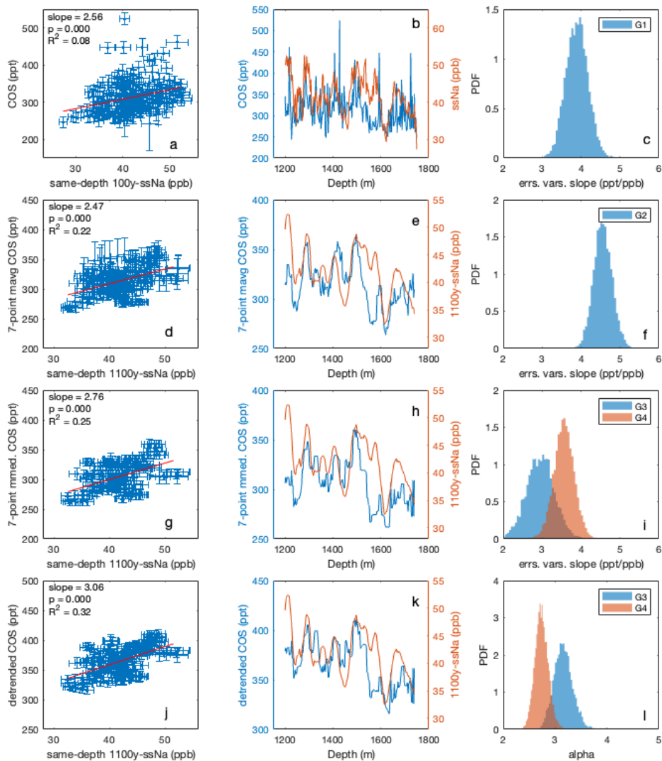
875 Figure A5. Same-depth correlations between ssNa and COS for different glacial period (>1200 m) analysis scenarios. a) G1: 100-y ssNa versus COS with least-squares regression results (same as Fig. 2c). b) Data from (a) vs. depth. c) Errors-in-variables PDF for (a) (same as in Fig. A4f). d) G2: 1100-y ssNa versus 7-point moving average COS with least-squares regression results. e) Data from (d) vs. depth. f) Errors-in-variables PDF for (d). g) G3: 1100-y ssNa versus 7-point moving median COS with least-squares regression results. h) Data from (g) vs. depth. i) Errors-in-variables PDFs for (g) and (j). j) G4: 1100-y ssNa versus 7-point moving median COS detrended for same-age correlation with ssNa, shown with least-squares regression results. 880 k) Data from (j) vs. depth. l) Errors-in-variables PDFs for the G3 and G4 alpha parameters.
