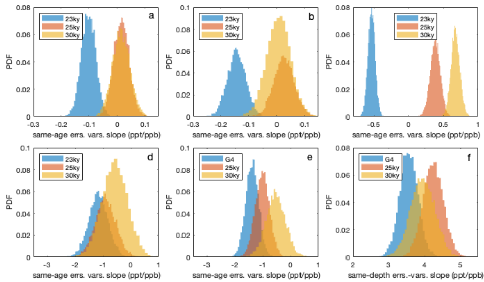
910 Figure A9. a) The errors-in-variables PDFs for the regression of the inverted 100-y ssNa interpolated to the SPC14 gas chronology at annual resolution versus the 100-y ssNa record on ice chronology at annual resolution during three periods (>23 ky, >25 ky, and >30 ky). b) Same as (a) except using 1100-y ssNa. c) Same as (b) but at the ages of the COS measurements. d) The errors-in-variables PDFs for the regression of the mean of the G4 corrected COS from Fig. 4b with the 1100-y ssNa. e) The same-age results from a repeat of the G4 regression (Fig. 3c) for different temporal cut-offs. f) The same-depth results 915 from a repeat of the G4 regression (Fig. 3a) for different temporal cut-offs.
