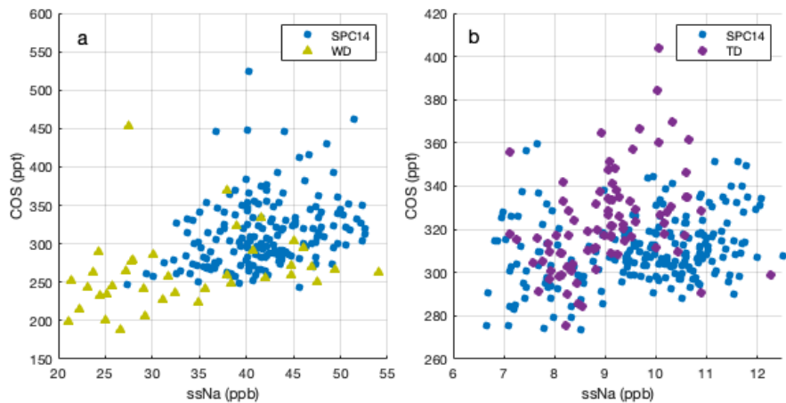
925 Figure A11. 100-y ssNa vs. measured COS levels. ssNa for the WD and TD ice cores is calculated using \text{Na}^+ and \text{Ca}^{2+} measurements from the respective cores (McConnell et al., 2017; Steig et al., 2000). a) The data used in the G1 scenario (Fig. 2c) for SPC14 is compared with all data from WD older than 11 ky. b) The data used in the H1 scenario (Fig. 2d) for SPC14 is compared with TD data younger than 8 ky.
