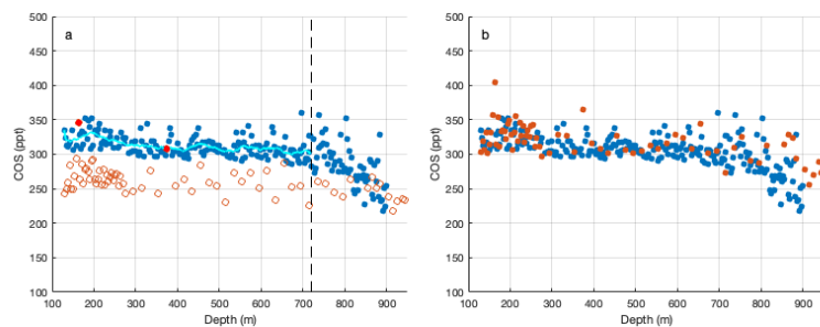
Figure A2. The dry (blue) and wet (red) extraction based COS measurements from the top 950 m of the SPC14 ice core. a)
