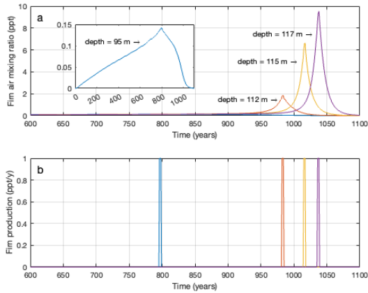
1115 Figure 6. Modeled trace gas production in the South Pole firn from an impurity layer. a) Firn air trace gas mixing ratio (y-axis) vs time (x-axis) at 95 m (blue), 112 m (red), 115 m (yellow), and 117 m (purple). The 95 m profile is shown in the inset because the excess gas peak at this depth is not visible at the scaling of the parent plot. Note that the gas mixing ratio at any given depth peaks when the production occurs at that depth. b) Gas production vs. time at the same depths as (a).
