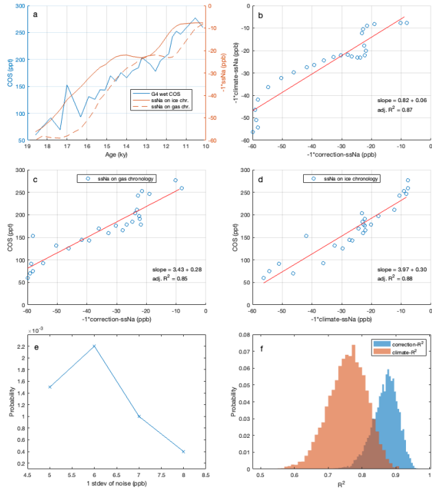
1210 Figure A10. a) The corrected COS (G4) during the deglaciation (left y-axis), and the correction-ssNa and climate-ssNa (right y-axis). b) The regression of the correction-ssNa (x-axis) versus the climate-ssNa (y-axis). c) The regression of the correction-ssNa versus COS. d) The regression of the climate-ssNa versus COS. e) The conditional probability of the climate- R^2 being higher than the correction- R^2 , given the climate- R^2 is at least 0.88, at different levels of random noise. f) The PDFs of the correction- R^2 and the climate- R^2 at 6 ppb noise.
