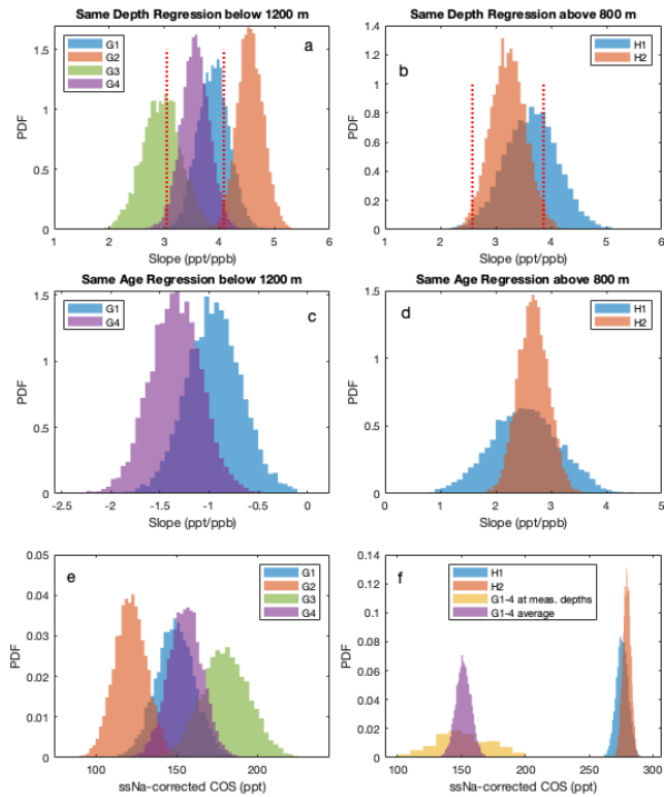
1085 Figure 3. a) PDFs of the same-depth errors-in-variables regressions for the glacial (below 1200 m) dry extraction COS 1090 measurements under four different analysis scenarios (section 3.1). b) Same as (a) for the two Holocene (above 800 m) scenarios. In (a) and (b), the \pm 2\sigma (95%) confidence intervals (red dashed lines) for the G4 and H2 regressions are shown to demonstrate the high statistical significance (being different from zero) of the PDFs for all scenarios. c-d) Same as (a) and (b) but for the same-age errors-in-variables linear regressions. e) Distributions of all dry COS measurements from 52–23 ky after correction with ssNa under G1 through G4 scenarios. f) Distributions of dry COS measurements after correction with ssNa under H1 (blue) and H2 (red) scenarios. For comparison, distributions of the average across G1 through G4 (purple, n=8000) and the average of all scenarios at discrete depths (yellow, n=177) are also shown. During the LGM, the ssNa-corrected wet COS measurements reach lower levels than what is displayed here for the 52–23 ky period (Fig. 4b).
