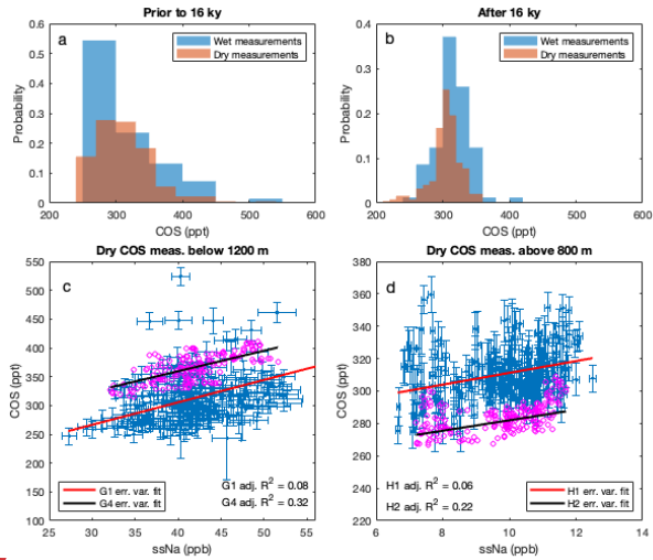
1075 Figure 2: a) Distribution of SPC14 COS measurements before 16 ky. The dry measurements shown here are the basis for the regressions shown in (c). b) Distribution of SPC14 COS measurements after 16 ky. The dry measurements shown here are the basis for the regressions shown in (d). c) The ssNa vs. dry COS measurements for the glacial period (below 1200 m) used in the G1 (blue error bars) and the G4 (magenta circles) scenarios (Table 2). The linear fits to errors-in-variables regressions are calculated using the mean slopes and intercepts for G1 and G4 (also see Figs. A5 and A6). d) Same as (c) but for the Holocene (above 800 m) H1 and H2 scenarios (also see Fig. A7).
